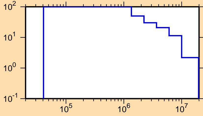
\Delta\sigma/\sigma vs. E for ^{204}\text{Fr}(n,n_1)
