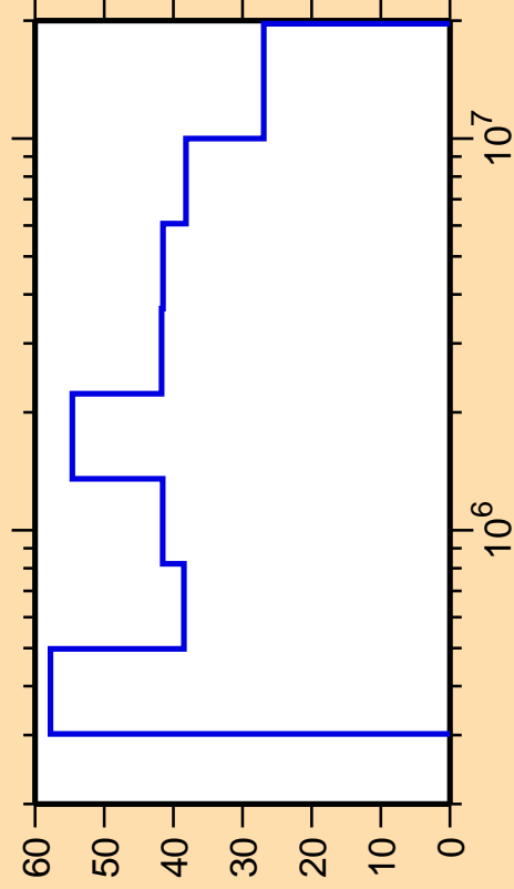
\Delta\sigma/\sigma vs. E for ^{204}\text{Fr}(n,n_4)
