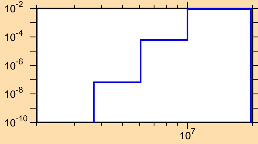
\sigma vs. E for ^{204}\text{Fr}(n,d)
