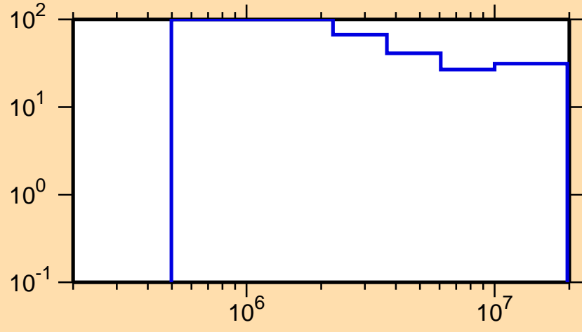
\Delta\sigma/\sigma vs. E for ^{204}\text{Fr}(n,ncont.)
