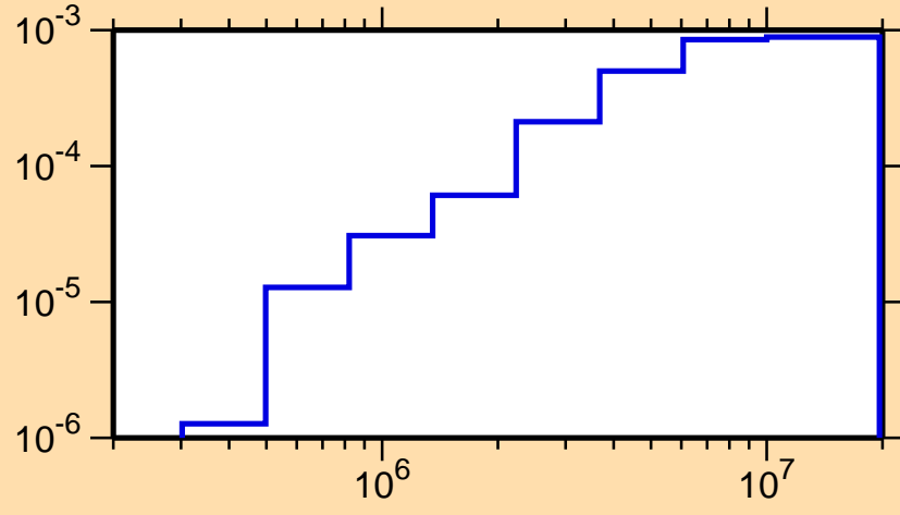
\sigma vs. E for ^{204}\text{Fr}(n,n_4)
