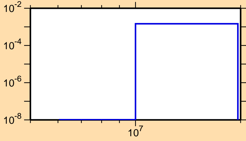
\sigma vs. E for ^{222}\text{Fr}(n,d)
