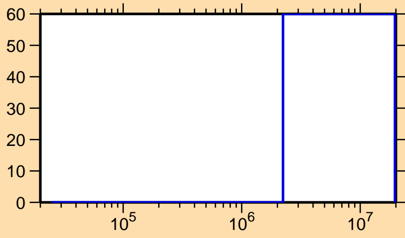
\Delta\sigma/\sigma vs. E for ^{222}\text{Fr}(n,f)
