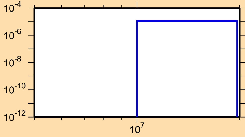
\sigma vs. E for ^{222}\text{Fr}(n,nd)
