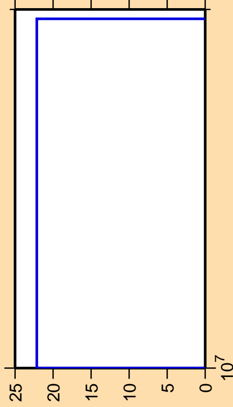
\Delta\sigma/\sigma vs. E for ^{222}\text{Fr} (mt 11)
