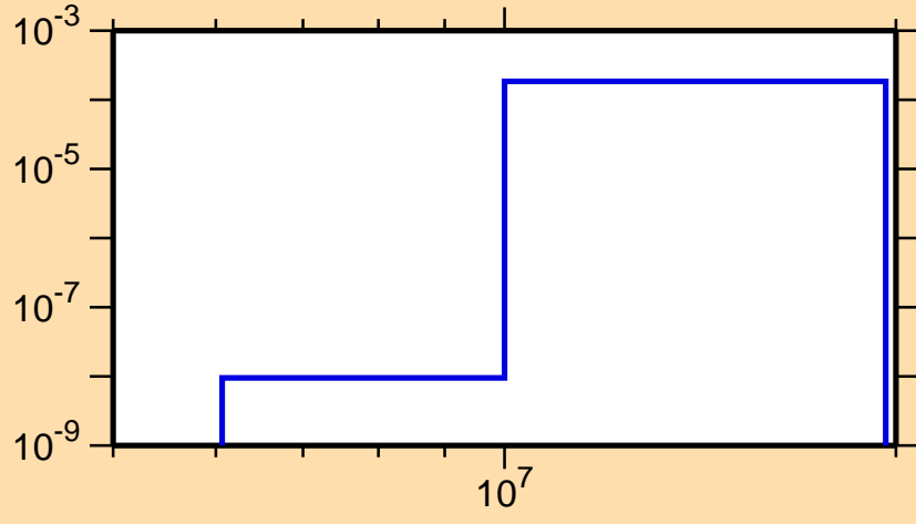
\sigma vs. E for ^{226}\text{Fr}(n,t)
