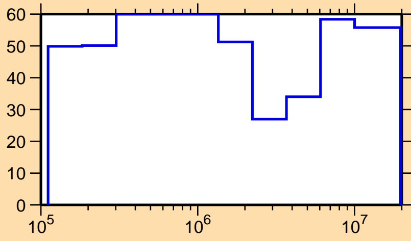
\Delta\sigma/\sigma vs. E for ^{226}\text{Fr}(n, \text{el.})
