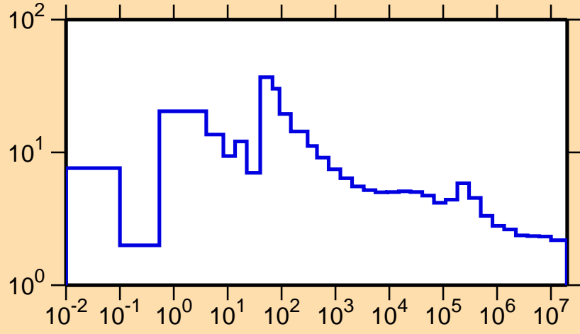
\sigma vs. E for ^{226}\text{Fr}(n,\text{nonel.})
