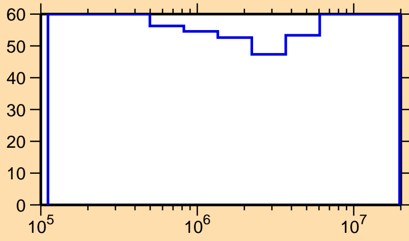
\Delta\sigma/\sigma vs. E for ^{228}\text{Fr}(n, ncont.)
