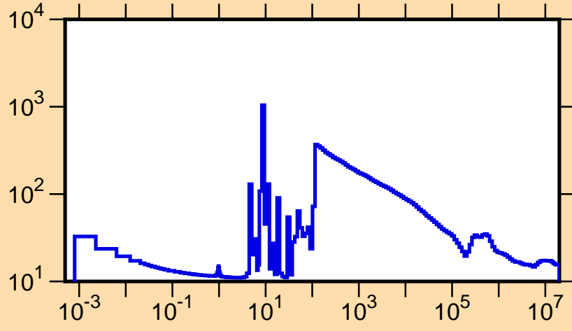
\sigma vs. E for ^{229}\text{Fr}(n,\text{tot.})
