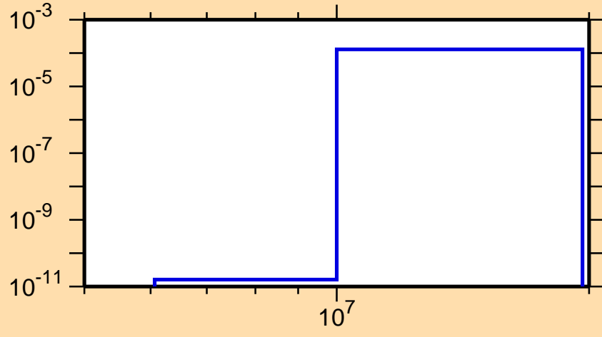
\sigma vs. E for ^{229}\text{Fr}(n,d)
