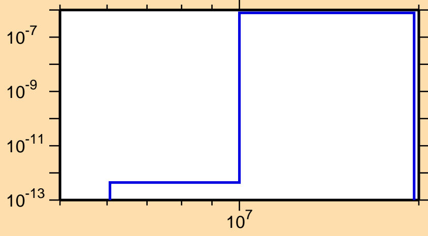
\sigma vs. E for ^{229}\text{Fr}(n,n\alpha)
