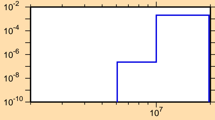
\sigma vs. E for ^{229}\text{Fr}(n,\alpha)
