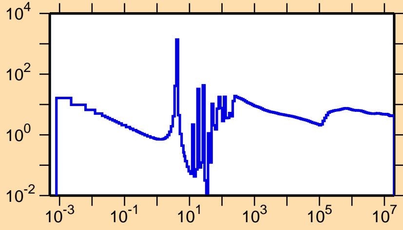
\sigma vs. E for ^{233}\text{Fr}(n,\text{nonel.})
