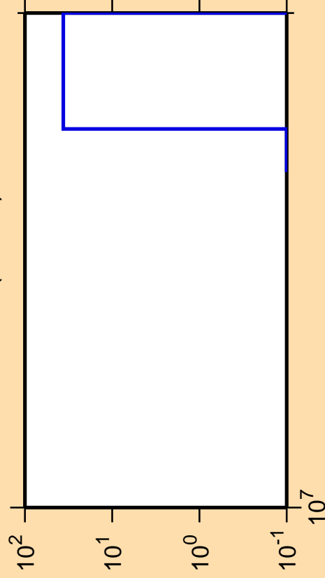
\Delta\sigma/\sigma vs. E for ^{233}\text{Fr}(n,3n\alpha)
