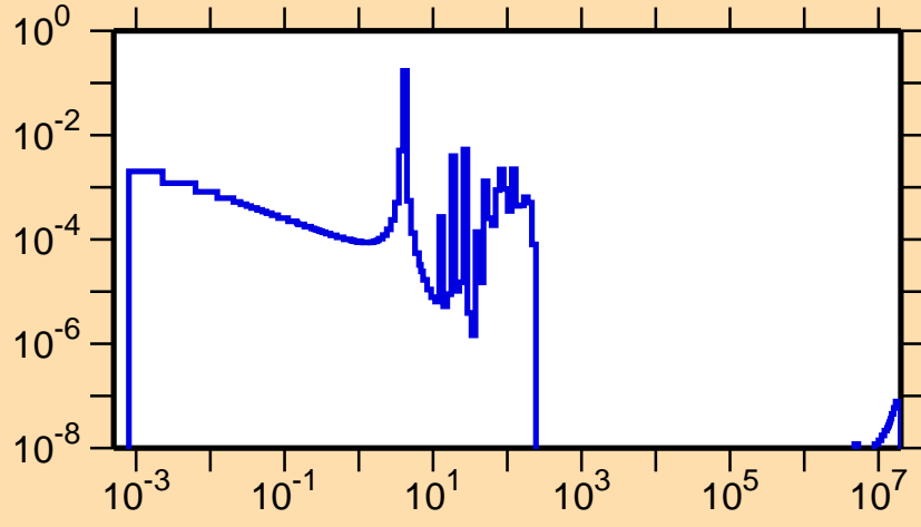
\sigma vs. E for ^{233}\text{Fr}(n,f)
