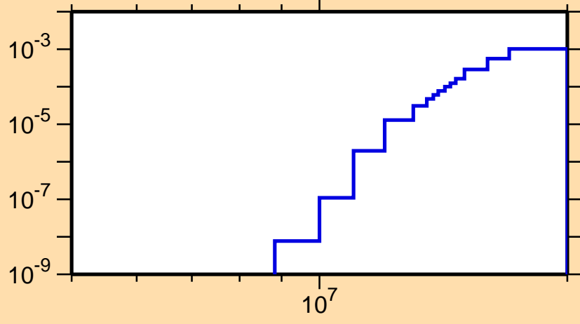
\sigma vs. E for ^{233}\text{Fr}(n,n\alpha)
