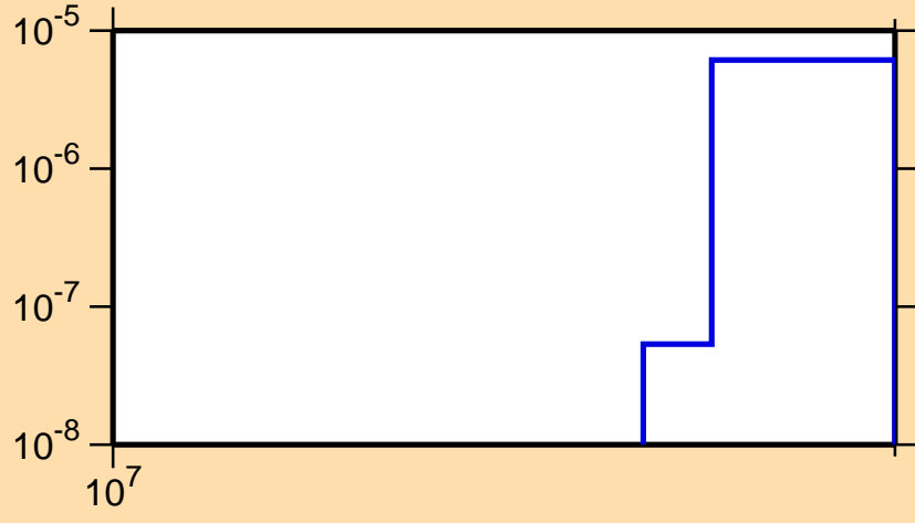
\sigma vs. E for ^{233}\text{Fr}(n,2np)
