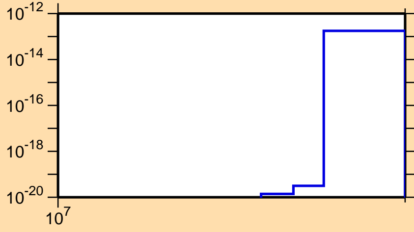
\sigma vs. E for ^{233}\text{Fr}(\text{mt } 11)
