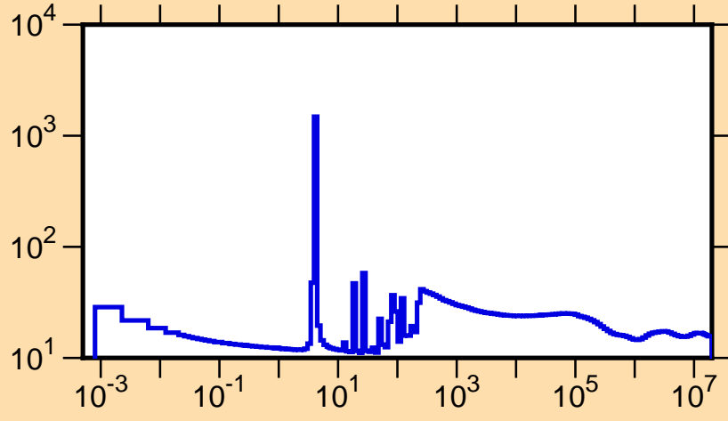
\sigma vs. E for ^{233}\text{Fr}(n,\text{tot.})
