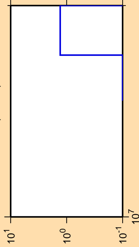
\Delta\sigma/\sigma vs. E for ^{233}\text{Fr}(\text{mt } 11)
