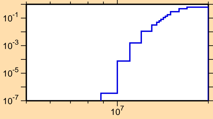
\sigma vs. E for ^{233}\text{Fr}(n,3n)
