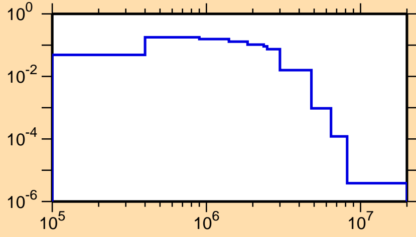
\sigma vs. E for ^{76}\text{Ga}(n,n_2)
