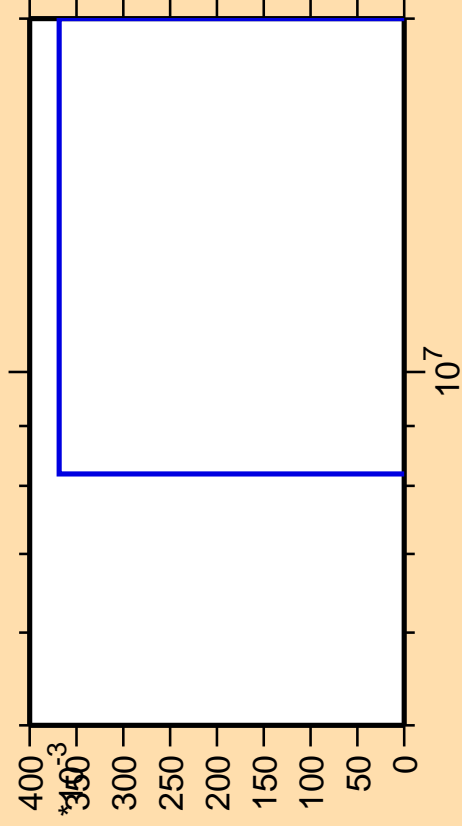
\Delta\sigma/\sigma vs. E for ^{76}\text{Ga}(n,2n\alpha)
