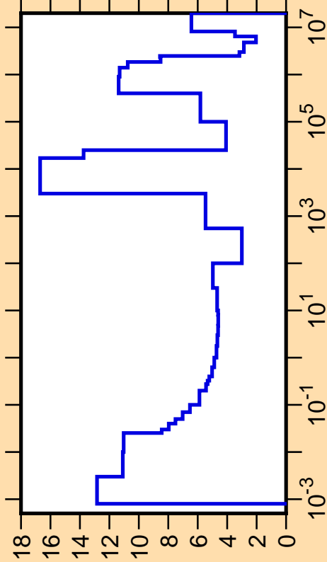
\Delta\sigma/\sigma vs. E for ^{76}\text{Ga}(n,\text{tot.})
