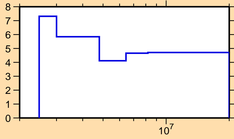
\Delta\sigma/\sigma vs. E for ^{76}\text{Ga}(n,n\text{onel.})
