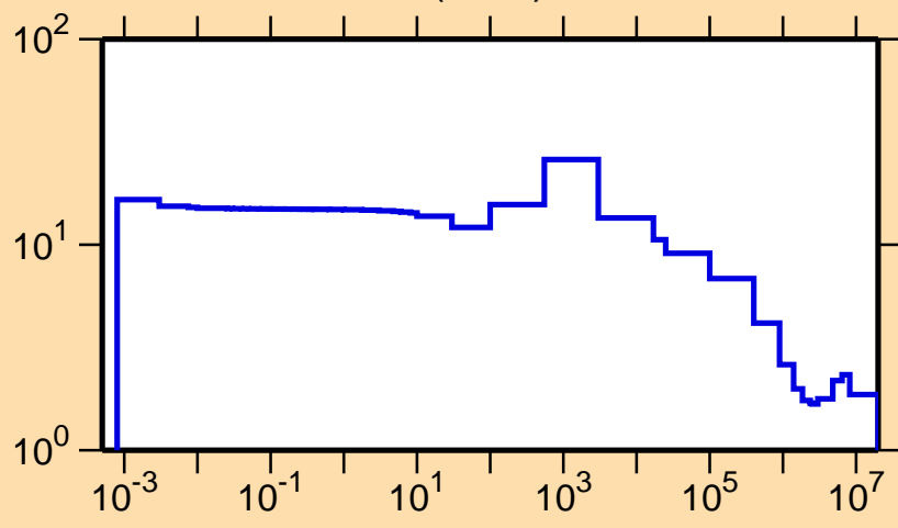
\sigma vs. E for ^{76}\text{Ga}(n,\text{el.})
