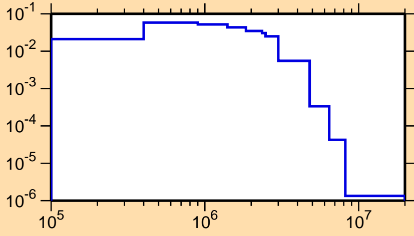
\sigma vs. E for ^{76}\text{Ga}(n,n_1)
