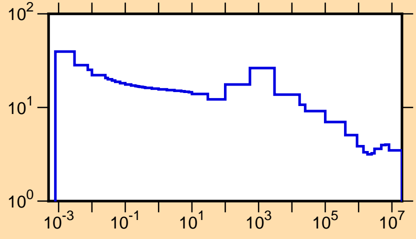
\sigma vs. E for ^{76}\text{Ga}(n,\text{tot.})
