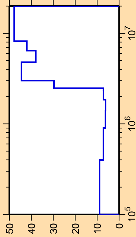
\Delta\sigma/\sigma vs. E for ^{76}\text{Ga}(n,n_3)
