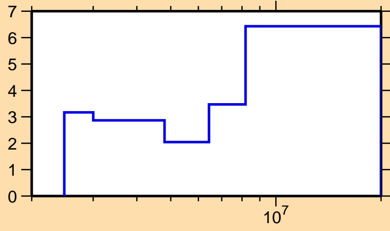
\Delta\sigma/\sigma vs. E for ^{76}\text{Ga}(n,\text{tot.})
