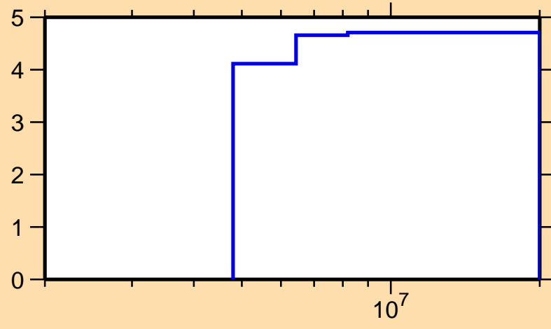
\Delta\sigma/\sigma vs. E for ^{76}\text{Ga}(n,\text{nonel.})
