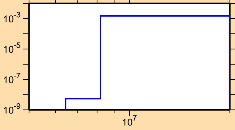
\sigma vs. E for ^{77}\text{Ga}(n,p)
