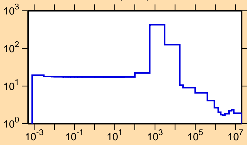
\sigma vs. E for ^{77}\text{Ga}(n,\text{el.})
