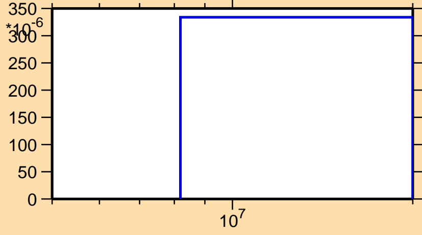
\sigma vs. E for ^{77}\text{Ga}(n,d)
