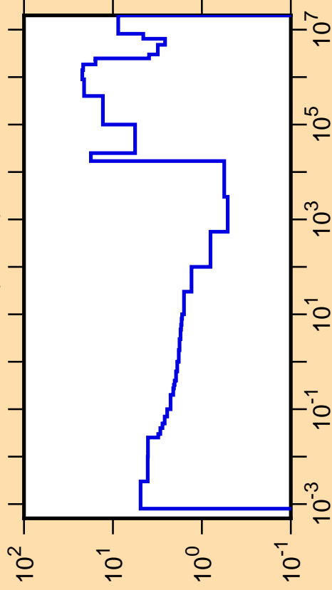
\Delta\sigma/\sigma vs. E for ^{77}\text{Ga}(n,\text{tot.})
