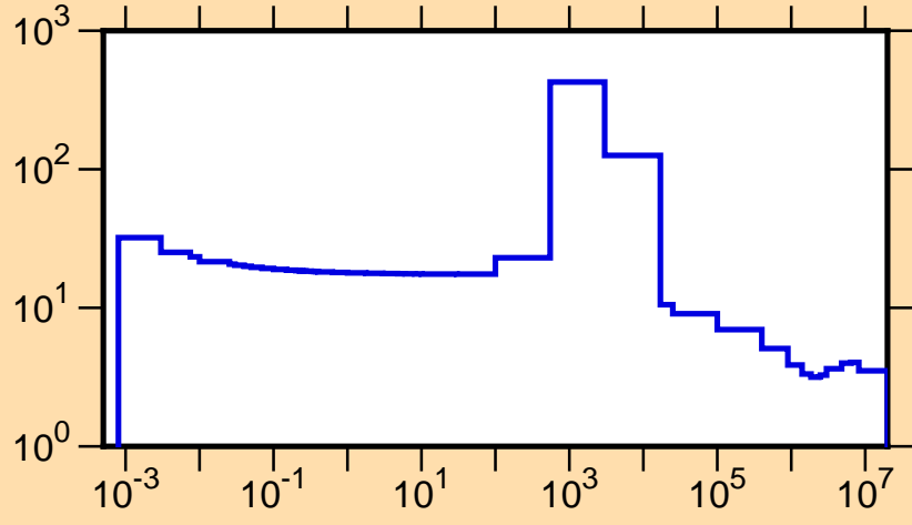
\sigma vs. E for ^{77}\text{Ga}(n,\text{tot.})
