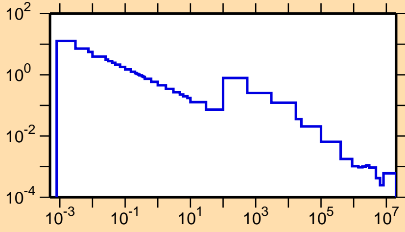
\sigma vs. E for ^{77}\text{Ga}(n,\gamma)
