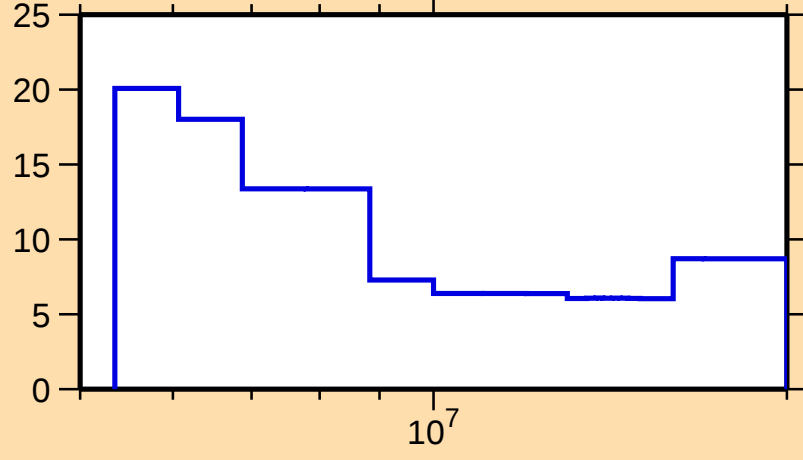
\Delta\sigma/\sigma vs. E for ^{158}\text{Hf}(n,\text{tot.})
