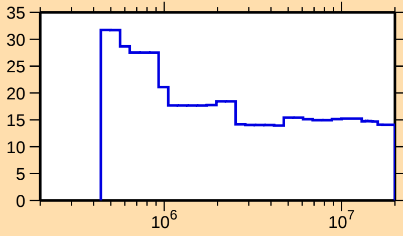
\Delta\sigma/\sigma vs. E for ^{158}\text{Hf}(n,\text{nonel.})
