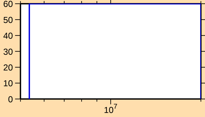
\Delta\sigma/\sigma vs. E for ^{158}\text{Hf}(n,n_1)
