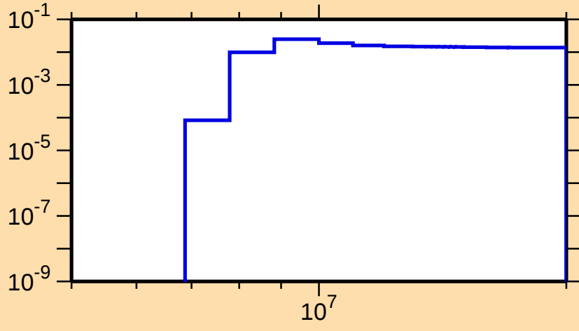
\sigma vs. E for ^{158}\text{Hf}(n,n\text{cont.})
