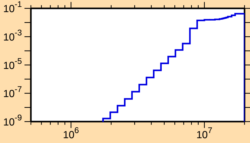
\sigma vs. E for ^{158}\text{Hf}(n,n\alpha)
