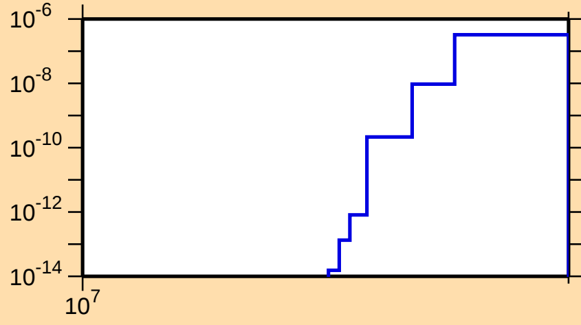
\sigma vs. E for ^{158}\text{Hf}(n,\text{nd})
