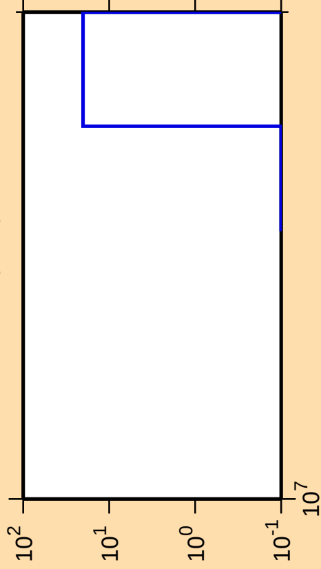
\Delta\sigma/\sigma vs. E for ^{158}\text{Hf}(n,nt)
