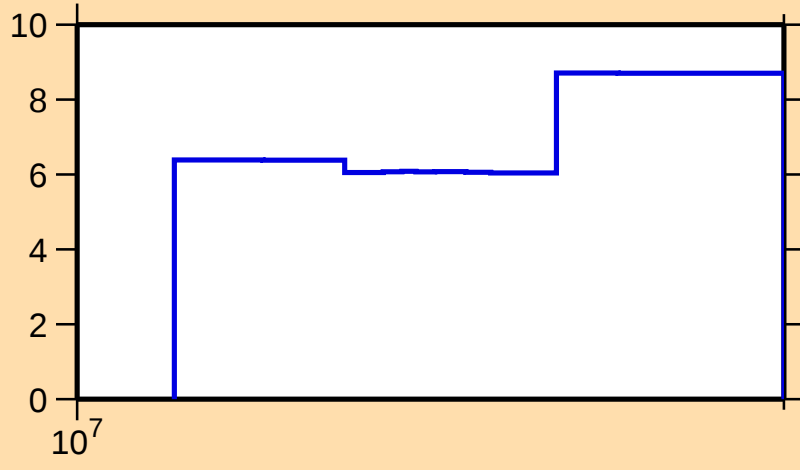
\Delta\sigma/\sigma vs. E for ^{158}\text{Hf}(n,\text{tot.})
