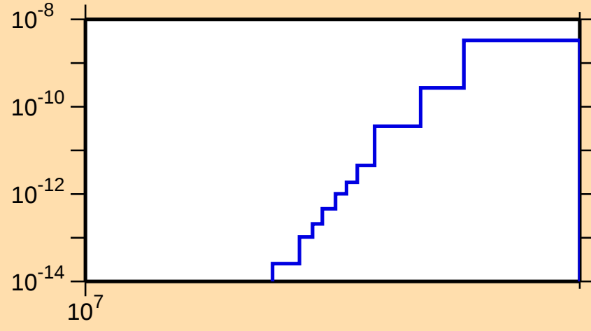
\sigma vs. E for ^{158}\text{Hf}(\text{mt } 34)
