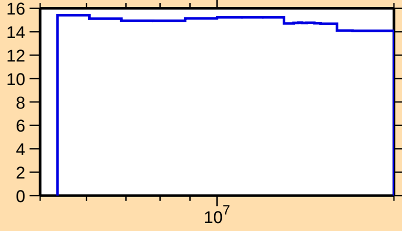
\Delta\sigma/\sigma vs. E for ^{158}\text{Hf}(n,\text{nonel.})
