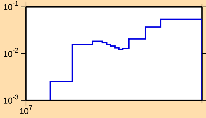
\sigma vs. E for ^{158}\text{Hf}(n,2n)
