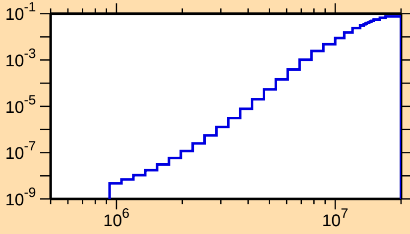
\sigma vs. E for ^{158}\text{Hf}(n,p\alpha)
