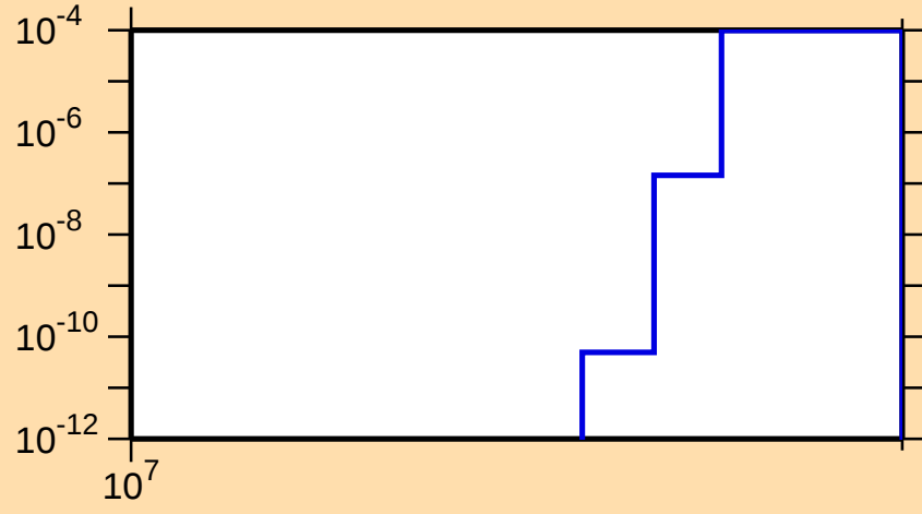
\sigma vs. E for ^{158}\text{Hf}(n,2np)
