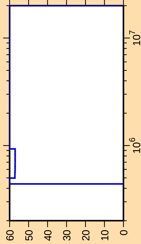
\Delta\sigma/\sigma vs. E for ^{158}\text{Hf}(n,n_1)
