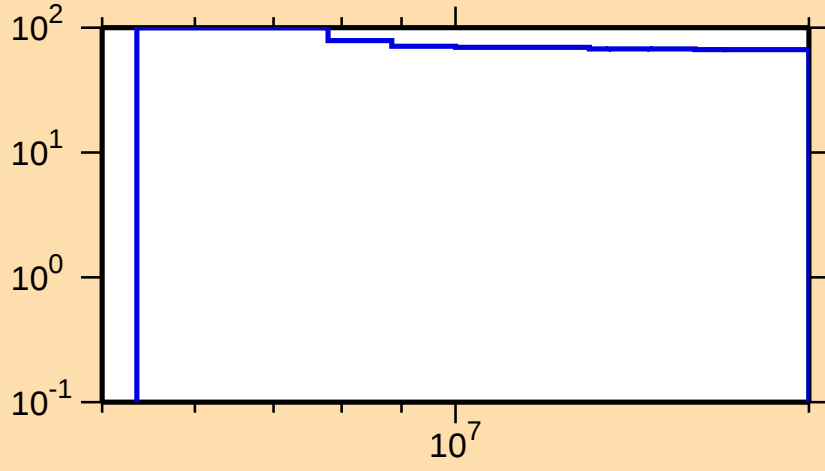
\Delta\sigma/\sigma vs. E for ^{158}\text{Hf}(n,n\text{cont.})
