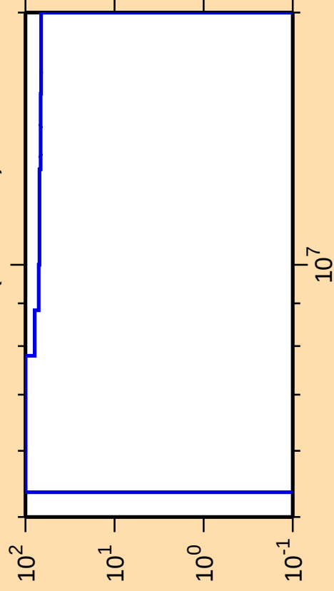
\Delta\sigma/\sigma vs. E for ^{158}\text{Hf}(n,\text{ncont.})
