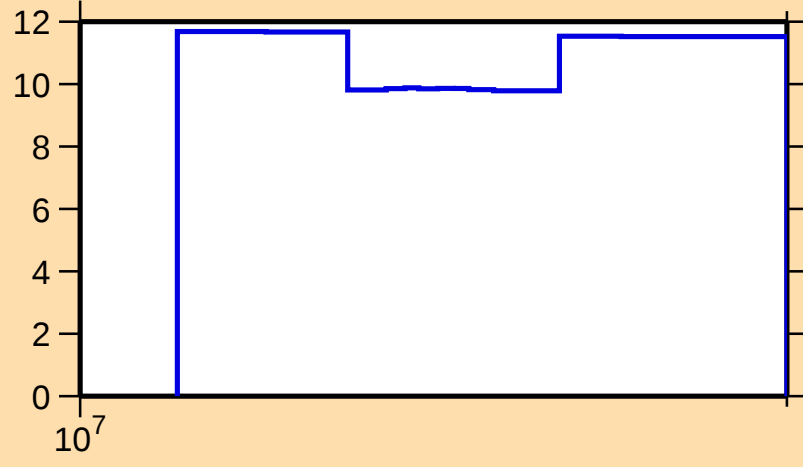
\Delta\sigma/\sigma vs. E for ^{158}\text{Hf}(n,\text{el.})
