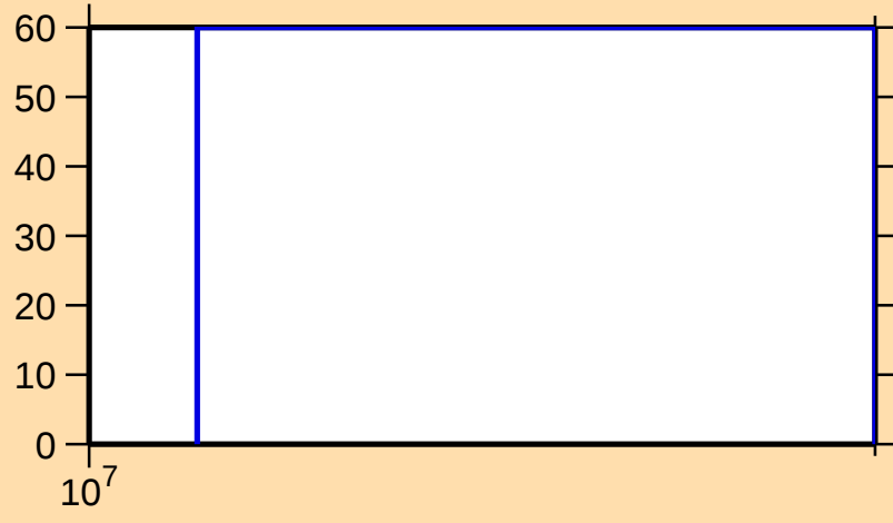
\Delta\sigma/\sigma vs. E for ^{158}\text{Hf}(n,2n)
