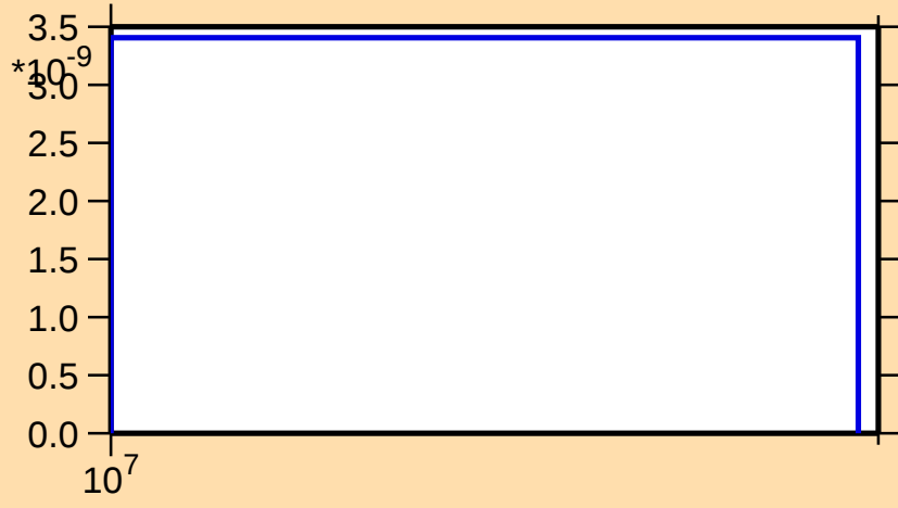
\sigma vs. E for ^{158}\text{Hf}(n,\text{nd})
