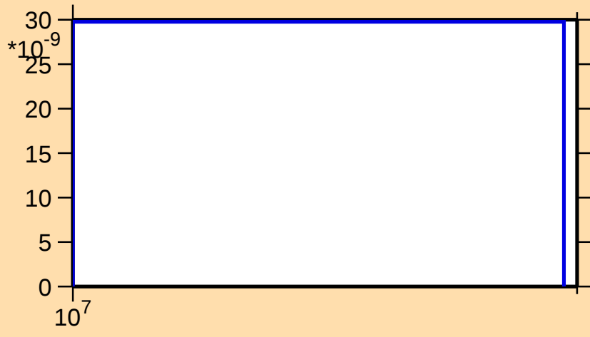
\sigma vs. E for ^{158}\text{Hf}(n,\text{pt})
