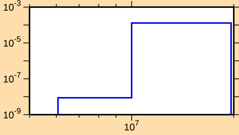
\sigma vs. E for ^{158}\text{Hf}(\text{mt } 45)
