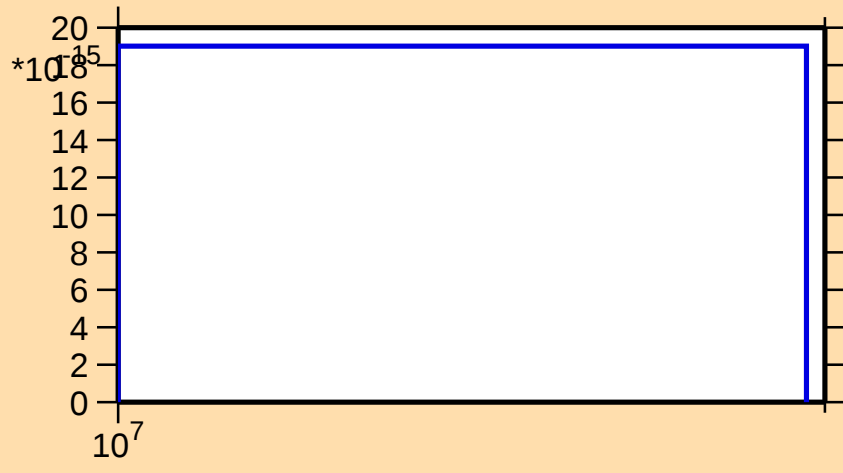
\sigma vs. E for ^{158}\text{Hf}(n,nt)
