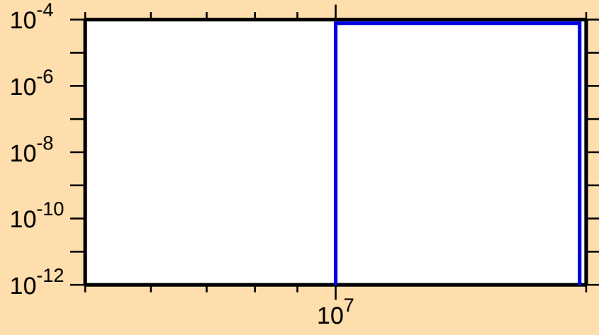
\sigma vs. E for ^{158}\text{Hf}(n,2n\alpha)
