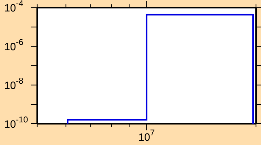
\sigma vs. E for ^{158}\text{Hf}(n,\text{pd})
