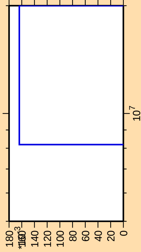
\Delta\sigma/\sigma vs. E for ^{158}\text{Hf}(n,nt)
