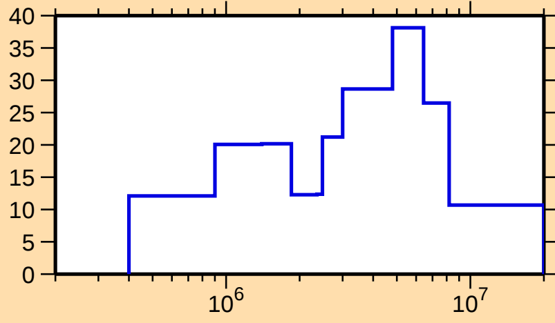
\Delta\sigma/\sigma vs. E for ^{158}\text{Hf}(n,\text{el.})
