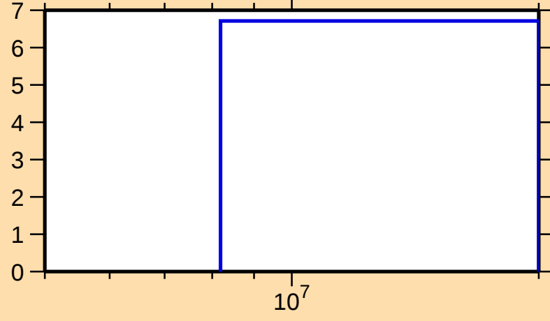
\Delta\sigma/\sigma vs. E for ^{158}\text{Hf}(n,\text{tot.})
