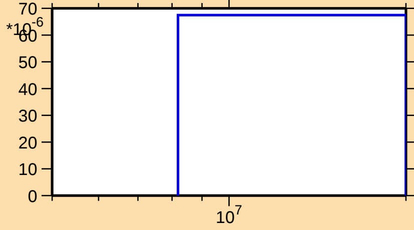
\sigma vs. E for ^{158}\text{Hf}(n,t)
