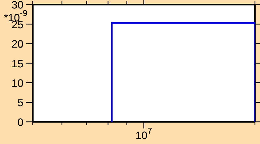
\sigma vs. E for ^{158}\text{Hf}(n,pt)
