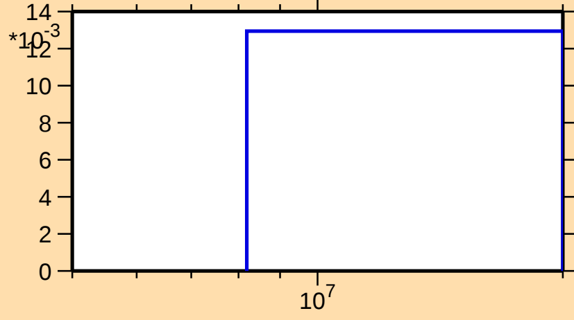
\sigma vs. E for ^{158}\text{Hf}(n,2n)
