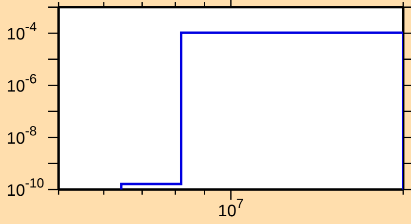
\sigma vs. E for ^{158}\text{Hf}(\text{mt } 45)
