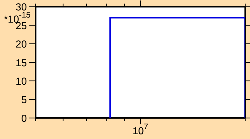
\sigma vs. E for ^{158}\text{Hf}(n,nt)
