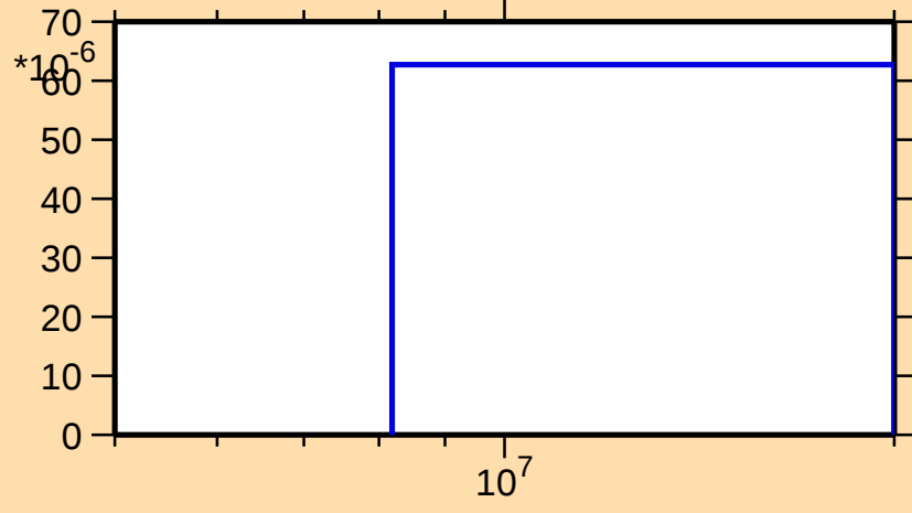
\sigma vs. E for ^{158}\text{Hf}(n,2n\alpha)
