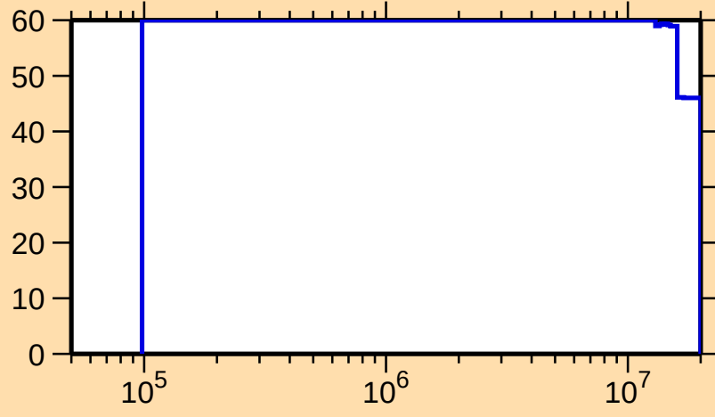
\Delta\sigma/\sigma vs. E for ^{159}\text{Hf}(n,\text{inel.})
