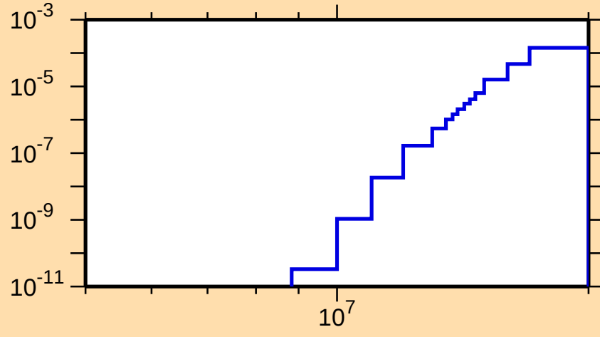
\sigma vs. E for ^{159}\text{Hf}(n,\text{pd})
