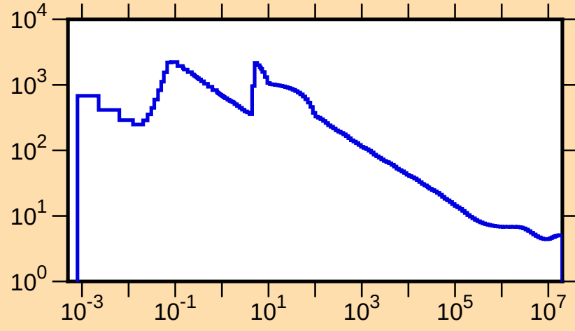
\sigma vs. E for ^{159}\text{Hf}(n,\text{tot.})
