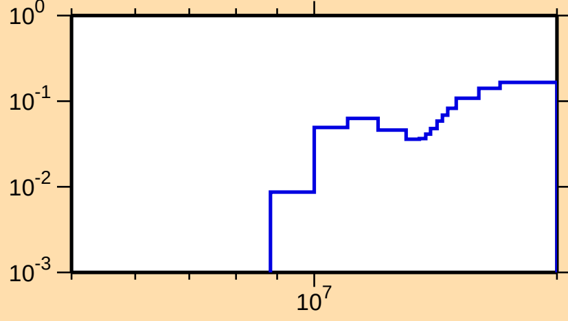
\sigma vs. E for ^{159}\text{Hf}(n,2n)
