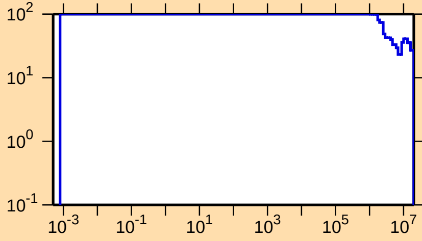
\Delta\sigma/\sigma vs. E for ^{159}\text{Hf}(n,p)
