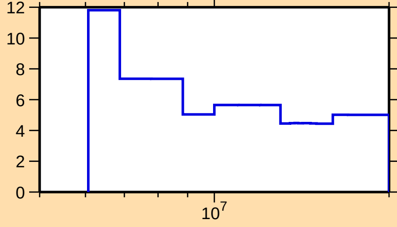
\Delta\sigma/\sigma vs. E for ^{159}\text{Hf}(n,\text{tot.})
