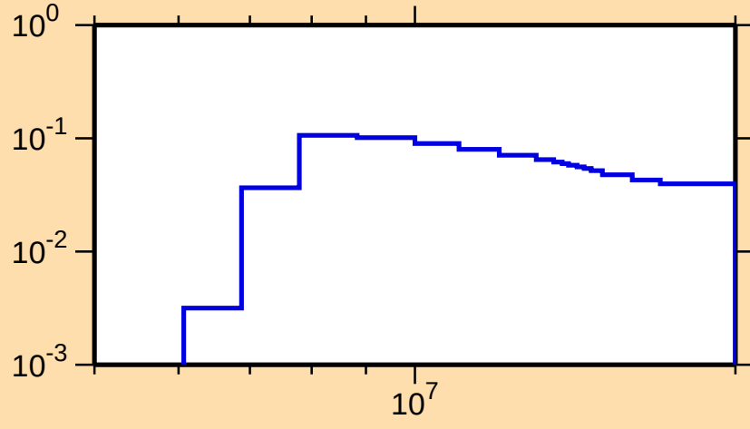
\sigma vs. E for ^{159}\text{Hf}(n,n\text{cont.})
