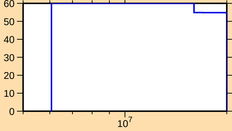
\Delta\sigma/\sigma vs. E for ^{159}\text{Hf}(n,\text{ncont.})
