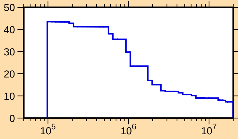
\Delta\sigma/\sigma vs. E for ^{159}\text{Hf}(n,\text{nonel.})
