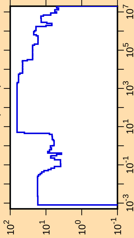
\Delta\sigma/\sigma vs. E for ^{159}\text{Hf}(n,\text{tot.})
