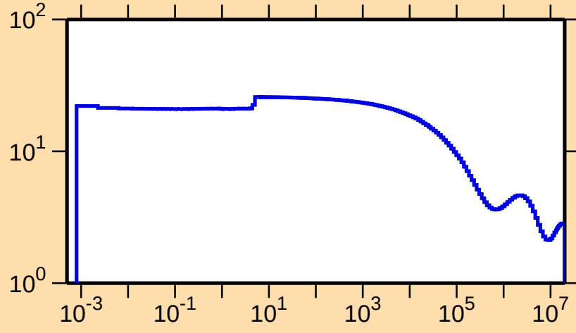
\sigma vs. E for ^{159}\text{Hf}(n,\text{el.})
