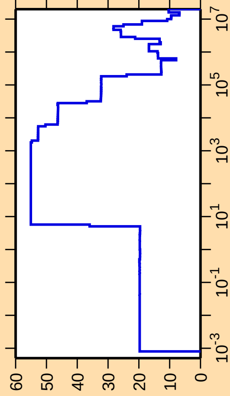
\Delta\sigma/\sigma vs. E for ^{161}\text{Hf}(n,\text{el.})
