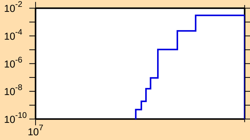
\sigma vs. E for ^{161}\text{Hf}(n,2np)
