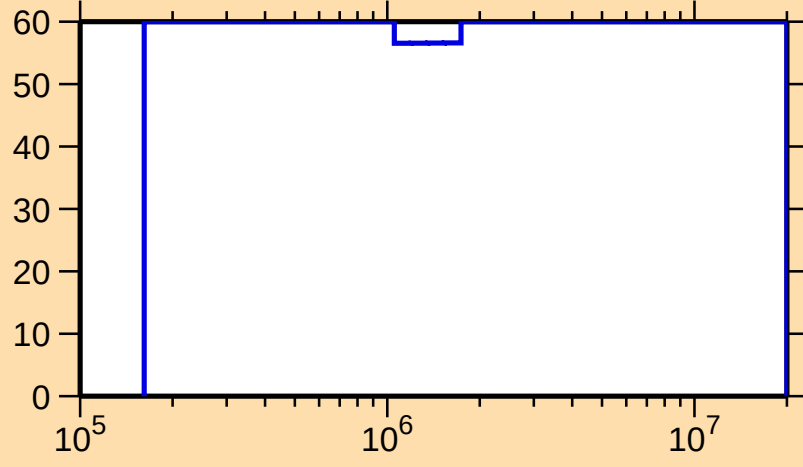
\Delta\sigma/\sigma vs. E for ^{161}\text{Hf}(n,n_1)
