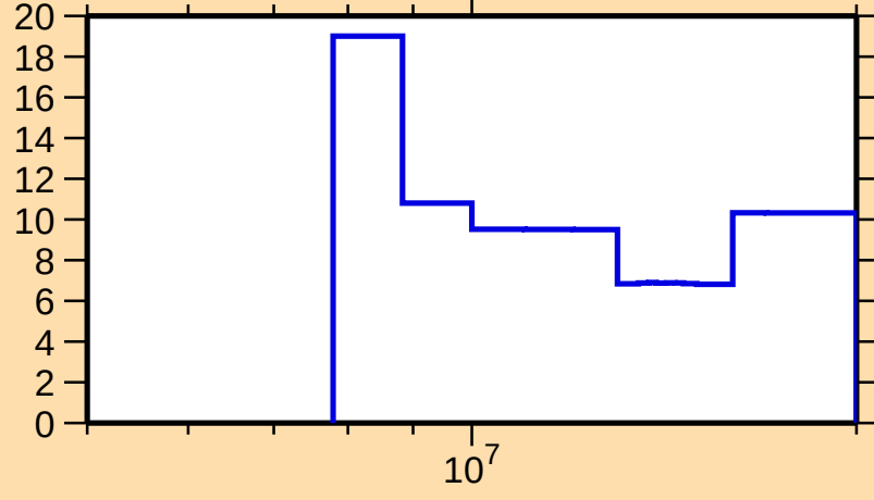
\Delta\sigma/\sigma vs. E for ^{161}\text{Hf}(n,\text{el.})
