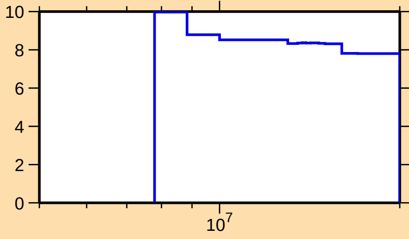
\Delta\sigma/\sigma vs. E for ^{161}\text{Hf}(n,\text{nonel.})
