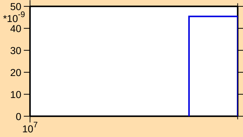
\sigma vs. E for ^{161}\text{Hf}(n,3n)
