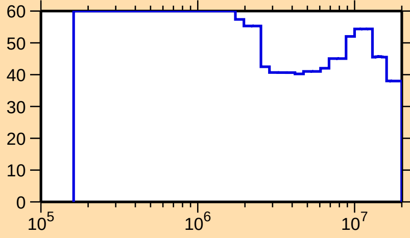
\Delta\sigma/\sigma vs. E for ^{161}\text{Hf}(n,n\text{cont.})
