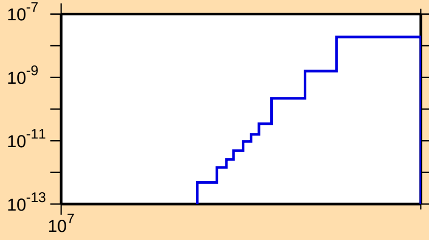
\sigma vs. E for ^{161}\text{Hf}(\text{mt } 34)
