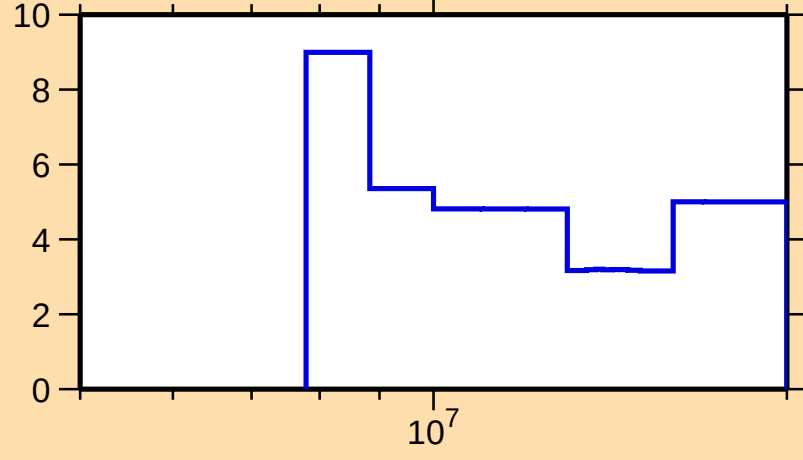
\Delta\sigma/\sigma vs. E for ^{161}\text{Hf}(n,\text{tot.})
