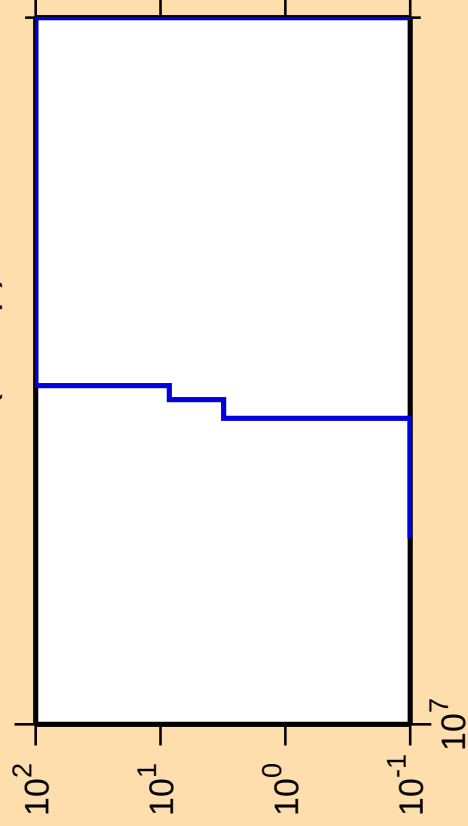
\Delta\sigma/\sigma vs. E for ^{161}\text{Hf}(n,2np)
