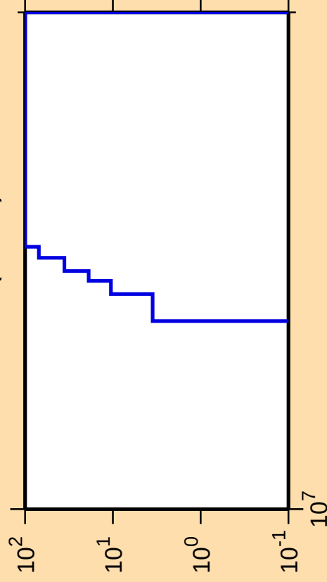
\Delta\sigma/\sigma vs. E for ^{161}\text{Hf}(\text{mt } 34)
