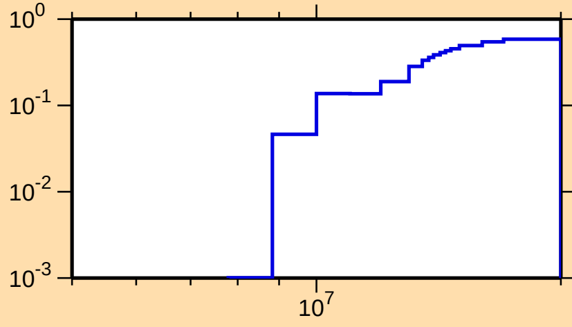
\sigma vs. E for ^{161}\text{Hf}(n,2n)
