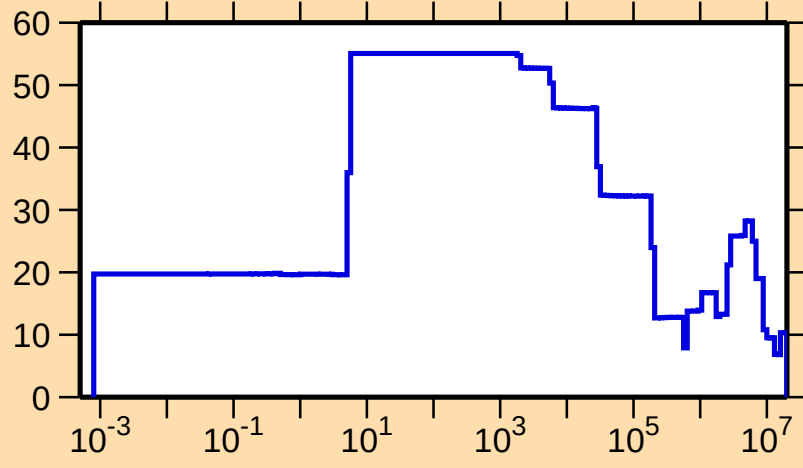
\Delta\sigma/\sigma vs. E for ^{161}\text{Hf}(n,\text{el.})
