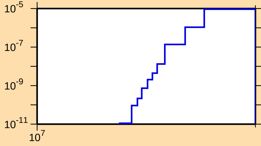
\sigma vs. E for ^{161}\text{Hf}(n,\text{nd})
