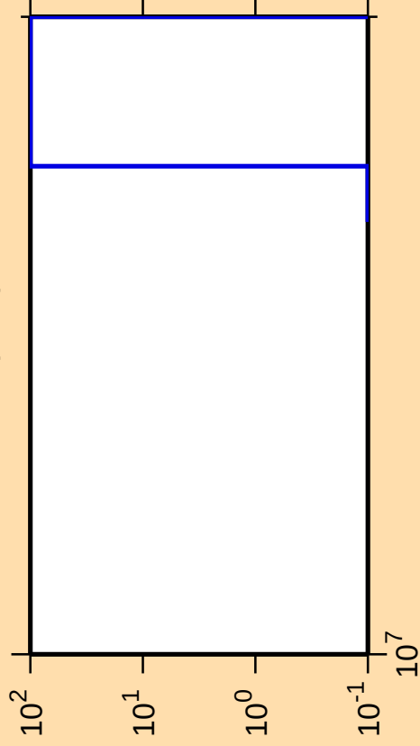
\Delta\sigma/\sigma vs. E for ^{161}\text{Hf}(n,nt)
