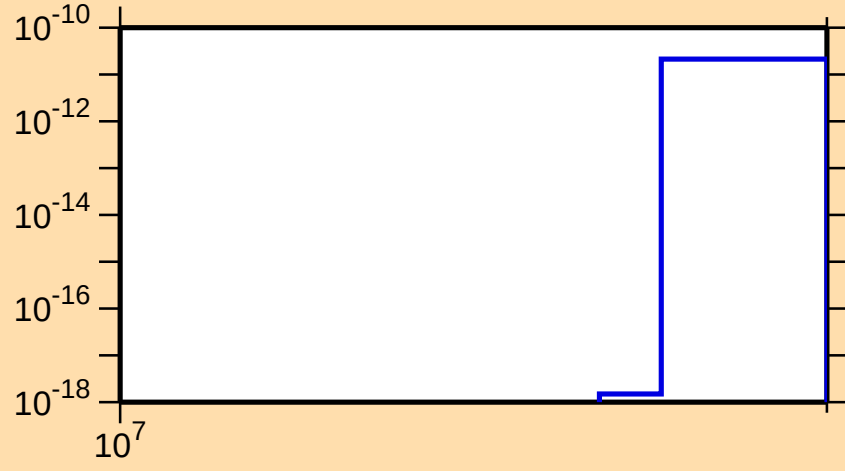
\sigma vs. E for ^{161}\text{Hf}(n,nt)
