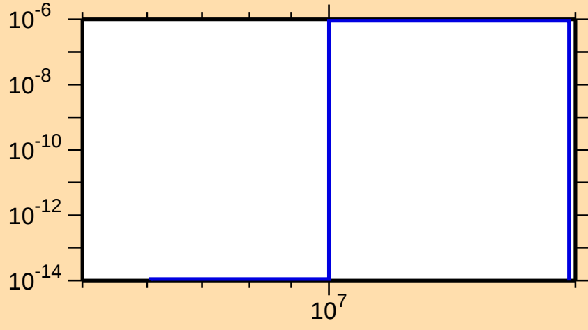
\sigma vs. E for ^{161}\text{Hf}(n,\text{pd})
