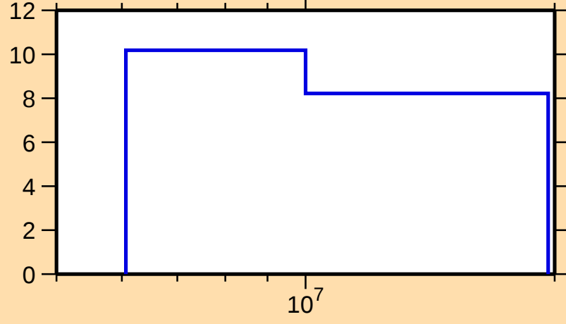
\Delta\sigma/\sigma vs. E for ^{161}\text{Hf}(n,\text{nonel.})
