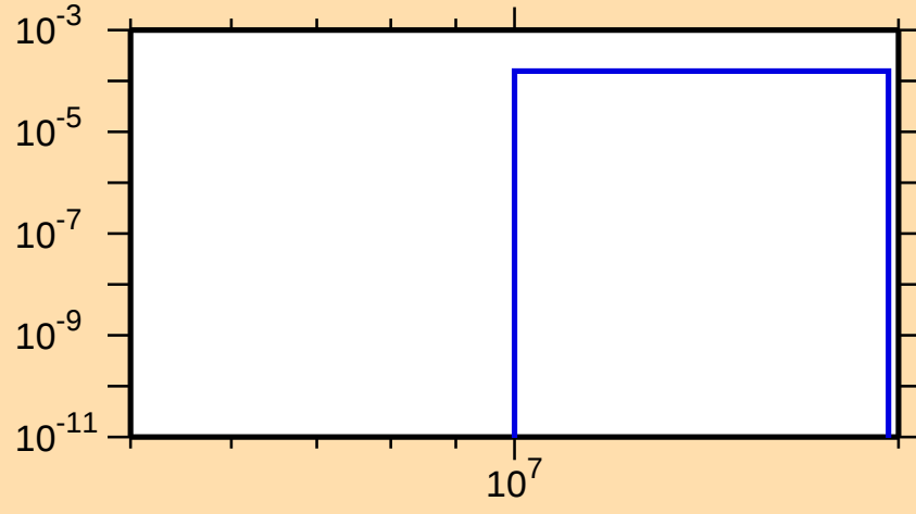
\sigma vs. E for ^{161}\text{Hf}(n,2n\alpha)
