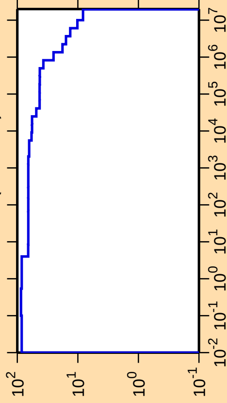
\Delta\sigma/\sigma vs. E for ^{161}\text{Hf}(n,\text{nonel.})
