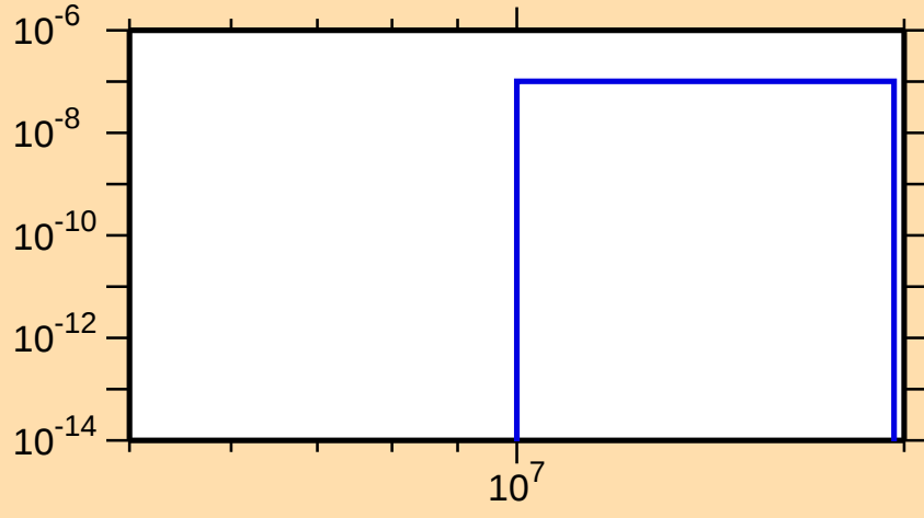
\sigma vs. E for ^{161}\text{Hf}(n,\text{pt})
