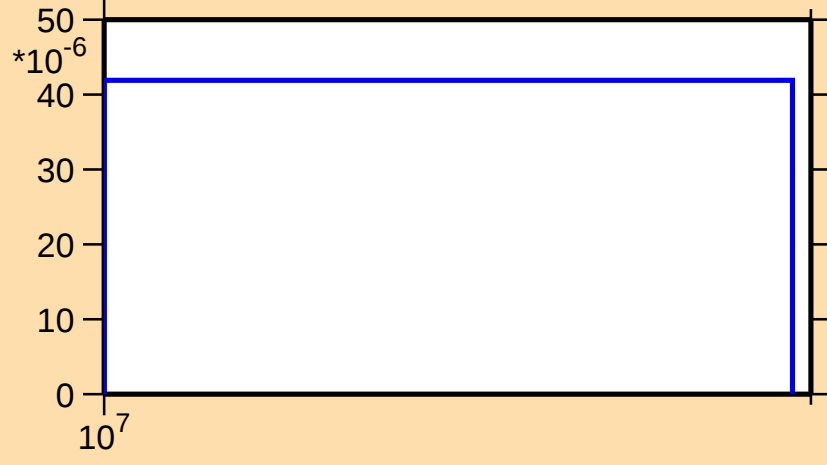
\sigma vs. E for ^{161}\text{Hf}(n,2np)
