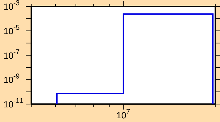
\sigma vs. E for ^{161}\text{Hf}(n,t)
