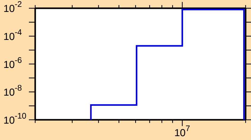
\sigma vs. E for ^{161}\text{Hf}(n,d)
