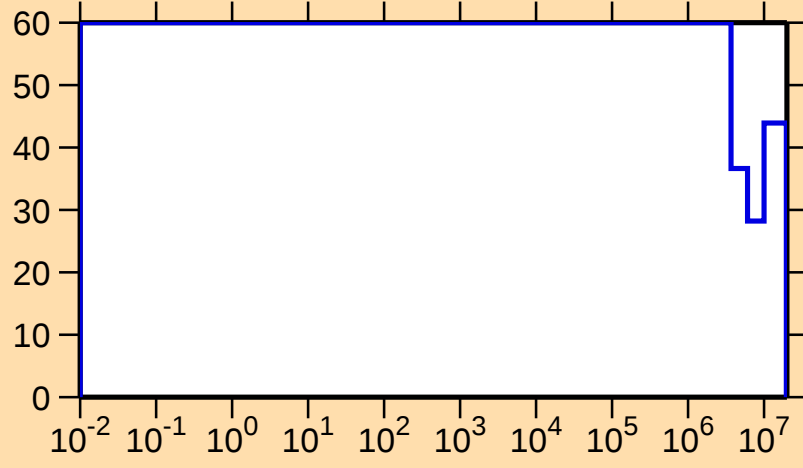
\Delta\sigma/\sigma vs. E for ^{161}\text{Hf}(n,p)
