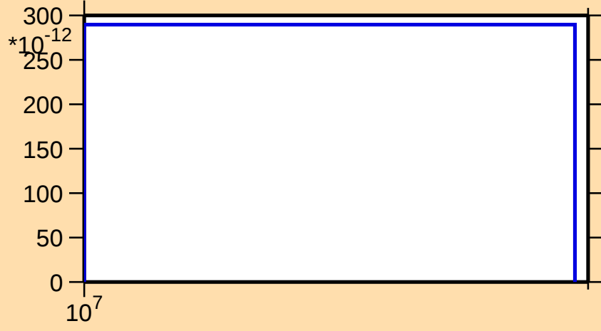
\sigma vs. E for ^{161}\text{Hf} (mt 34)
