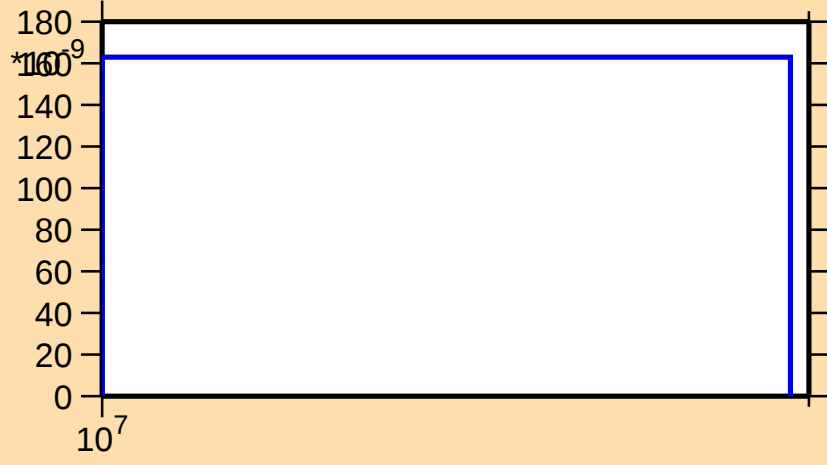
\sigma vs. E for ^{161}\text{Hf}(n,\text{nd})
