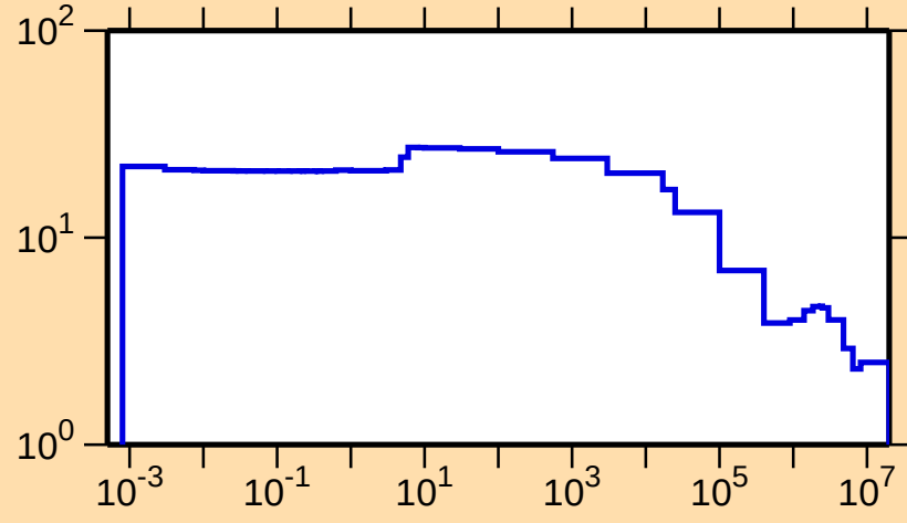
\sigma vs. E for ^{161}\text{Hf}(n,\text{el.})
