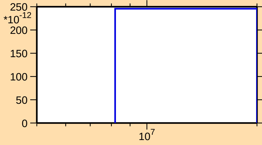
\sigma vs. E for ^{161}\text{Hf}(\text{mt } 34)
