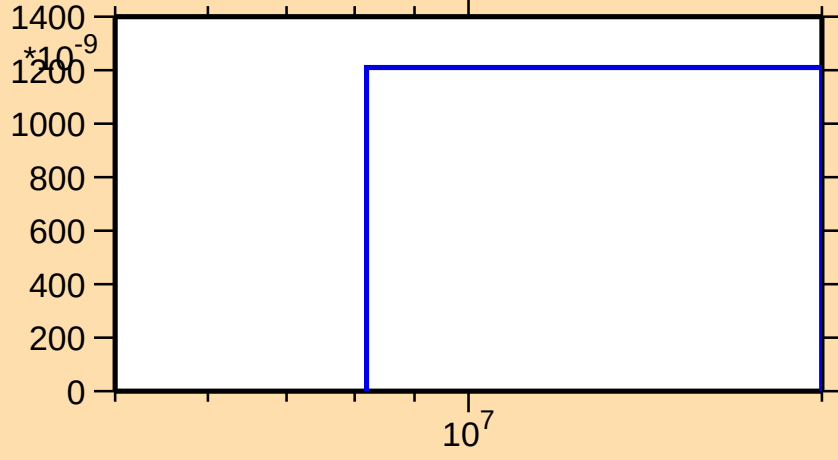
\sigma vs. E for ^{161}\text{Hf}(\text{mt } 45)
