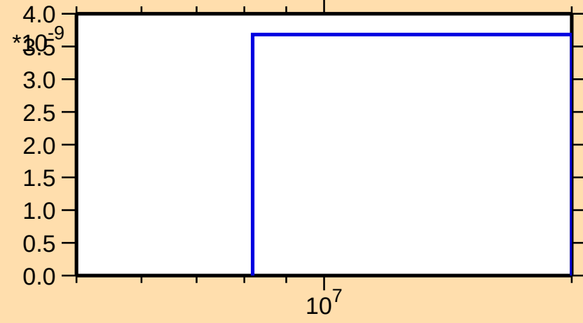
\sigma vs. E for ^{161}\text{Hf}(\text{mt117})
