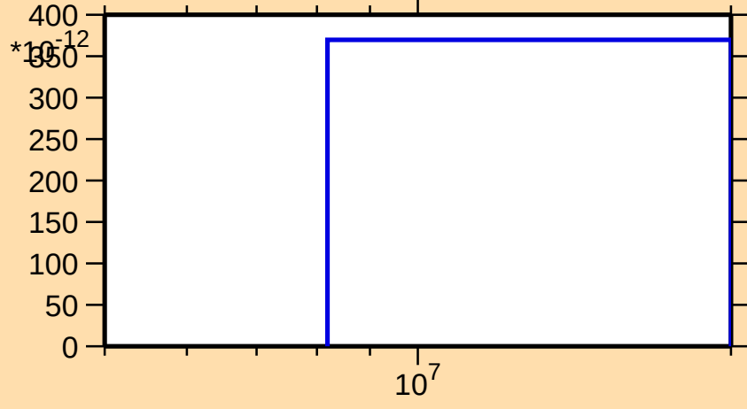
\sigma vs. E for ^{161}\text{Hf}(n,3n)
