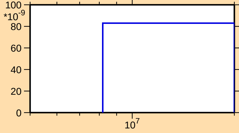
\sigma vs. E for ^{161}\text{Hf}(n,\text{pt})
