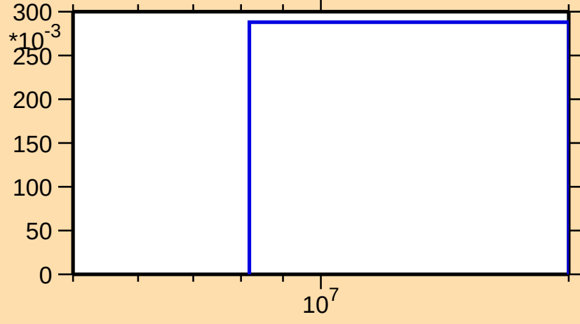
\sigma vs. E for ^{161}\text{Hf}(n,2n)
