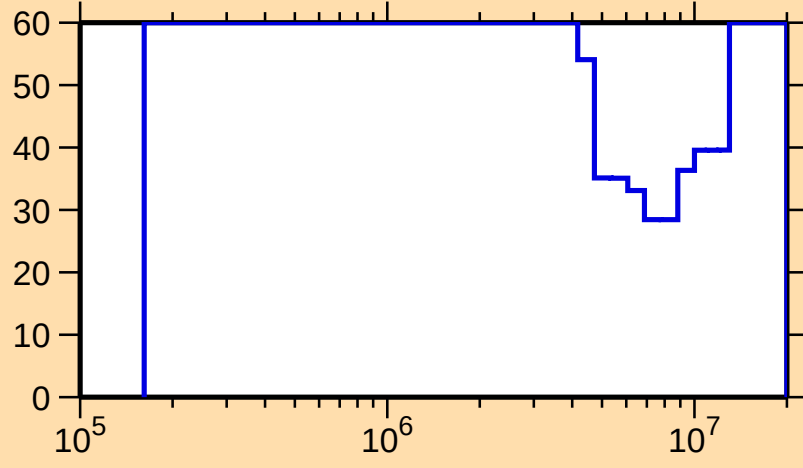
\Delta\sigma/\sigma vs. E for ^{163}\text{Hf}(n,\text{inel.})
