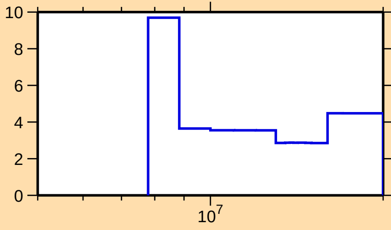
\Delta\sigma/\sigma vs. E for ^{163}\text{Hf}(n,\text{tot.})
