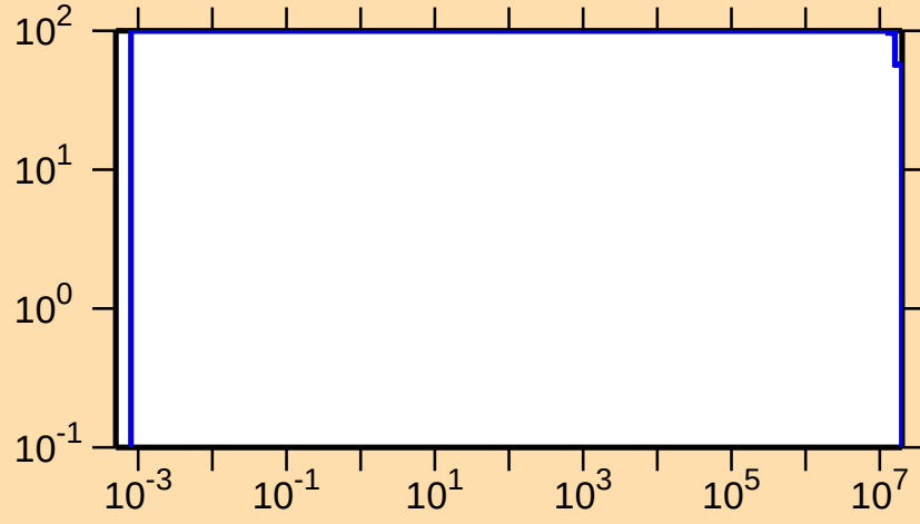
\Delta\sigma/\sigma vs. E for ^{163}\text{Hf}(n,p)
