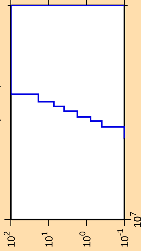
\Delta\sigma/\sigma vs. E for ^{163}\text{Hf}(\text{mt } 34)
