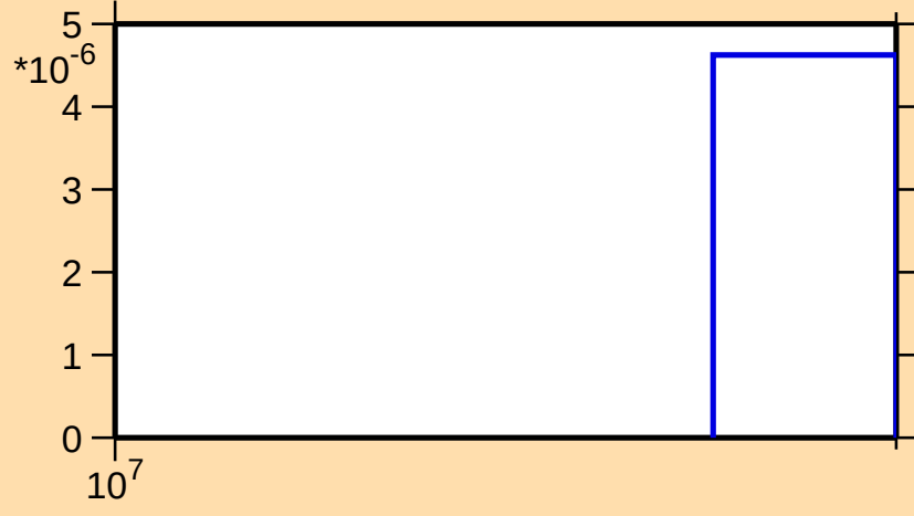
\sigma vs. E for ^{163}\text{Hf}(n,3n)
