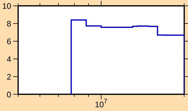
\Delta\sigma/\sigma vs. E for ^{163}\text{Hf}(n,\text{nonel.})
