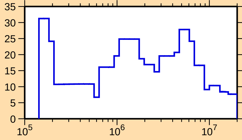
\Delta\sigma/\sigma vs. E for ^{163}\text{Hf}(n,\text{el.})
