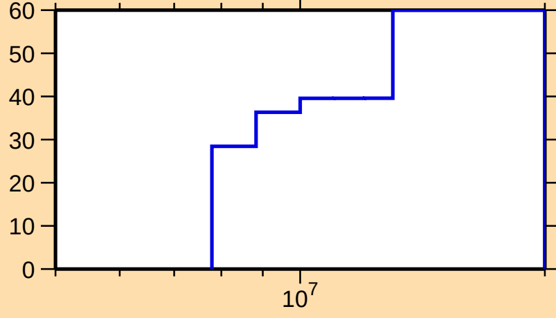
\Delta\sigma/\sigma vs. E for ^{163}\text{Hf}(n,\text{inel.})
