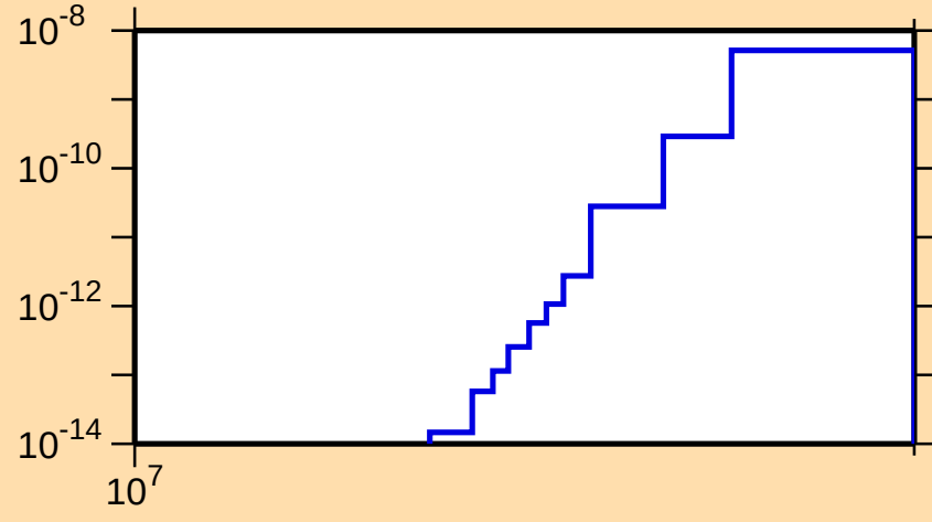
\sigma vs. E for ^{163}\text{Hf}(\text{mt } 34)
