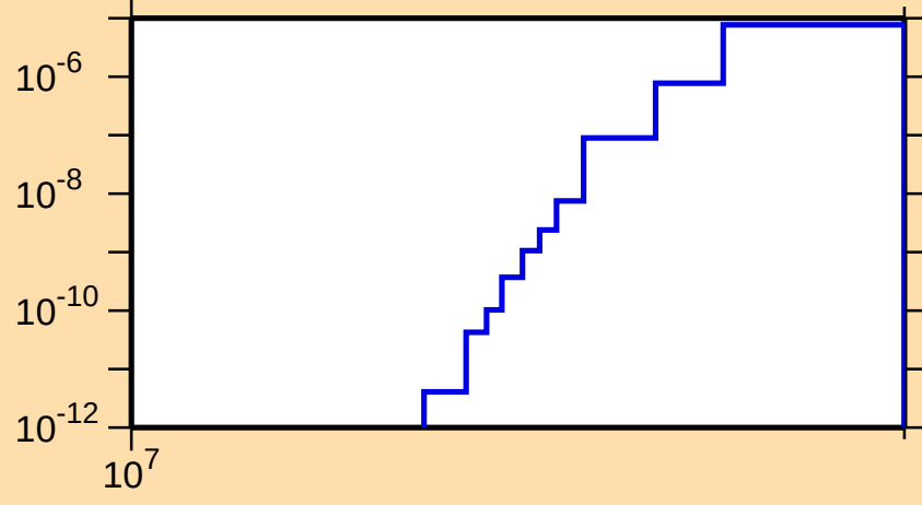
\sigma vs. E for ^{163}\text{Hf}(n,\text{nd})
