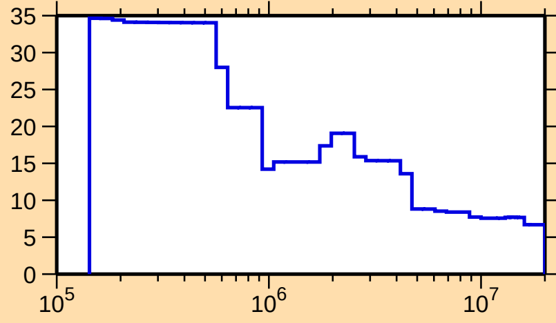
\Delta\sigma/\sigma vs. E for ^{163}\text{Hf}(n,\text{nonel.})
