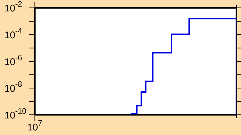
\sigma vs. E for ^{163}\text{Hf}(n,2np)
