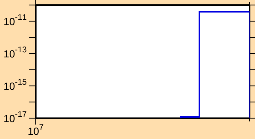
\sigma vs. E for ^{163}\text{Hf}(n,nt)
