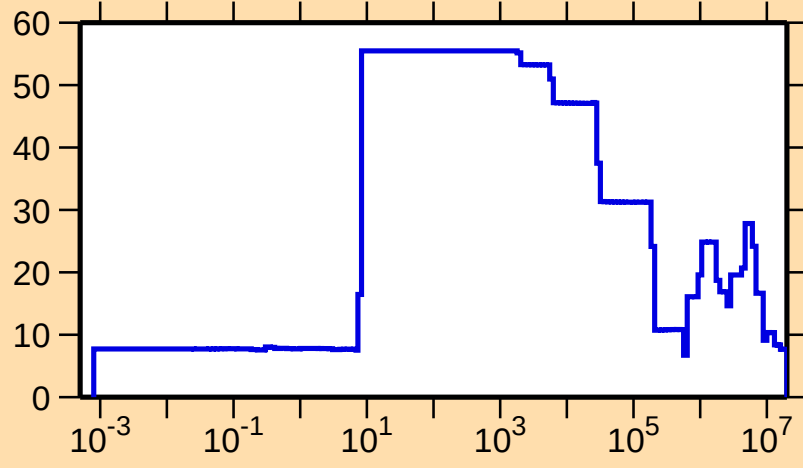
\Delta\sigma/\sigma vs. E for ^{163}\text{Hf}(n,\text{el.})
