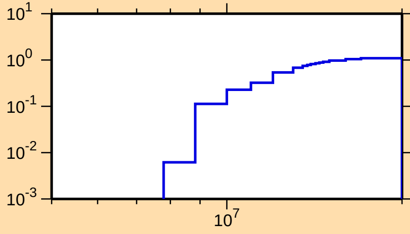
\sigma vs. E for ^{163}\text{Hf}(n,2n)
