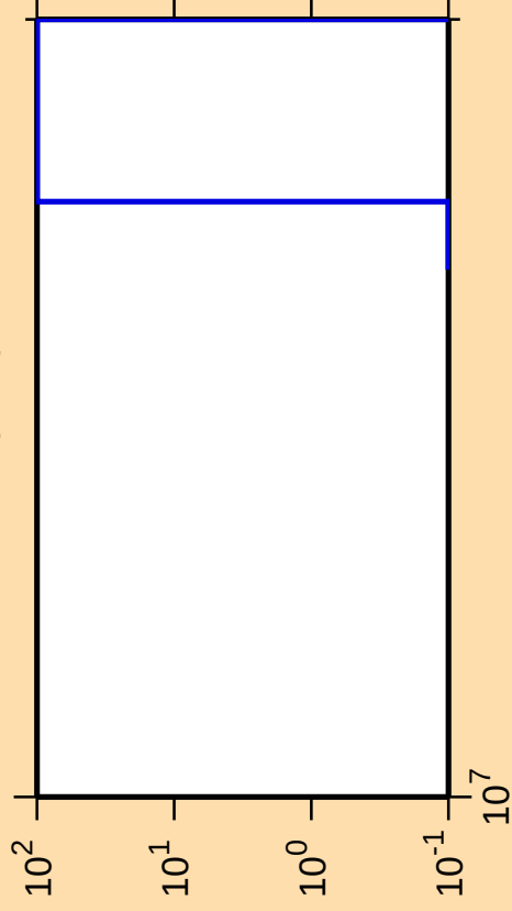
\Delta\sigma/\sigma vs. E for ^{163}\text{Hf}(n,nt)
