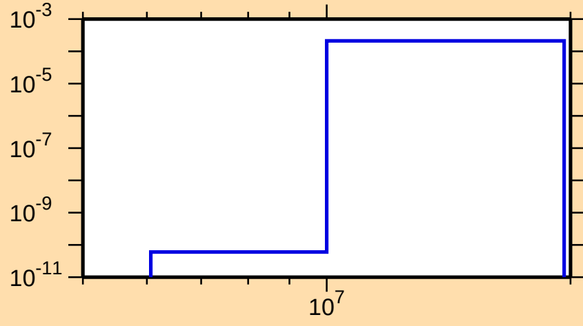
\sigma vs. E for ^{163}\text{Hf}(n,t)
