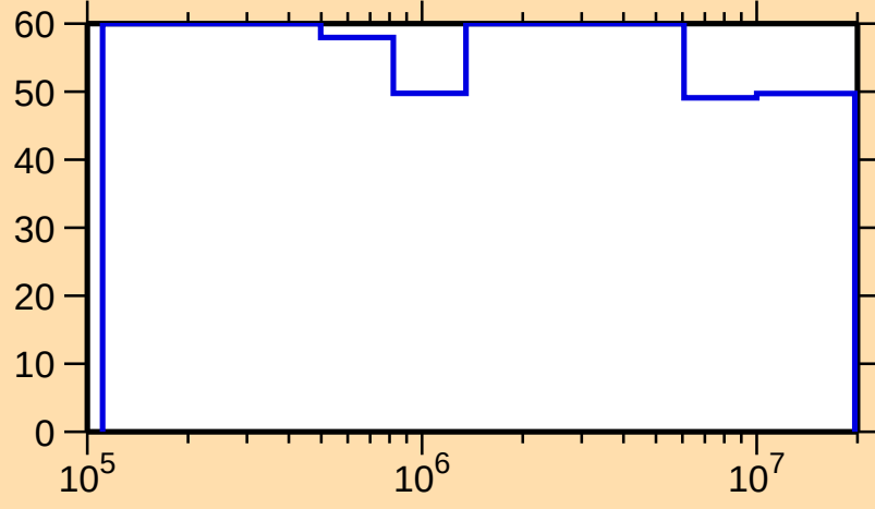
\Delta\sigma/\sigma vs. E for ^{163}\text{Hf}(n,n_1)
