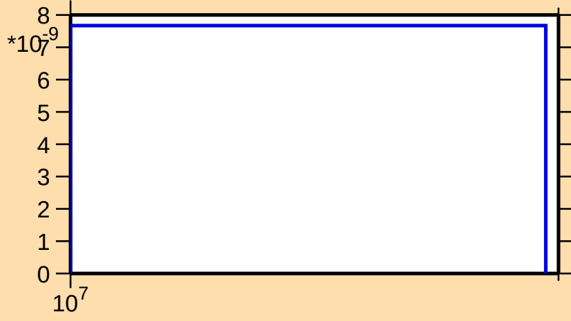
\sigma vs. E for ^{163}\text{Hf}(n,\text{pt})
