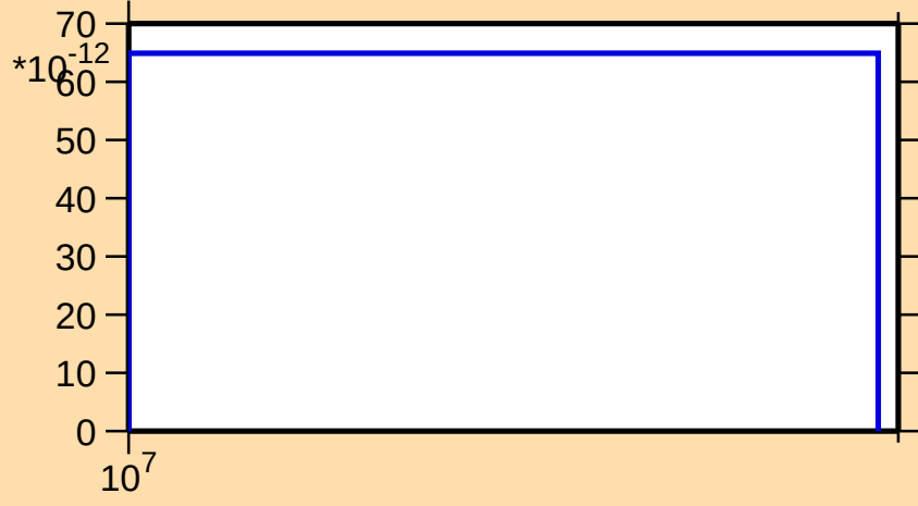
\sigma vs. E for ^{163}\text{Hf} (mt 34)
