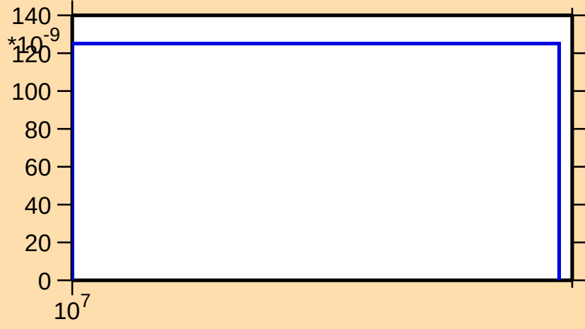
\sigma vs. E for ^{163}\text{Hf}(n,\text{nd})
