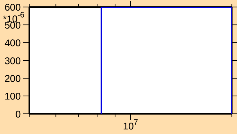
\sigma vs. E for ^{163}\text{Hf}(n,2n\alpha)
