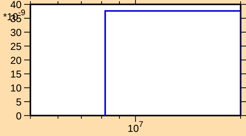
\sigma vs. E for ^{163}\text{Hf}(n,3n)
