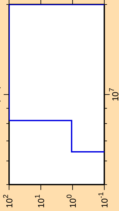
\Delta\sigma/\sigma vs. E for ^{163}\text{Hf}(n,t)
