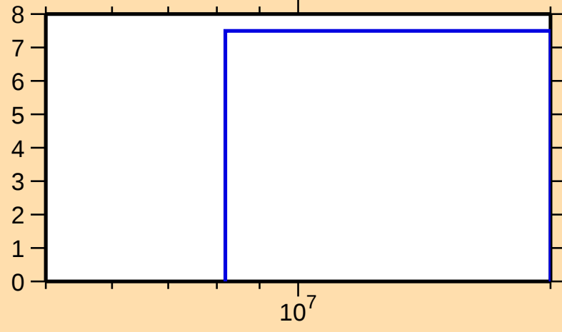
\Delta\sigma/\sigma vs. E for ^{163}\text{Hf}(n,\text{el.})
