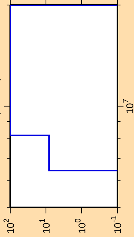
\Delta\sigma/\sigma vs. E for ^{163}\text{Hf}(n,\text{He3})
