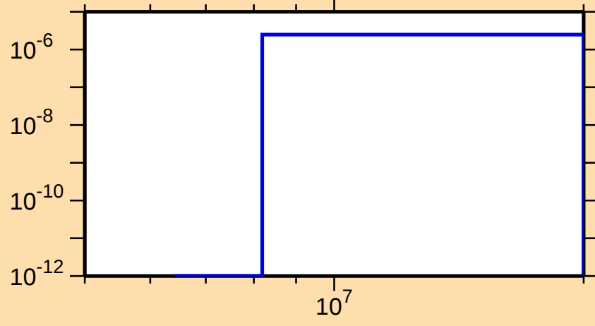
\sigma vs. E for ^{163}\text{Hf}(n,\text{He3})
