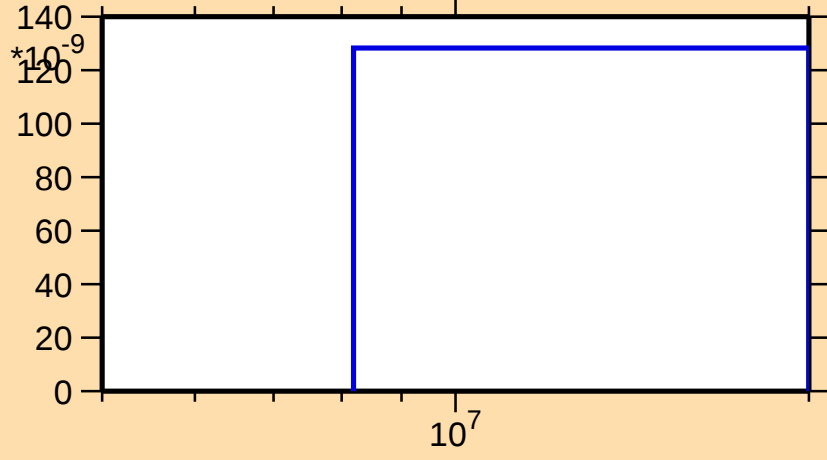
\sigma vs. E for ^{163}\text{Hf}(\text{mt } 45)
