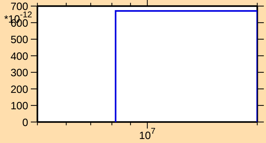
\sigma vs. E for ^{163}\text{Hf}(\text{mt117})
