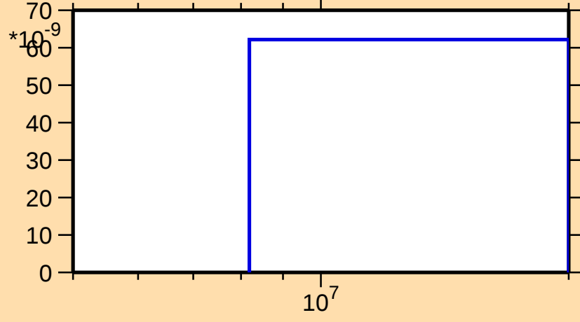
\sigma vs. E for ^{163}\text{Hf}(n,\text{pd})
