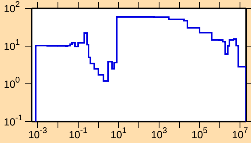
\Delta\sigma/\sigma vs. E for ^{163}\text{Hf}(n,\text{tot.})
