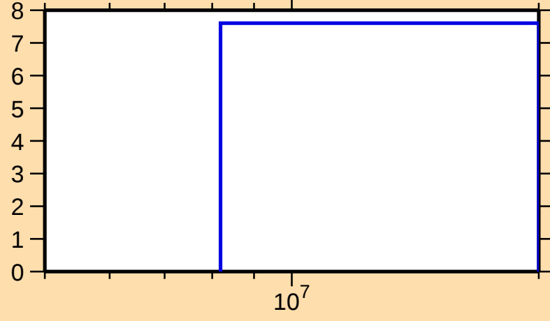
\Delta\sigma/\sigma vs. E for ^{163}\text{Hf}(n,\text{nonel.})
