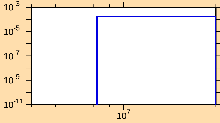
\sigma vs. E for ^{163}\text{Hf}(n,t)
