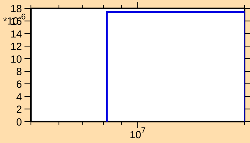
\sigma vs. E for ^{163}\text{Hf}(n,2np)
