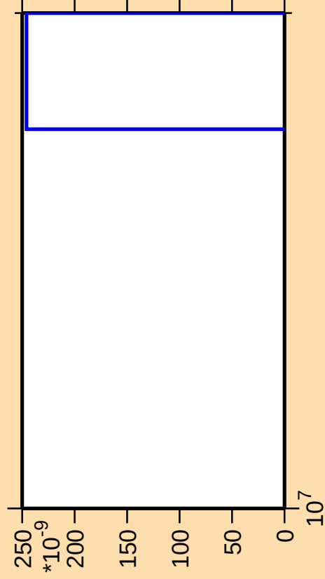
\Delta\sigma/\sigma vs. E for ^{178}\text{Hf}(\text{mt } 11)
