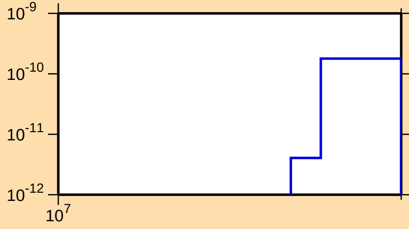
\sigma vs. E for ^{178}\text{Hf}(n,\text{He}3)
