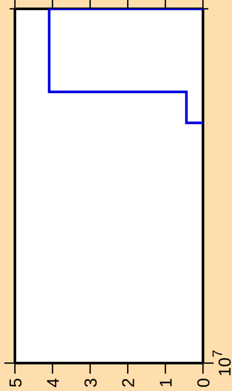
\Delta\sigma/\sigma vs. E for ^{178}\text{Hf}(n,p\alpha)
