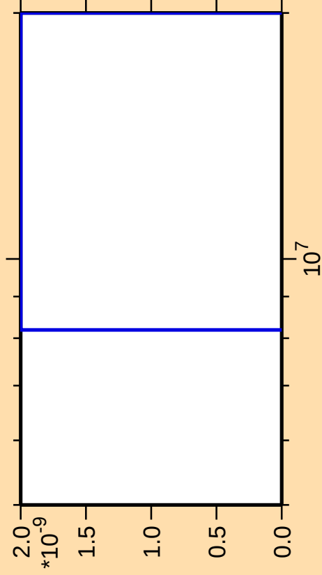
\Delta\sigma/\sigma vs. E for ^{178}\text{Hf}(\text{mt 11})
