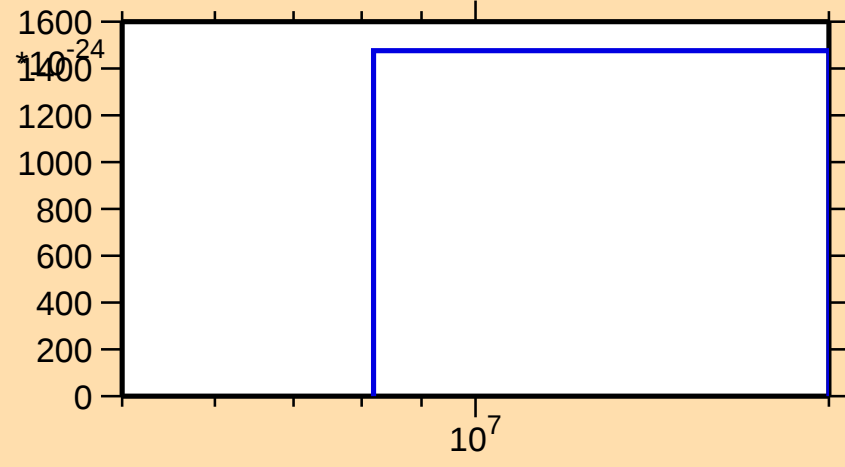
\sigma vs. E for ^{178}\text{Hf}(\text{mt 11})
