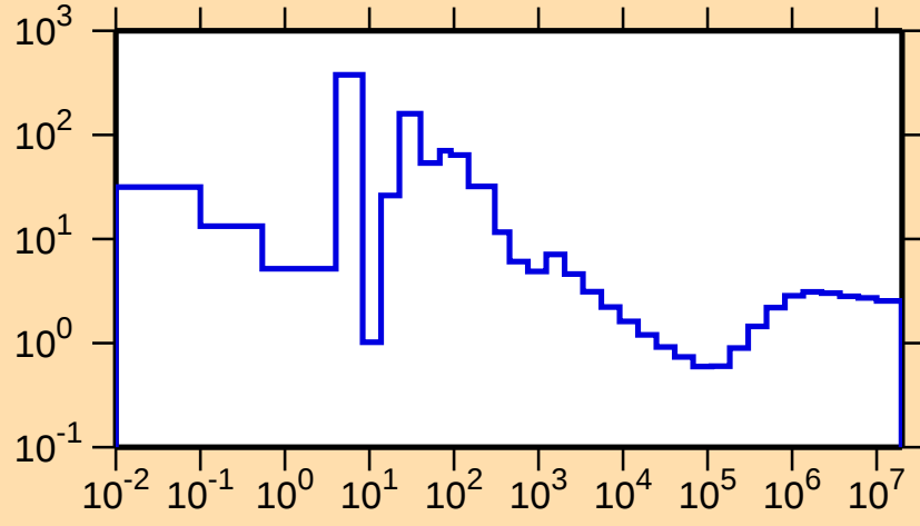
\sigma vs. E for ^{179}\text{Hf}(n,\text{nonel.})
