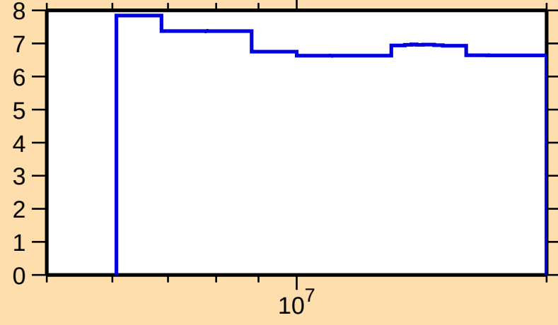
\Delta\sigma/\sigma vs. E for ^{184}\text{Hf}(n,\text{nonel.})
