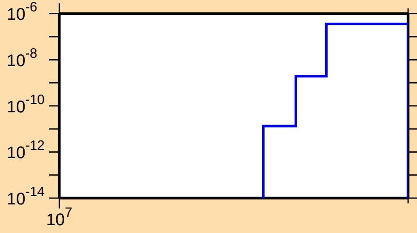
\sigma vs. E for ^{184}\text{Hf}(n,nt)
