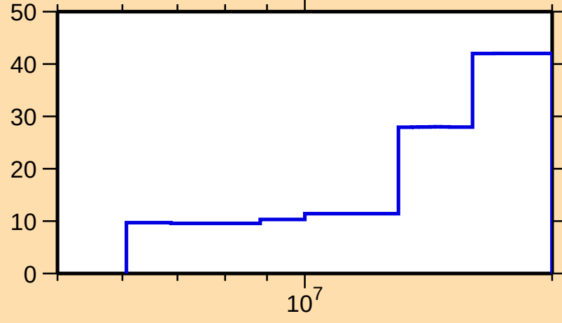
\Delta\sigma/\sigma vs. E for ^{184}\text{Hf}(n,2n)
