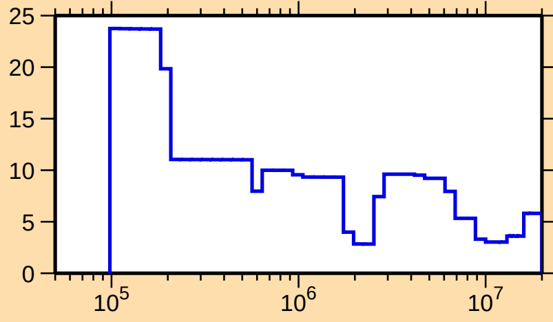
\Delta\sigma/\sigma vs. E for ^{184}\text{Hf}(n,\text{tot.})
