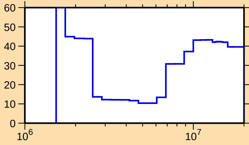
\Delta\sigma/\sigma vs. E for ^{184}\text{Hf}(n,n\text{cont.})
