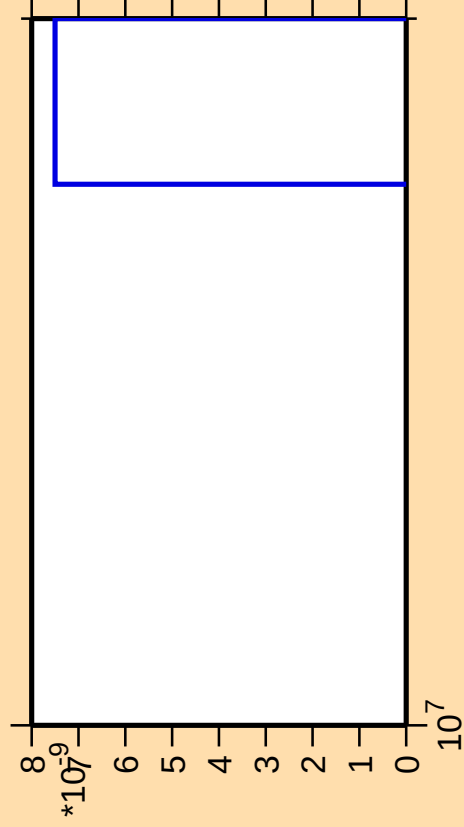
\Delta\sigma/\sigma vs. E for ^{184}\text{Hf}(\text{mt } 11)
