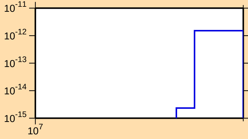
\sigma vs. E for ^{184}\text{Hf}(n,3n\alpha)
