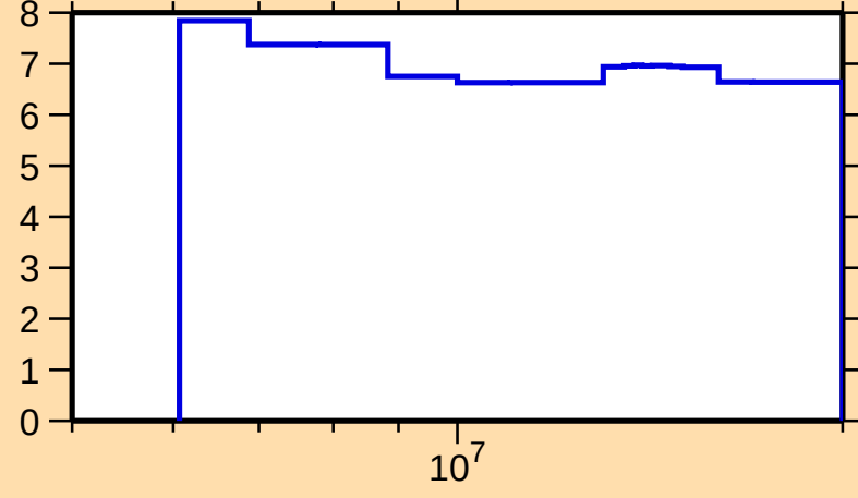
\Delta\sigma/\sigma vs. E for ^{184}\text{Hf}(n,\text{nonel.})
