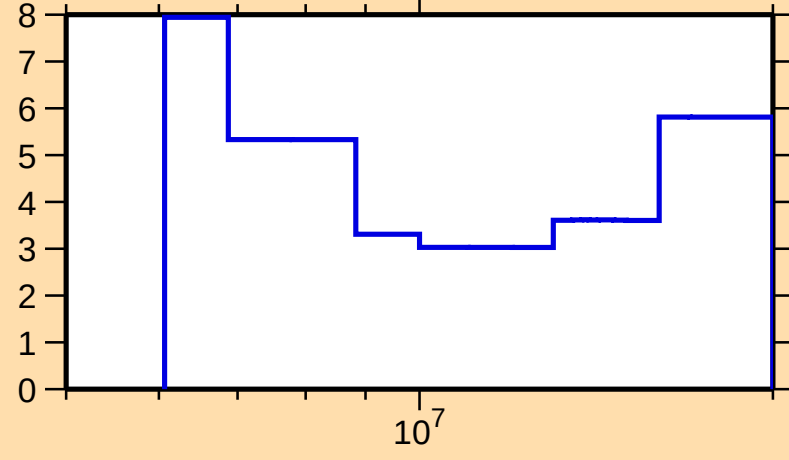
\Delta\sigma/\sigma vs. E for ^{184}\text{Hf}(n,\text{tot.})
