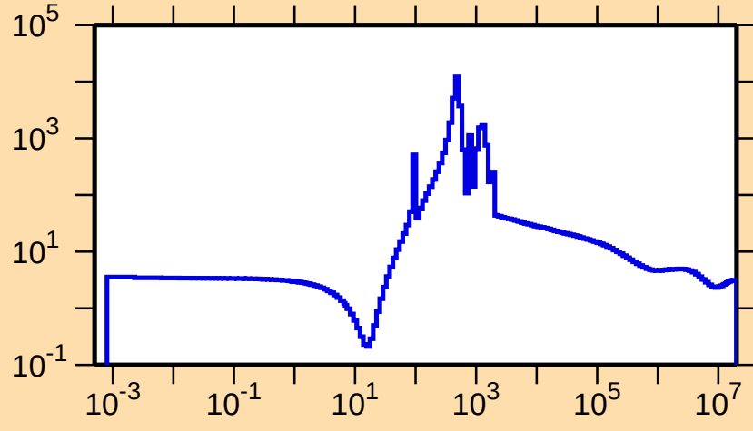
\sigma vs. E for ^{184}\text{Hf}(n,\text{el.})
