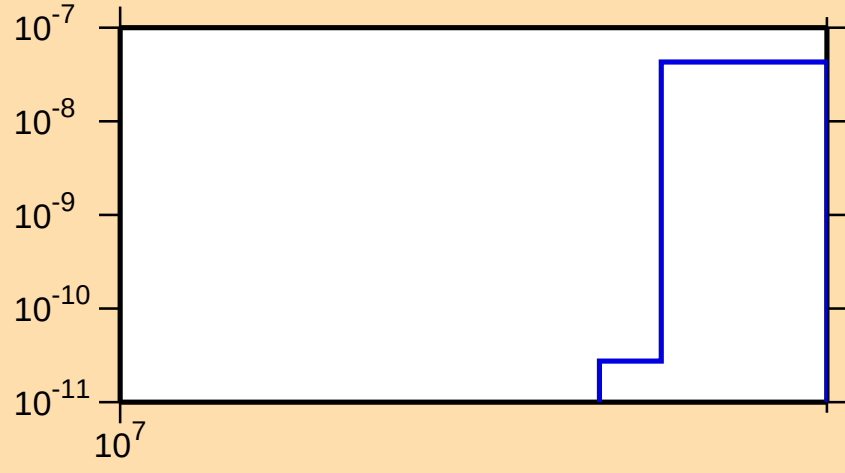
\sigma vs. E for ^{184}\text{Hf}(n,\text{nd})
