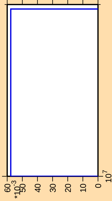
\Delta\sigma/\sigma vs. E for ^{184}\text{Hf}(n,3n\alpha)
