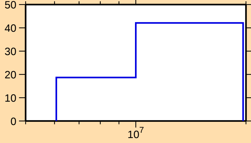
\Delta\sigma/\sigma vs. E for ^{184}\text{Hf}(n,n\text{cont.})
