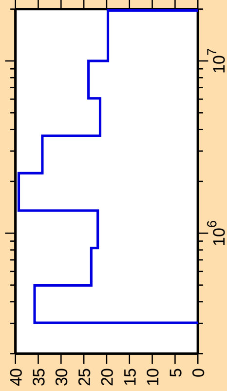
\Delta\sigma/\sigma vs. E for ^{184}\text{Hf}(n,n_2)
