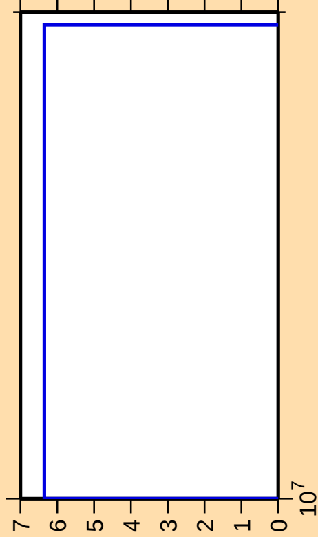
\Delta\sigma/\sigma vs. E for ^{184}\text{Hf}(n,2np)
