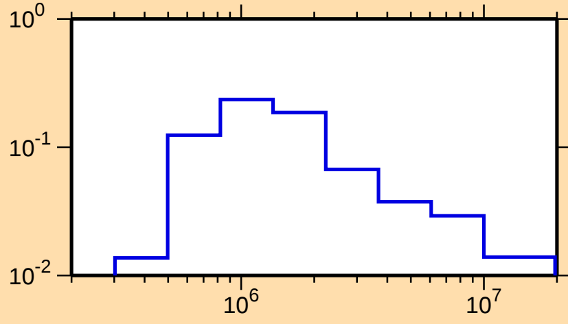
\sigma vs. E for ^{184}\text{Hf}(n,n_2)
