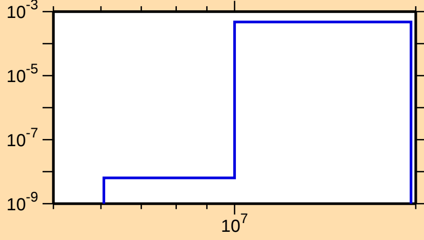
\sigma vs. E for ^{184}\text{Hf}(n,p)
