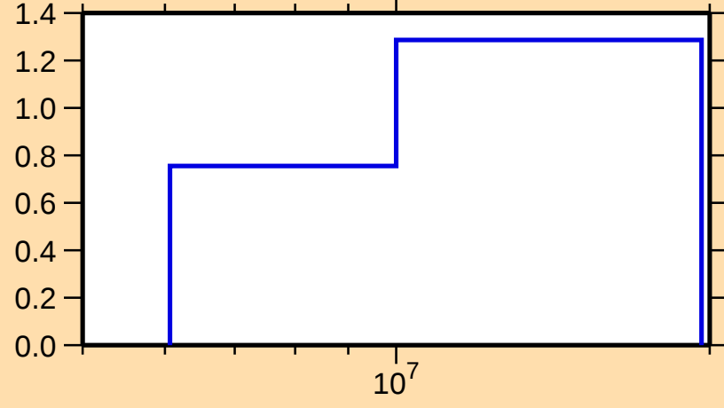
\sigma vs. E for ^{184}\text{Hf}(n,2n)
