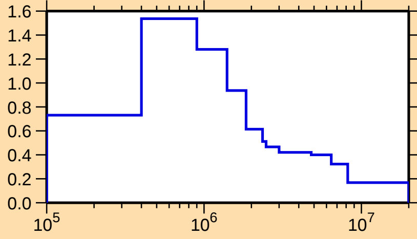
\sigma vs. E for ^{184}\text{Hf}(n,n_1)
