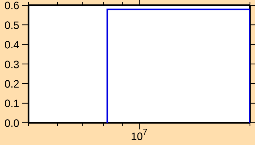
\sigma vs. E for ^{184}\text{Hf}(n,3n)
