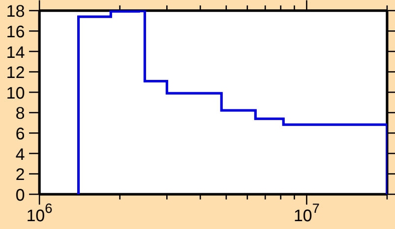
\Delta\sigma/\sigma vs. E for ^{184}\text{Hf}(n,\text{nonel.})
