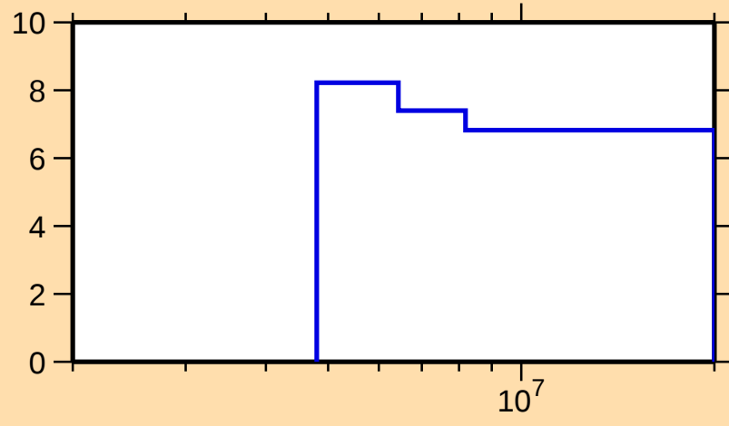
\Delta\sigma/\sigma vs. E for ^{184}\text{Hf}(n,\text{nonel.})
