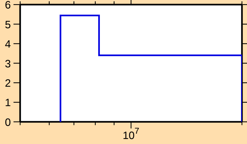
\Delta\sigma/\sigma vs. E for ^{184}\text{Hf}(n,\text{el.})
