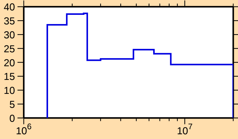
\Delta\sigma/\sigma vs. E for ^{184}\text{Hf}(n,n_1)
