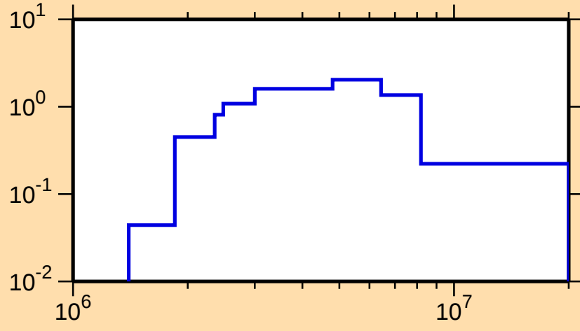
\sigma vs. E for ^{184}\text{Hf}(n,n\text{cont.})
