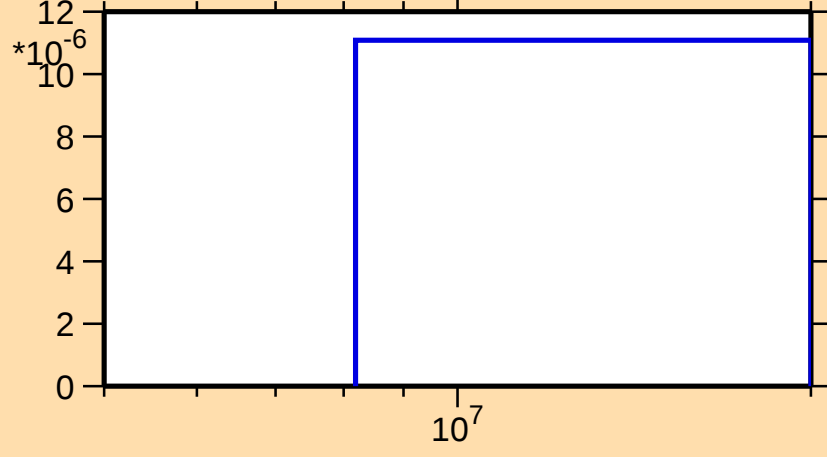
\sigma vs. E for ^{184}\text{Hf}(n,np)
