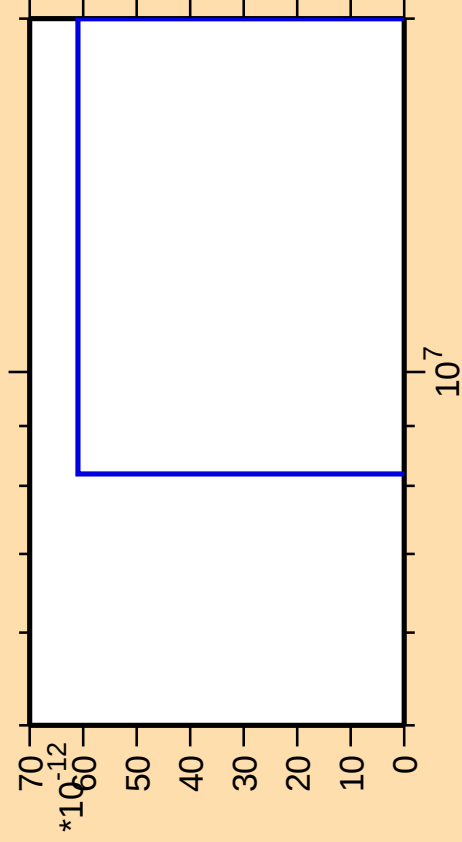
\Delta\sigma/\sigma vs. E for ^{184}\text{Hf}(\text{mt } 11)
