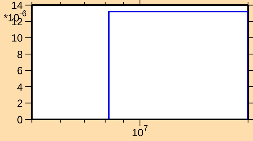
\sigma vs. E for ^{184}\text{Hf}(n,d)
