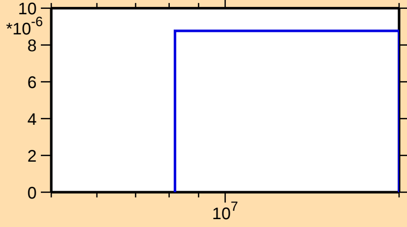
\sigma vs. E for ^{184}\text{Hf}(n,t)
