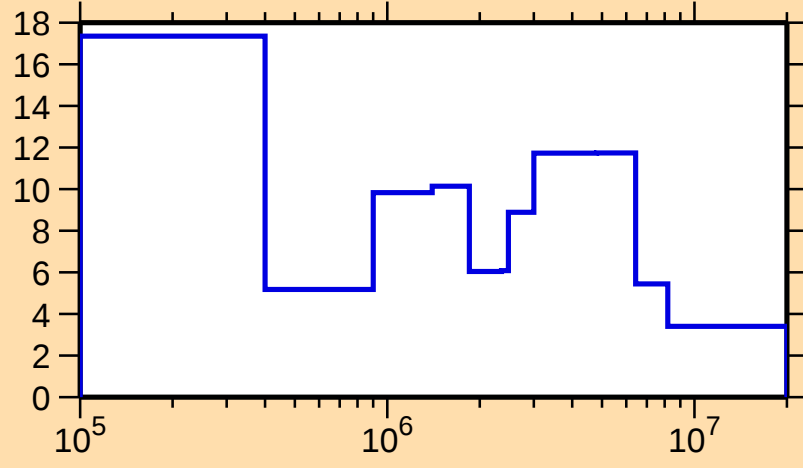
\Delta\sigma/\sigma vs. E for ^{184}\text{Hf}(n,\text{el.})
