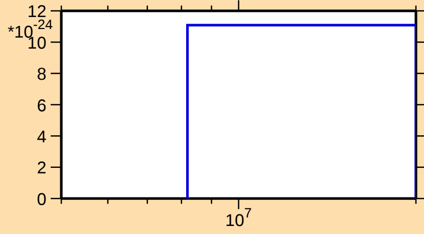
\sigma vs. E for ^{184}\text{Hf}(\text{mt } 11)
