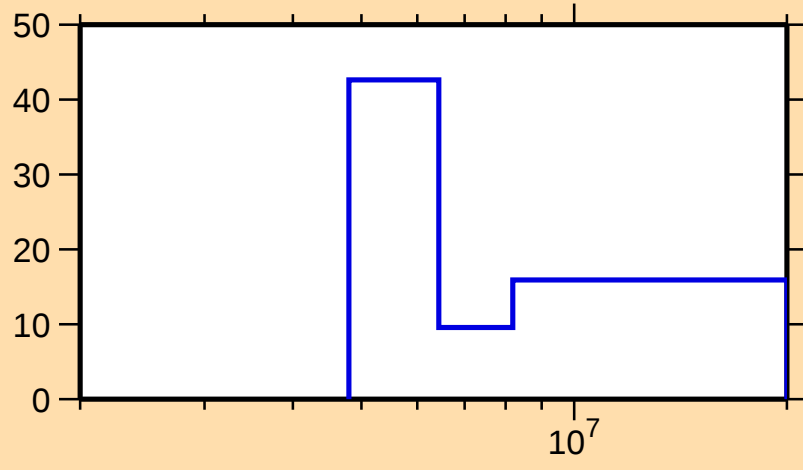
\Delta\sigma/\sigma vs. E for ^{184}\text{Hf}(n,2n)
