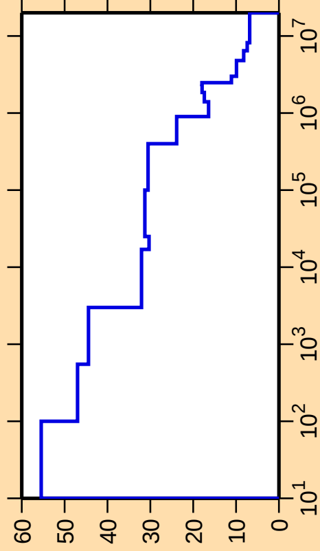
\Delta\sigma/\sigma vs. E for ^{184}\text{Hf}(n,\text{nonel.})
