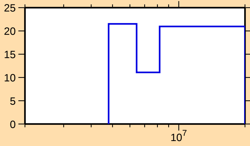
\Delta\sigma/\sigma vs. E for ^{186}\text{Hf}(n,2n)
