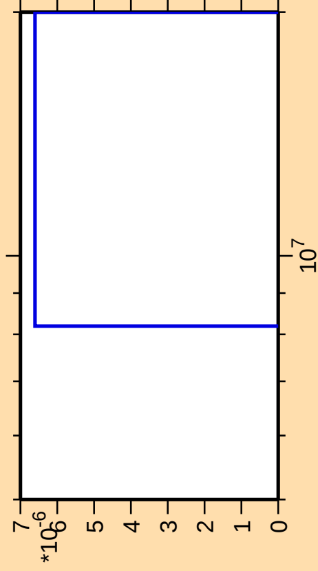
\Delta\sigma/\sigma vs. E for ^{186}\text{Hf}(\text{mt } 11)
