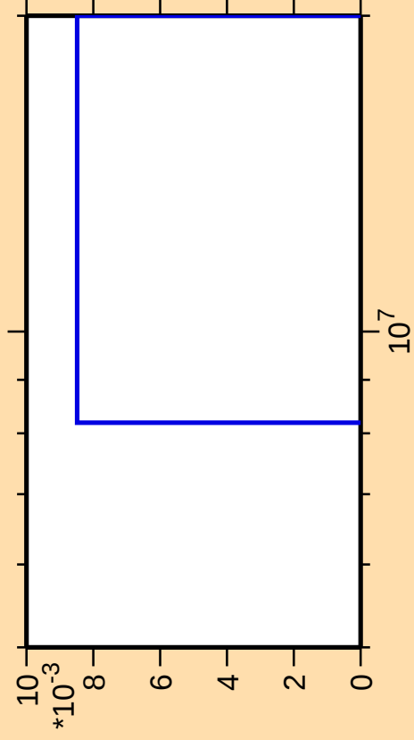
\Delta\sigma/\sigma vs. E for ^{186}\text{Hf}(n,3n\alpha)
