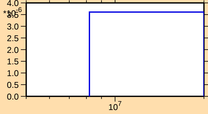
\sigma vs. E for ^{186}\text{Hf}(n,np)
