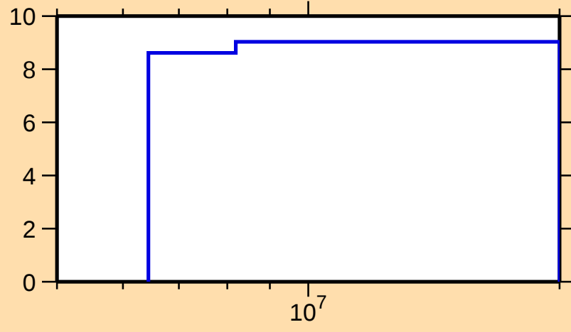
\Delta\sigma/\sigma vs. E for ^{186}\text{Hf}(n,\text{nonel.})
