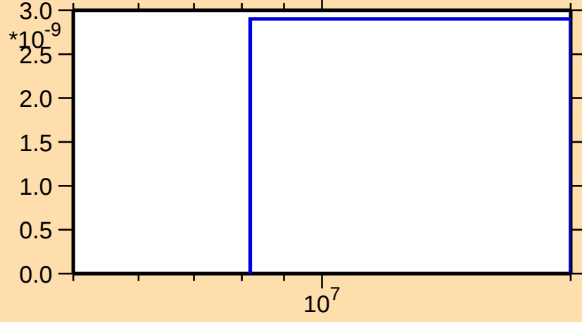
\sigma vs. E for ^{186}\text{Hf}(n,nt)
