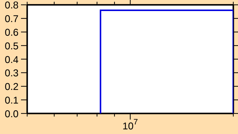
\sigma vs. E for ^{186}\text{Hf}(n,3n)
