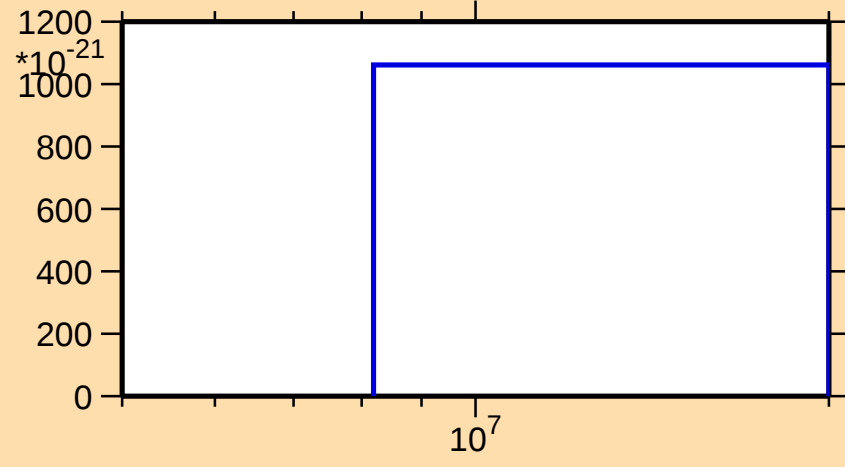
\sigma vs. E for ^{186}\text{Hf}(\text{mt } 11)
