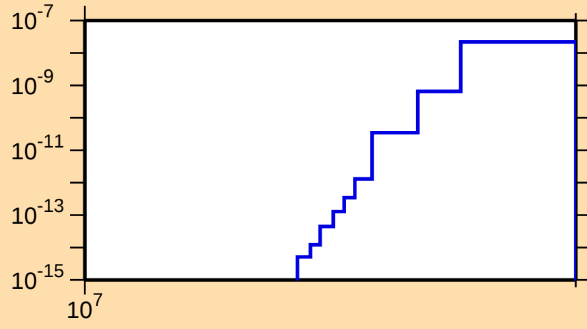
\sigma vs. E for ^{118}\text{I} (mt 34)
