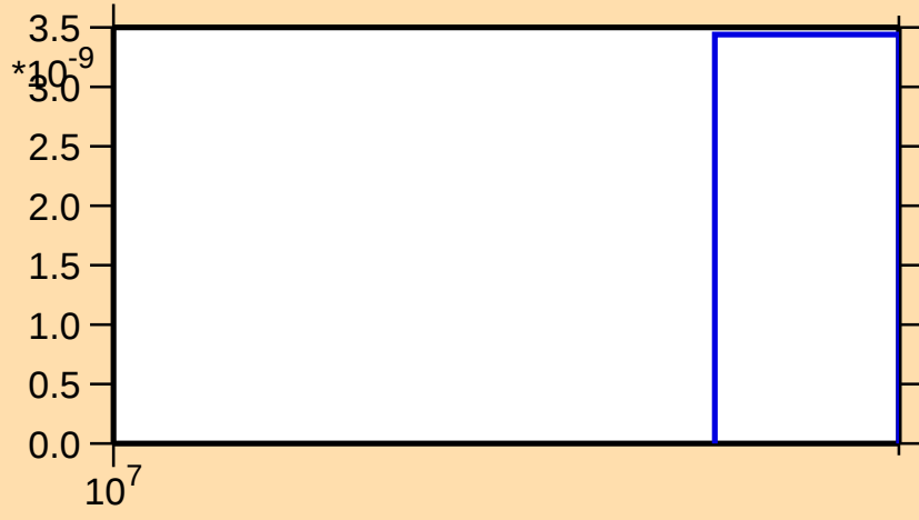
\sigma vs. E for ^{118}\text{I}(n,3n)
