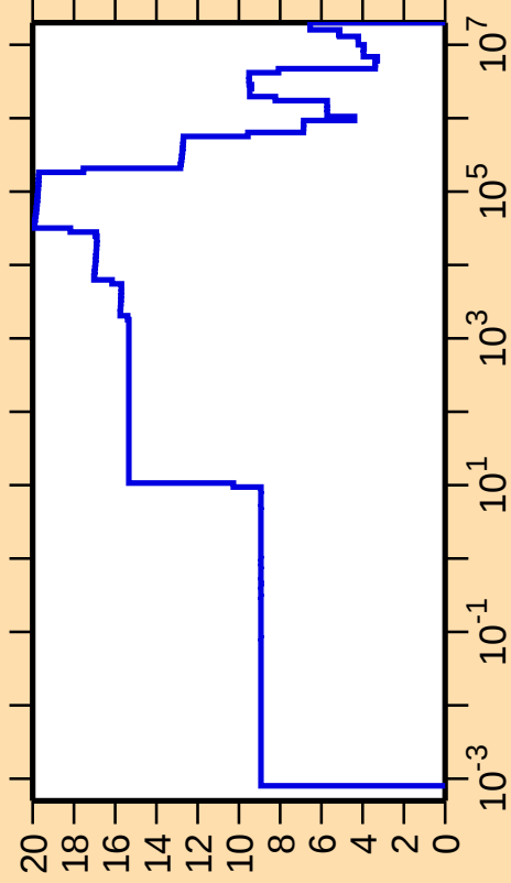
\Delta\sigma/\sigma vs. E for ^{120}\text{I}(\text{n,el.})
