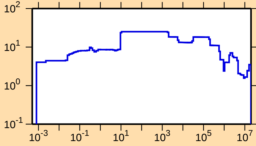
\Delta\sigma/\sigma vs. E for ^{120}\text{I}(\text{n,tot.})
