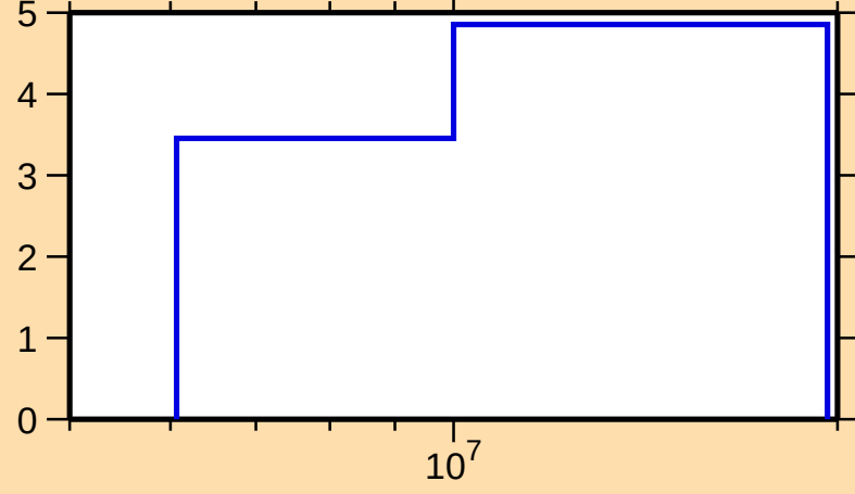
\Delta\sigma/\sigma vs. E for ^{120}\text{I}(n,\text{el.})
