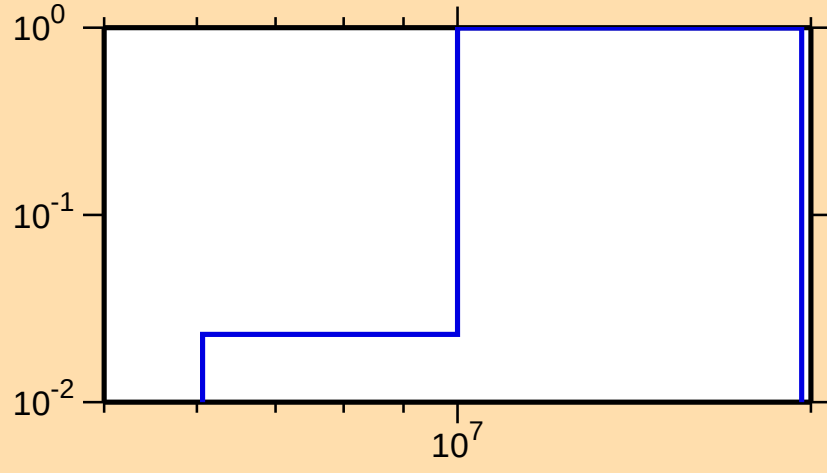
\sigma vs. E for ^{120}\text{I}(n,2n)
