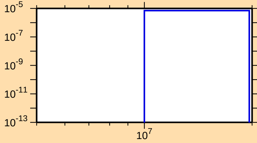
\sigma vs. E for ^{120}\text{I}(n,\text{nd})
