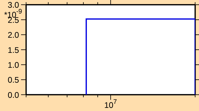
\sigma vs. E for ^{120}\text{I}(n,\text{pd})
