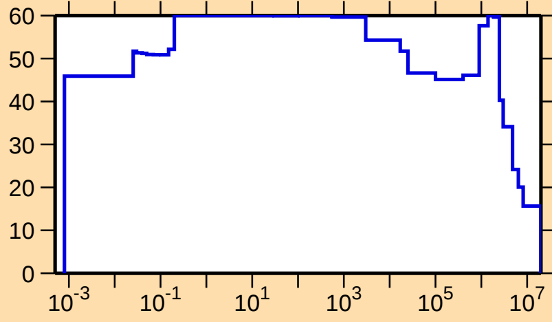
\Delta\sigma/\sigma vs. E for ^{120}\text{I}(n,p)
