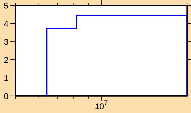
\Delta\sigma/\sigma vs. E for ^{120}\text{I}(n,\text{el.})
