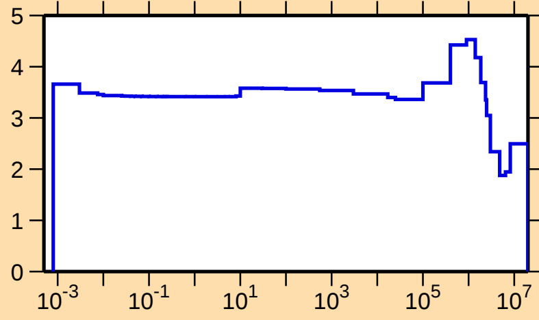
\sigma vs. E for ^{120}\text{I}(n,\text{el.})
