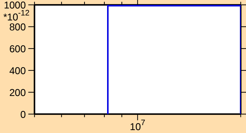
\sigma vs. E for ^{120}\text{I}(\text{n},\text{nt})
