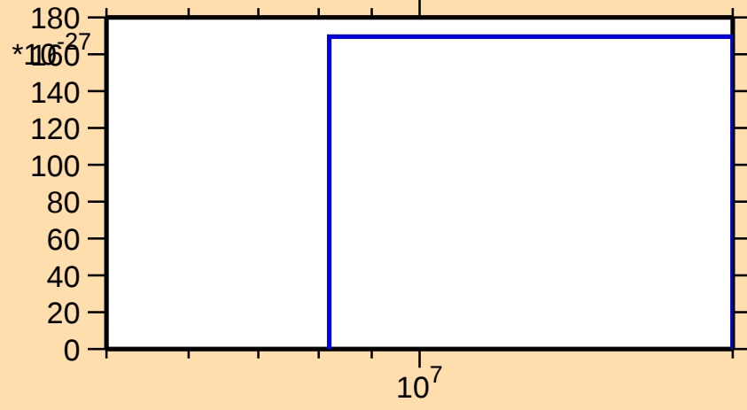
\sigma vs. E for ^{120}\text{I}(\text{mt 11})
