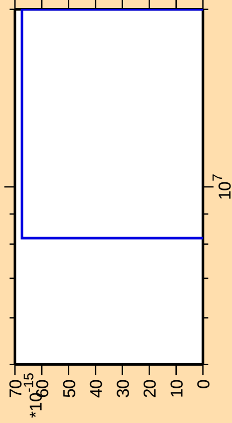
\Delta\sigma/\sigma vs. E for ^{120}\text{I}(\text{mt 11})
