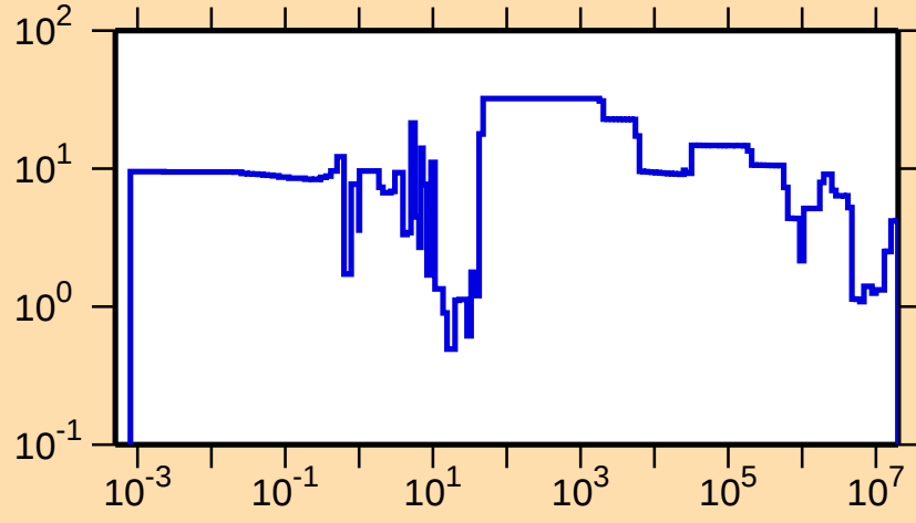
\Delta\sigma/\sigma vs. E for ^{122}\text{I}(\text{n,tot.})
