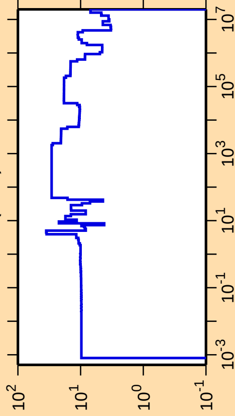
\Delta\sigma/\sigma vs. E for ^{122}\text{I}(\text{n,el.})
