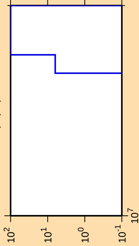
\Delta\sigma/\sigma vs. E for ^{122}\text{I}(\text{n},\text{pd})
