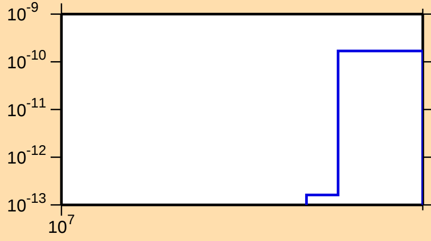
\sigma vs. E for ^{122}\text{I}(\text{n},\text{pt})
