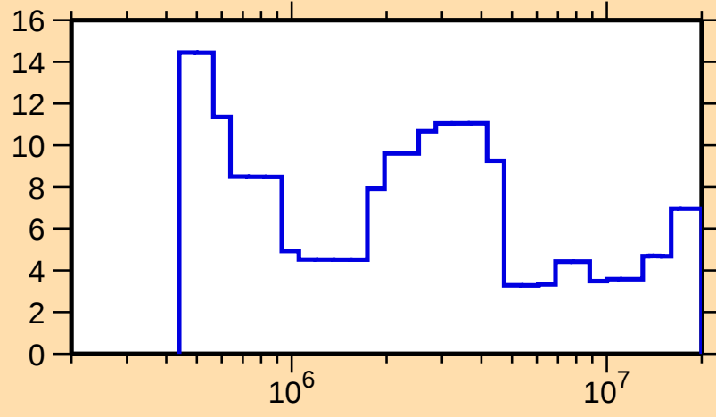
\Delta\sigma/\sigma vs. E for ^{122}\text{I}(\text{n},\text{el.})
