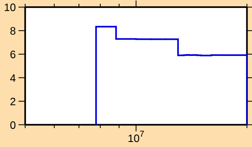
\Delta\sigma/\sigma vs. E for ^{122}\text{I}(n,2n)
