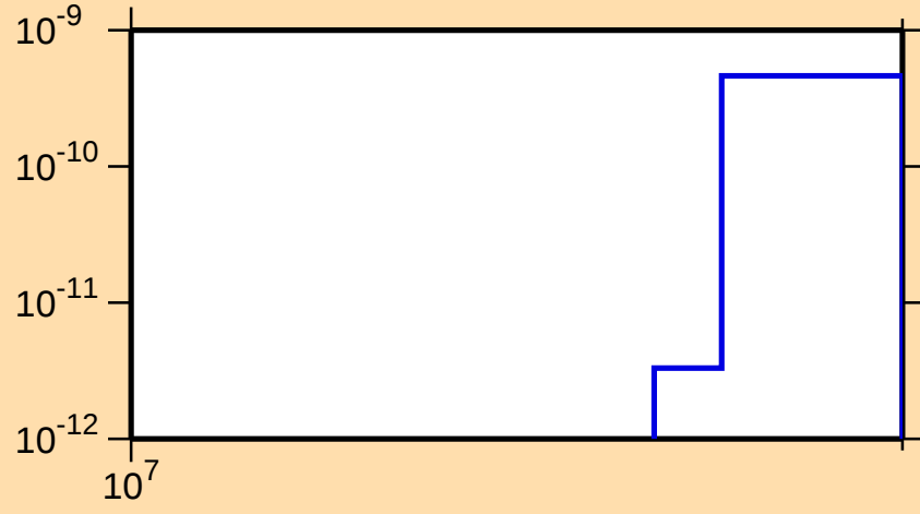
\sigma vs. E for ^{122}\text{I}(\text{n},\text{pd})
