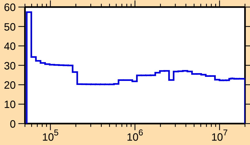
\Delta\sigma/\sigma vs. E for ^{122}\text{I}(n,n_1)
