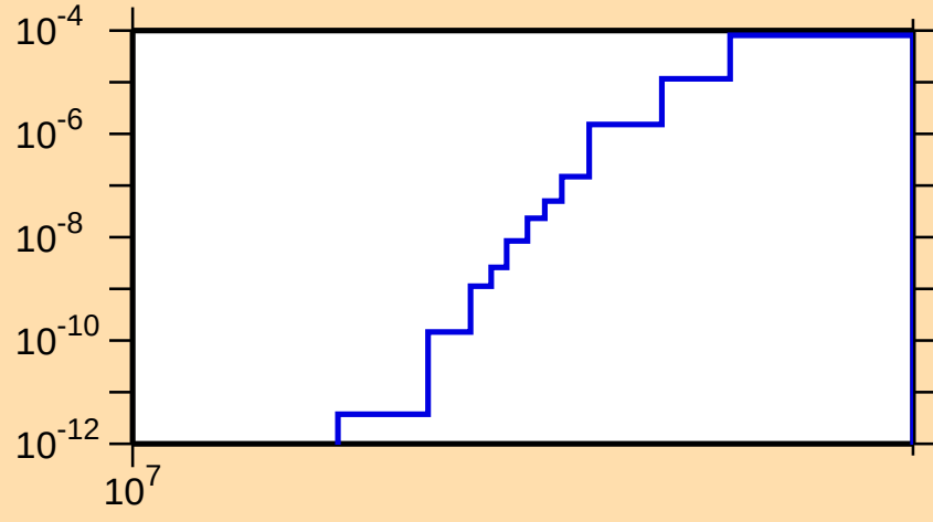
\sigma vs. E for ^{124}\text{I}(\text{n},\text{nd})
