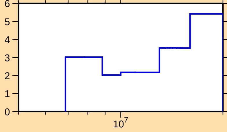
\Delta\sigma/\sigma vs. E for ^{124}\text{I}(n,\text{el.})
