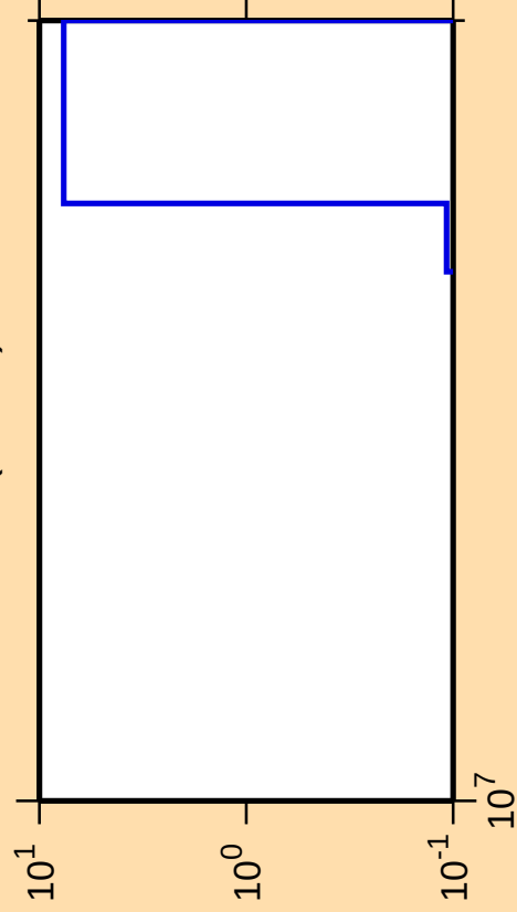
\Delta\sigma/\sigma vs. E for ^{124}\text{I} (mt 45)
