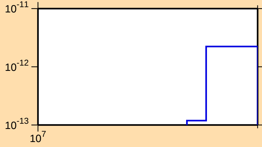
\sigma vs. E for ^{136}\text{I}(n,p\alpha)
