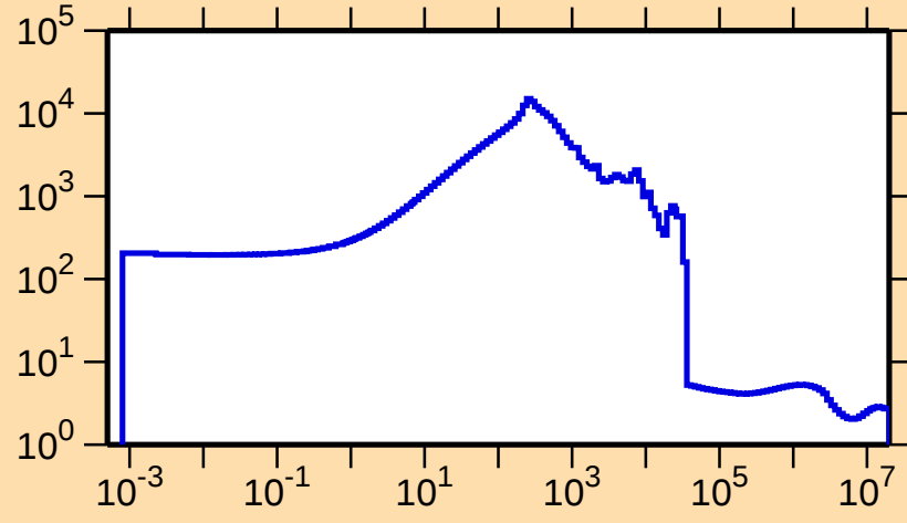
\sigma vs. E for ^{136}\text{I}(\text{n},\text{el.})
