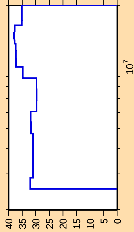
\Delta\sigma/\sigma vs. E for ^{136}\text{I}(\text{n},\text{ncont.})
