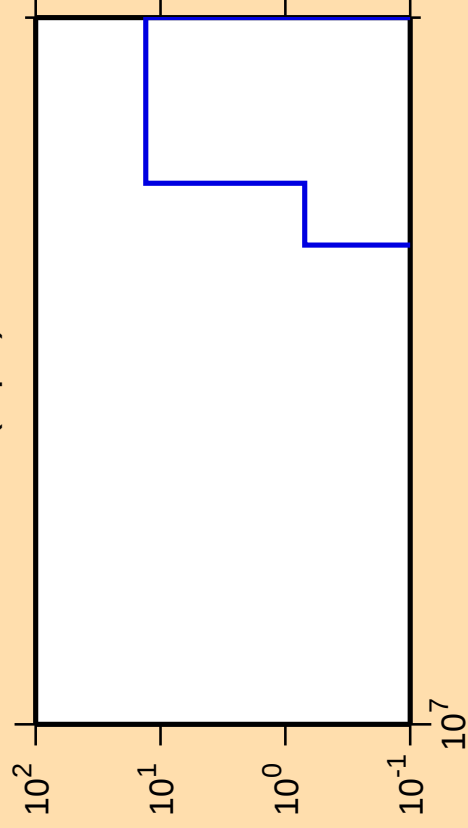
\Delta\sigma/\sigma vs. E for ^{136}\text{I}(n,p\alpha)
