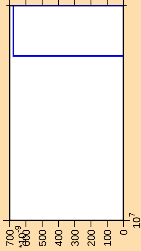
\Delta\sigma/\sigma vs. E for ^{136}\text{I}(\text{mt } 42)
