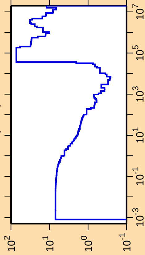
\Delta\sigma/\sigma vs. E for ^{136}\text{I}(\text{n},\text{el.})
