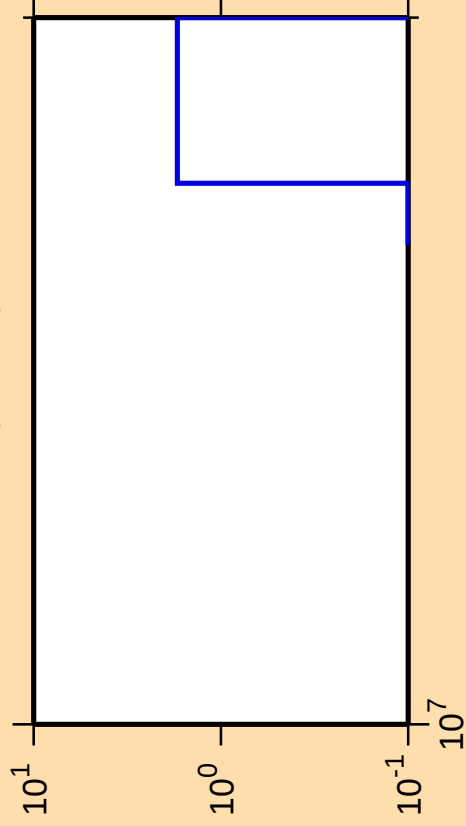
\Delta\sigma/\sigma vs. E for ^{136}\text{I}(n,\text{He}3)
