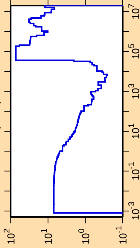
\Delta\sigma/\sigma vs. E for ^{136}\text{I}(\text{n,el.})
