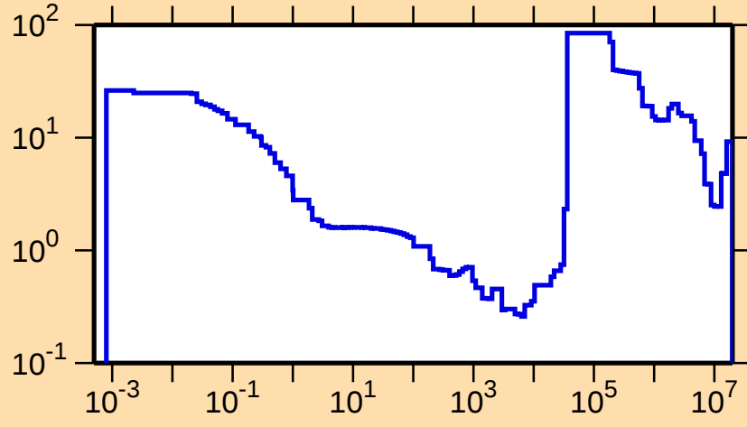
\Delta\sigma/\sigma vs. E for ^{136}\text{I}(\text{n,tot.})
