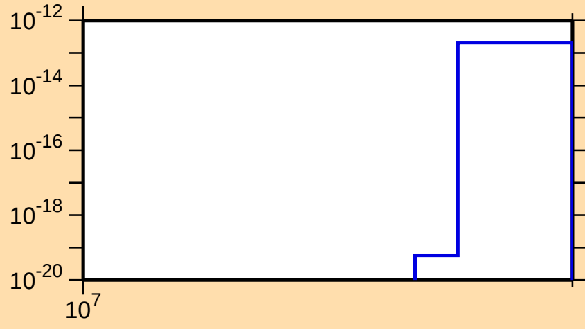
\sigma vs. E for ^{136}\text{I}(n,\text{He}3)
