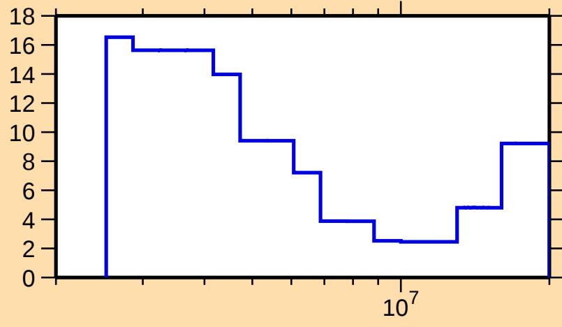
\Delta\sigma/\sigma vs. E for ^{136}\text{I}(\text{n},\text{tot.})
