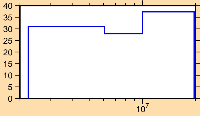
\Delta\sigma/\sigma vs. E for ^{136}\text{I}(n,n\text{cont.})
