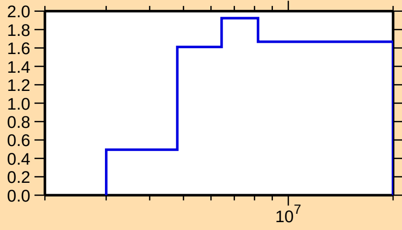
\sigma vs. E for ^{136}\text{I}(n,2n)
