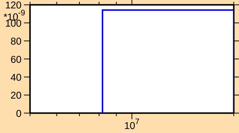
\sigma vs. E for ^{136}\text{I}(n,2np)
