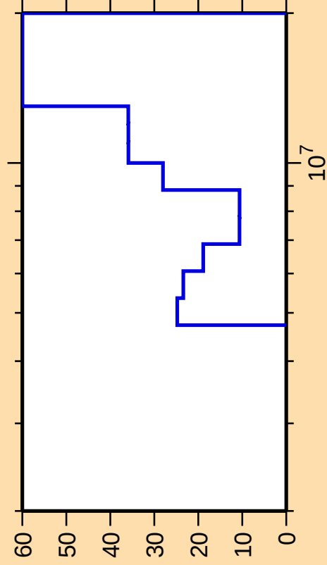
\Delta\sigma/\sigma vs. E for ^{137}\text{I}(n,2n)
