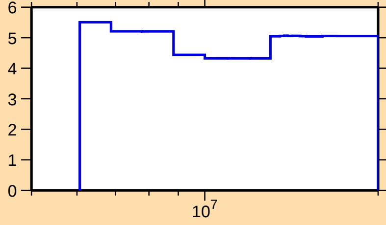
\Delta\sigma/\sigma vs. E for ^{137}\text{I}(n,\text{tot.})
