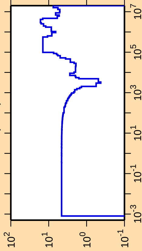
\Delta\sigma/\sigma vs. E for ^{137}\text{I}(n,\text{el.})
