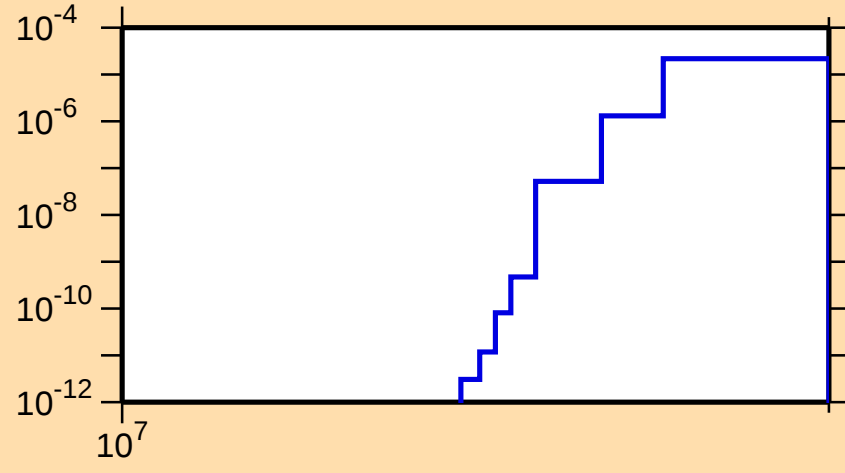
\sigma vs. E for ^{137}\text{I}(n,\text{nd})
