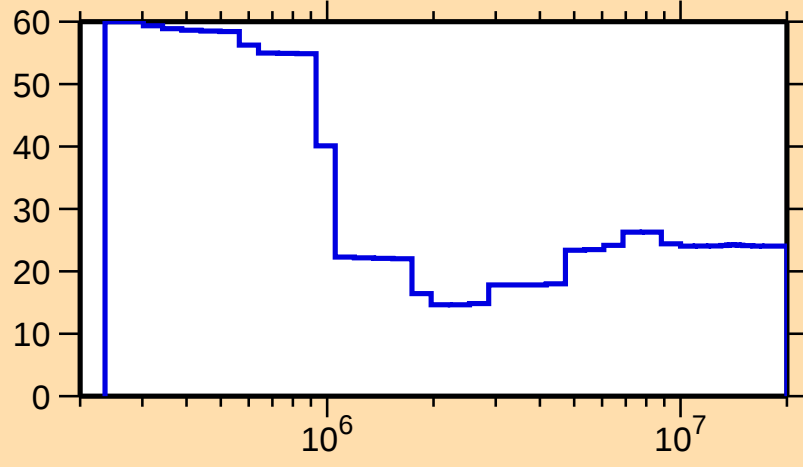
\Delta\sigma/\sigma vs. E for ^{137}\text{I}(n,n_1)
