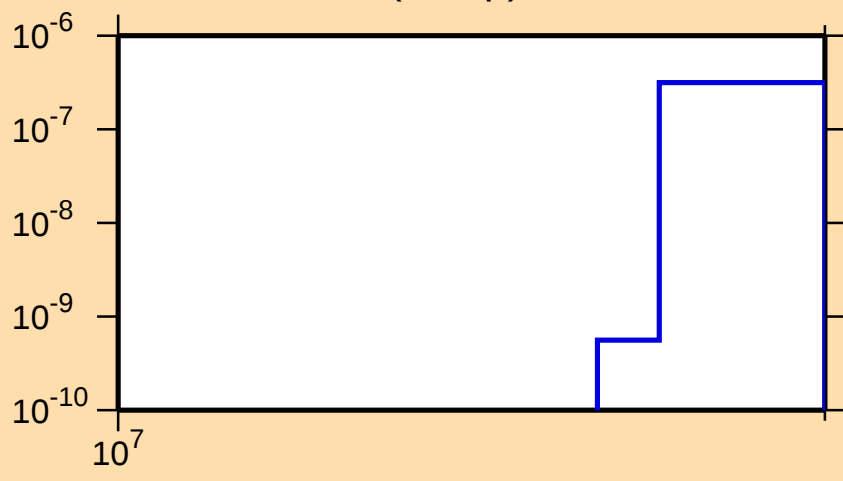
\sigma vs. E for ^{137}\text{I}(n,2np)
