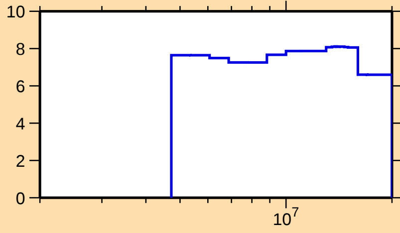
\Delta\sigma/\sigma vs. E for ^{137}\text{I}(n,\text{nonel.})
