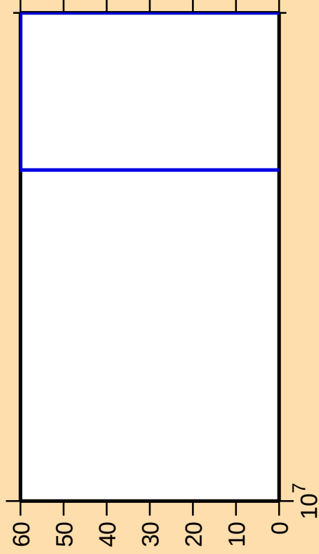
\Delta\sigma/\sigma vs. E for ^{137}\text{I}(n,2np)
