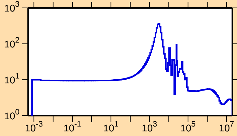
\sigma vs. E for ^{137}\text{I}(n,\text{el.})
