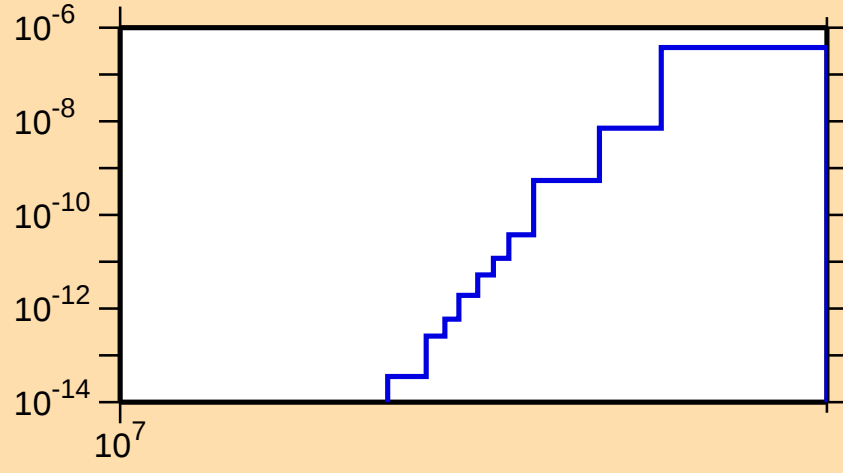
\sigma vs. E for ^{137}\text{I}(n,2n\alpha)
