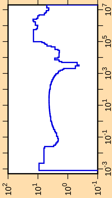
\Delta\sigma/\sigma vs. E for ^{137}\text{I}(n,\text{tot.})
