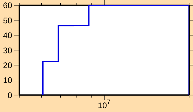
\Delta\sigma/\sigma vs. E for ^{137}\text{I}(n,n\text{cont.})
