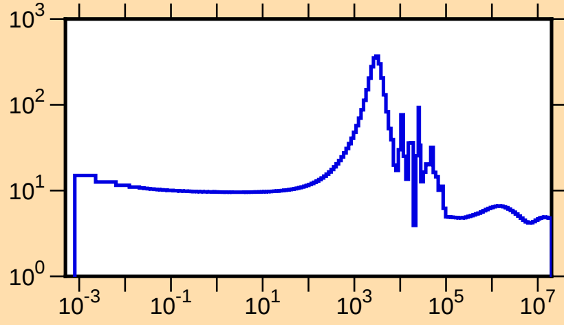
\sigma vs. E for ^{137}\text{I}(n,\text{tot.})
