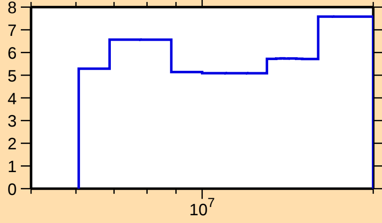
\Delta\sigma/\sigma vs. E for ^{137}\text{I}(\text{n,el.})
