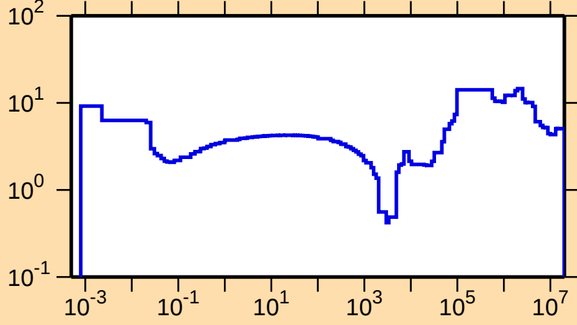
\Delta\sigma/\sigma vs. E for ^{137}\text{I}(\text{n,tot.})
