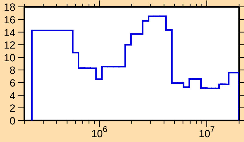
\Delta\sigma/\sigma vs. E for ^{137}\text{I}(\text{n,el.})
