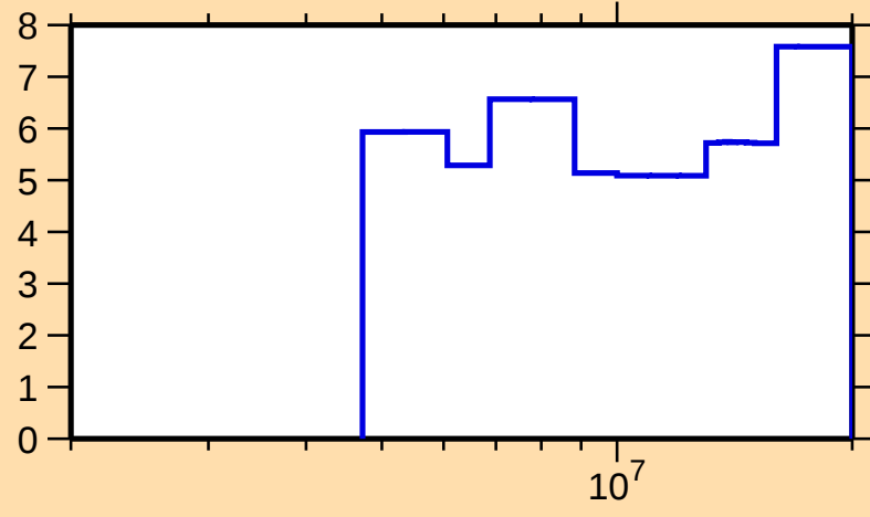
\Delta\sigma/\sigma vs. E for ^{137}\text{I}(n,\text{el.})
