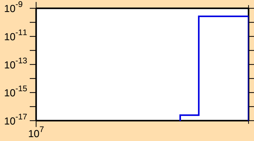
\sigma vs. E for ^{137}\text{I} (mt 11)
