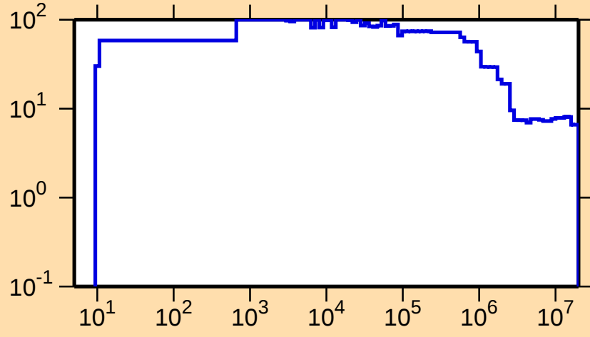
\Delta\sigma/\sigma vs. E for ^{137}\text{I}(n,\text{nonel.})
