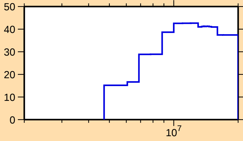
\Delta\sigma/\sigma vs. E for ^{137}\text{I}(n,\text{inel.})
