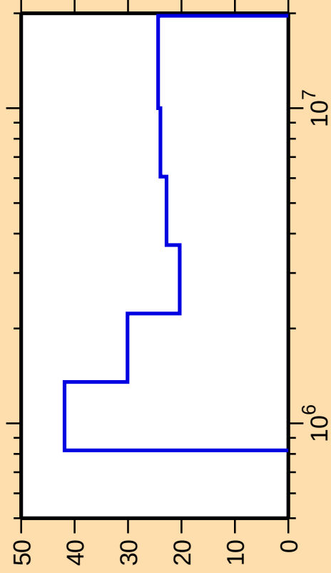
\Delta\sigma/\sigma vs. E for ^{137}\text{I}(n,n_4)
