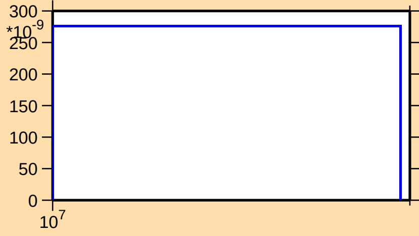
\sigma vs. E for ^{137}\text{I}(n,\text{nd})
