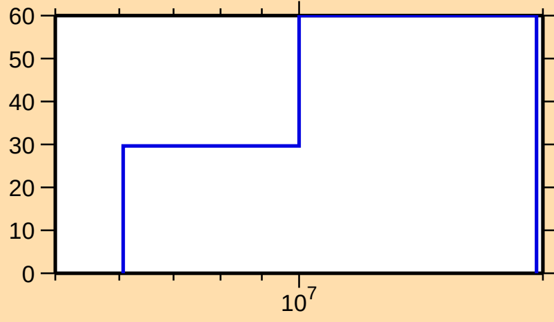
\Delta\sigma/\sigma vs. E for ^{137}\text{I}(n,\text{ncont.})
