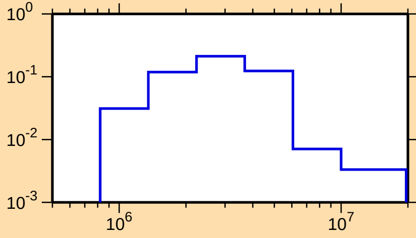
\sigma vs. E for ^{137}\text{I}(n,n_4)
