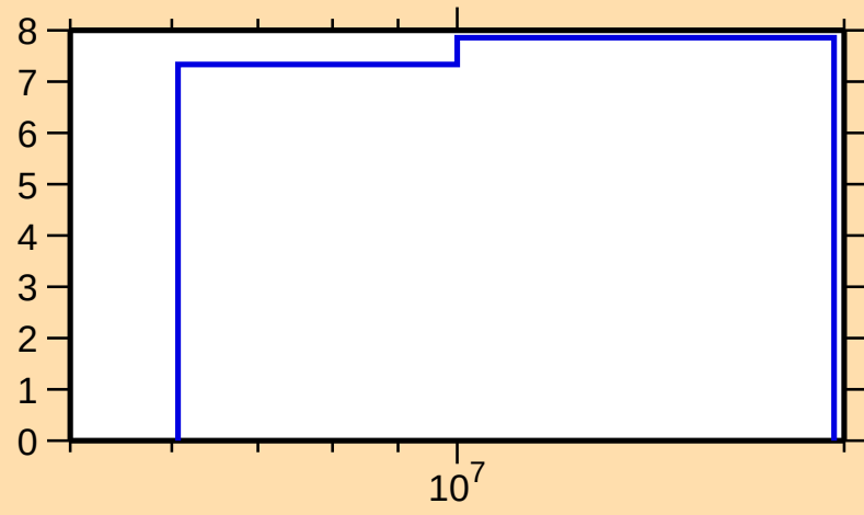
\Delta\sigma/\sigma vs. E for ^{137}\text{I}(\text{n,nonel.})
