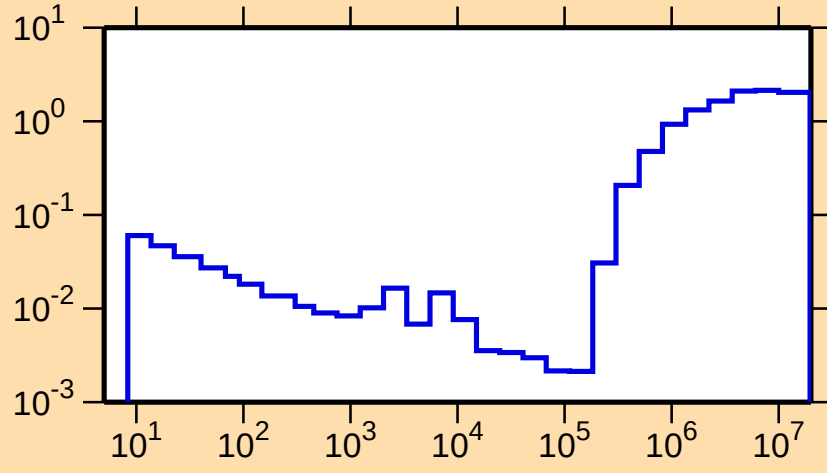
\sigma vs. E for ^{137}\text{I}(n,\text{nonel.})
