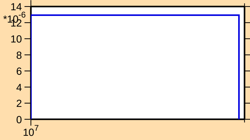
\sigma vs. E for ^{137}\text{I}(n,nt)
