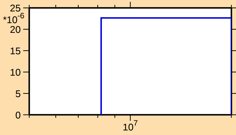
\sigma vs. E for ^{137}\text{I}(n,np)
