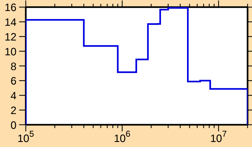
\Delta\sigma/\sigma vs. E for ^{137}\text{I}(n,\text{el.})
