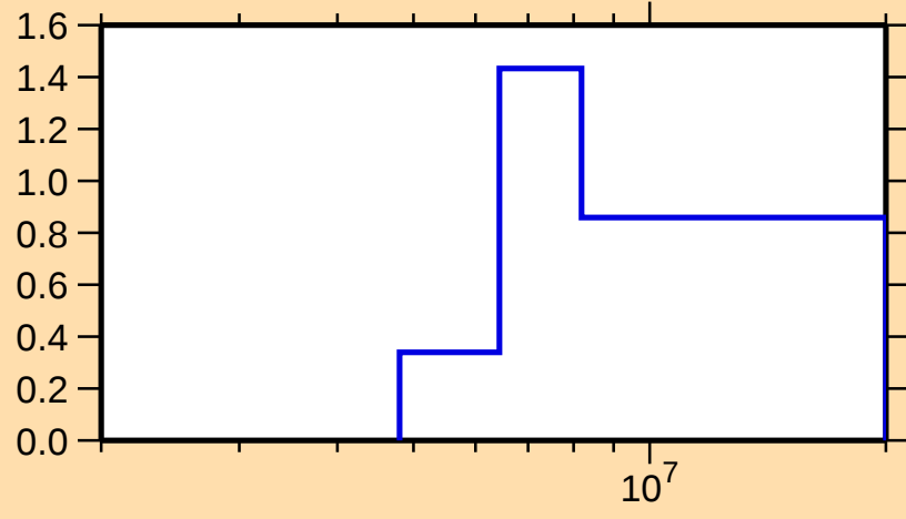
\sigma vs. E for ^{137}\text{I}(n,2n)
