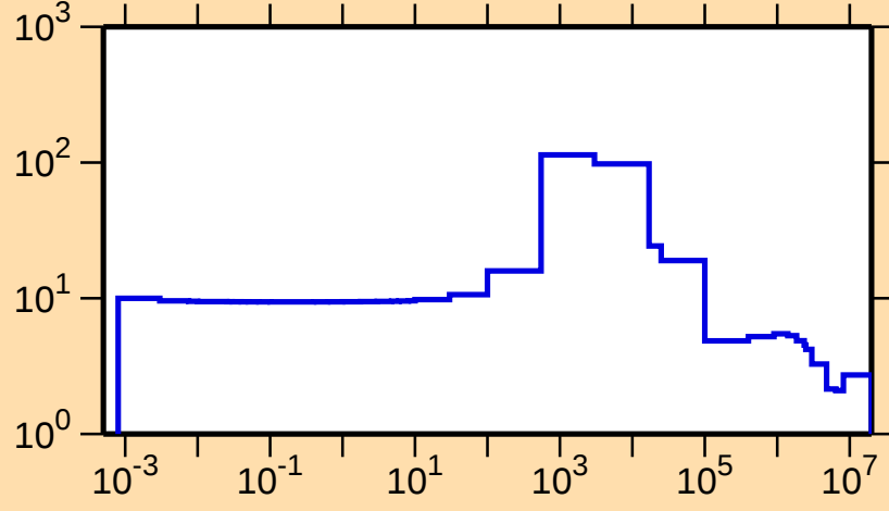
\sigma vs. E for ^{137}\text{I}(\text{n,el.})
