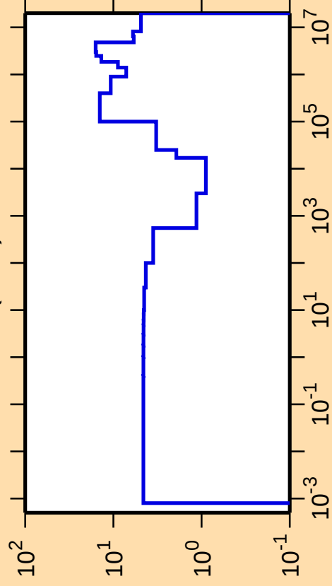
\Delta\sigma/\sigma vs. E for ^{137}\text{I}(\text{n,el.})
