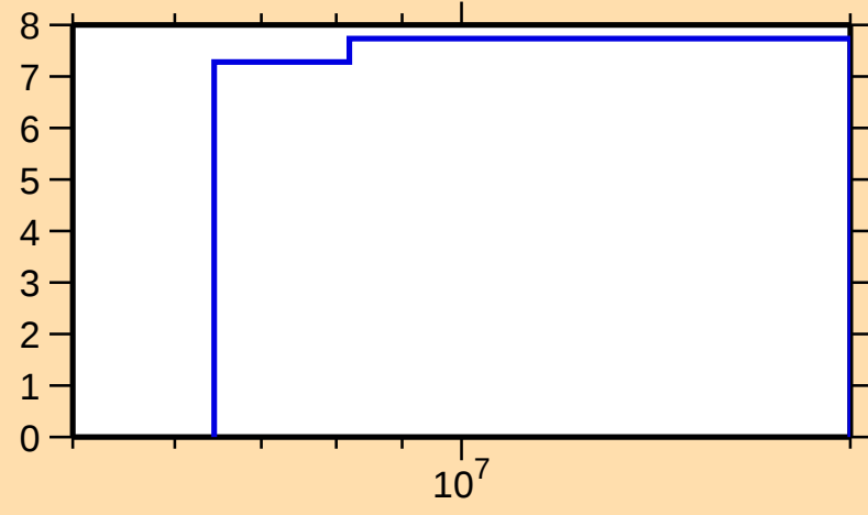
\Delta\sigma/\sigma vs. E for ^{137}\text{I}(n,\text{nonel.})
