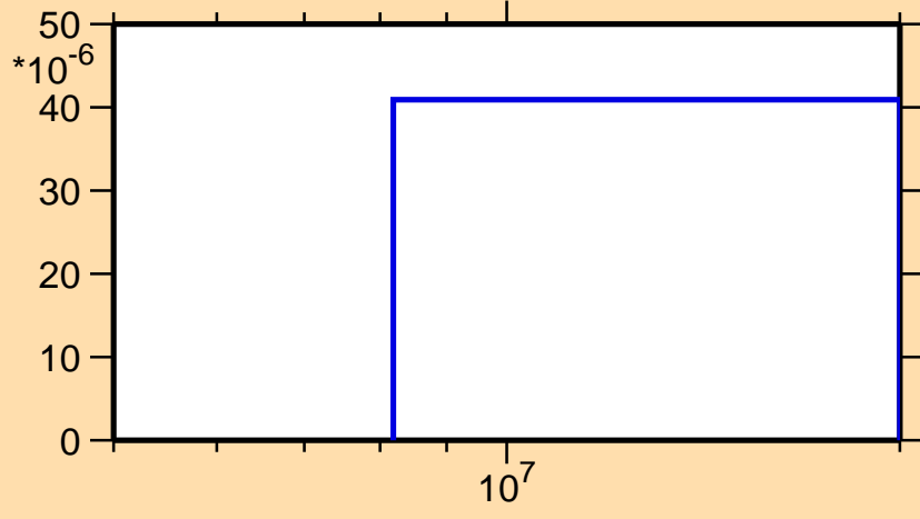
\sigma vs. E for ^{104}\text{In}(n,\text{pd})
