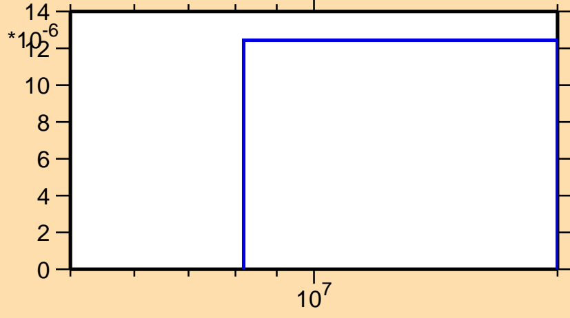
\sigma vs. E for ^{104}\text{In}(n,nd)
