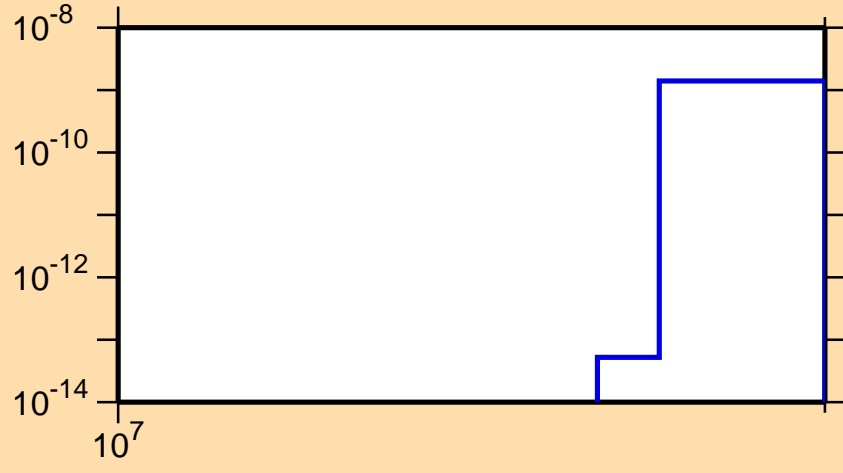
\sigma vs. E for ^{107}\text{In}(n,\text{pt})
