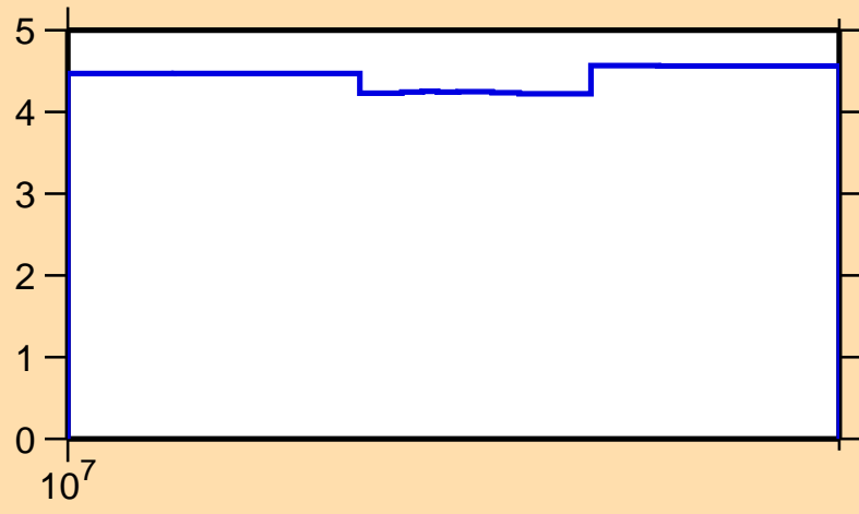
\Delta\sigma/\sigma vs. E for ^{107}\text{In}(n,\text{nonel.})
