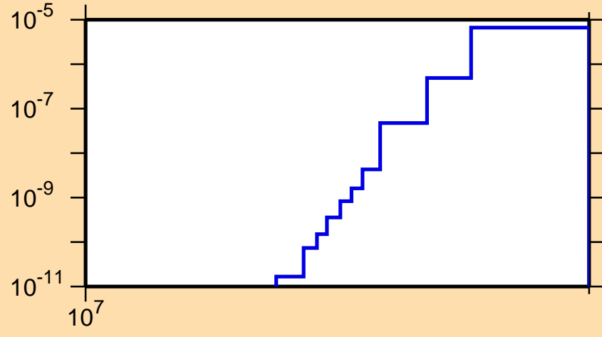
\sigma vs. E for ^{107}\text{In}(\text{mt } 45)
