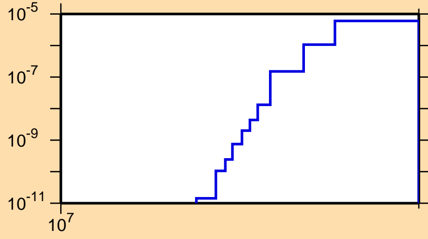
\sigma vs. E for ^{107}\text{In}(n,\text{pd})
