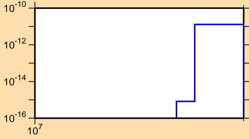
\sigma vs. E for ^{107}\text{In} (mt 34)
