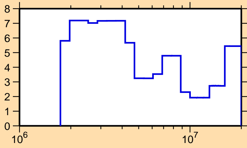
\Delta\sigma/\sigma vs. E for ^{107}\text{In}(n,\text{el.})
