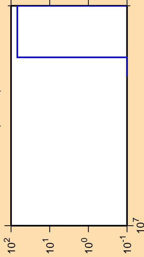
\Delta\sigma/\sigma vs. E for ^{107}\text{In} (mt 34)
