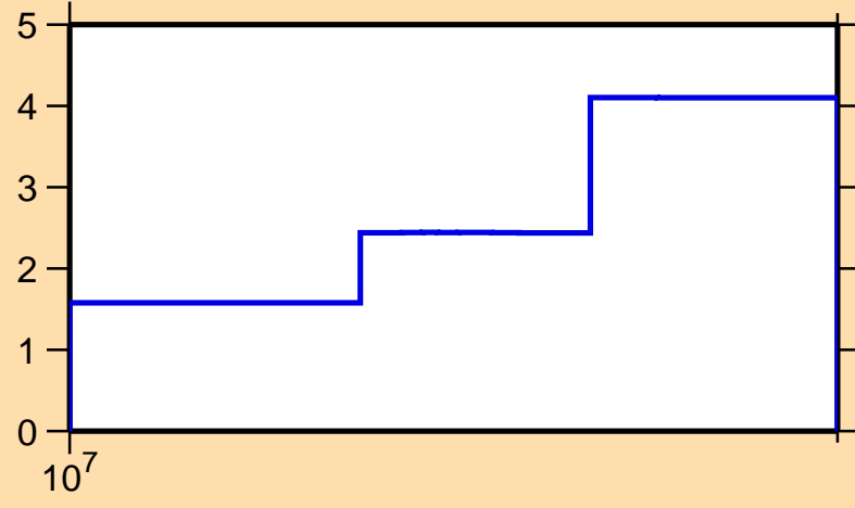
\Delta\sigma/\sigma vs. E for ^{107}\text{In}(n,\text{tot.})
