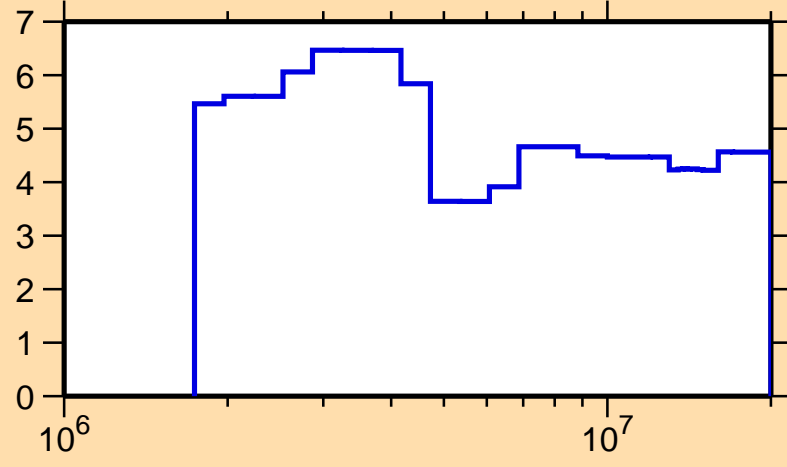
\Delta\sigma/\sigma vs. E for ^{107}\text{In}(n, n_{\text{nonel}})
