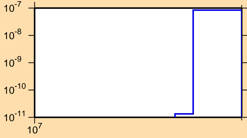
\sigma vs. E for ^{107}\text{In}(n,nt)
