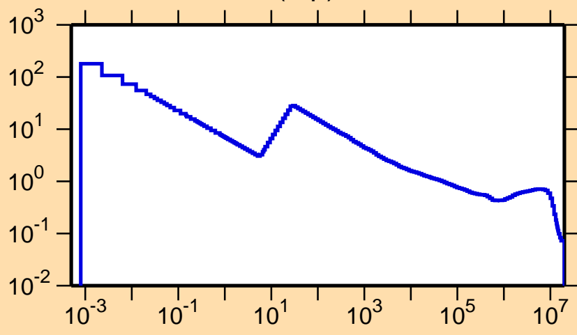
\sigma vs. E for ^{107}\text{In}(n,p)
