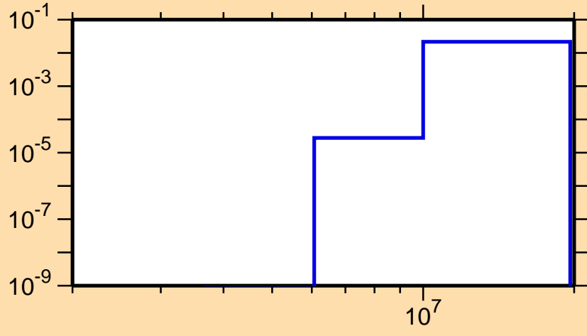
\sigma vs. E for ^{107}\text{In}(n,n\alpha)
