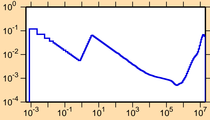
\sigma vs. E for ^{108}\text{In}(n,\alpha)
