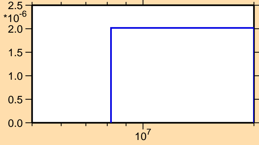
\sigma vs. E for ^{108}\text{In}(n,\text{He}3)
