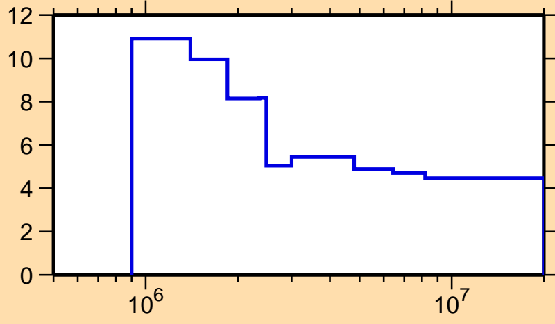
\Delta\sigma/\sigma vs. E for ^{108}\text{In}(n, n_{\text{nonel}})
