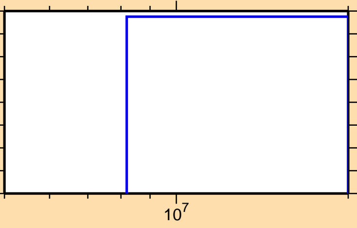
\sigma vs. E for ^{108}\text{In}(n,nd)
