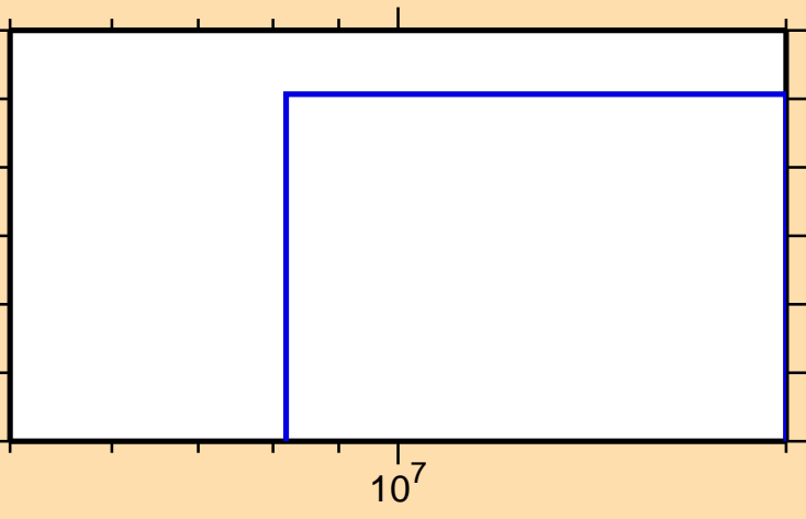
\sigma vs. E for ^{108}\text{In}(n,2np)
