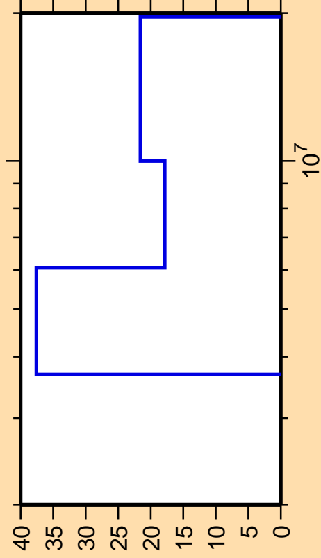
\Delta\sigma/\sigma vs. E for ^{109}\text{In}(n,np)
