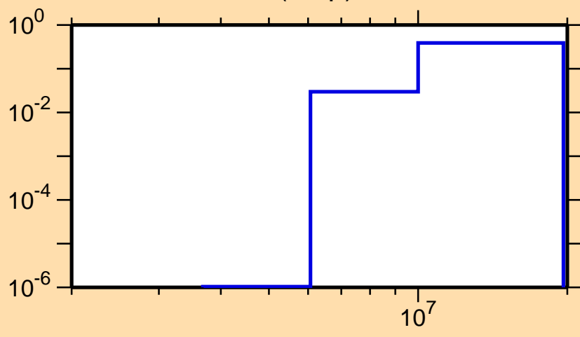
\sigma vs. E for ^{109}\text{In}(n,np)
