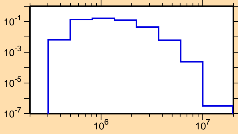
\sigma vs. E for ^{109}\text{In}(n,n_4)
