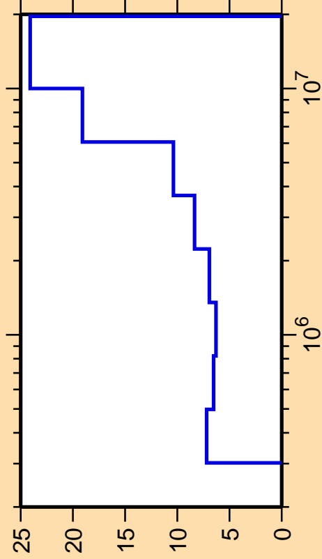
\Delta\sigma/\sigma vs. E for ^{109}\text{In}(n,n_4)
