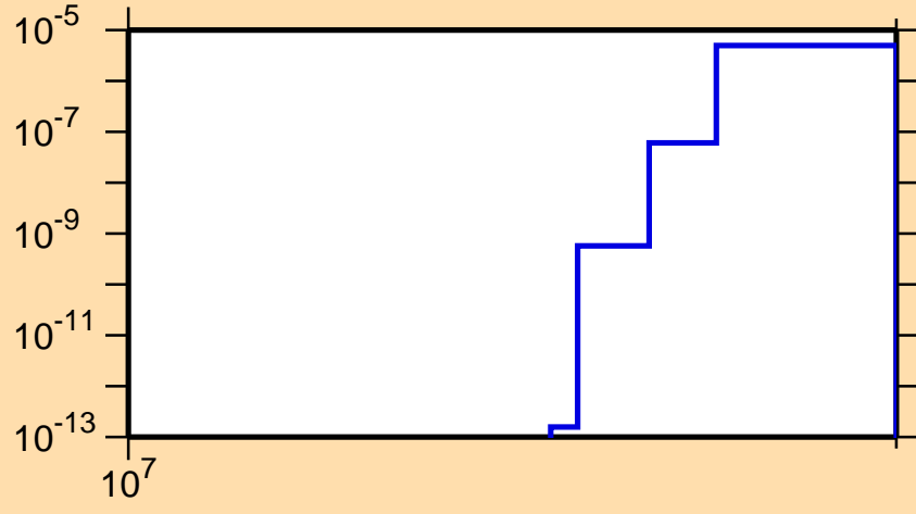
\sigma vs. E for ^{113}\text{In}(n,nd)
