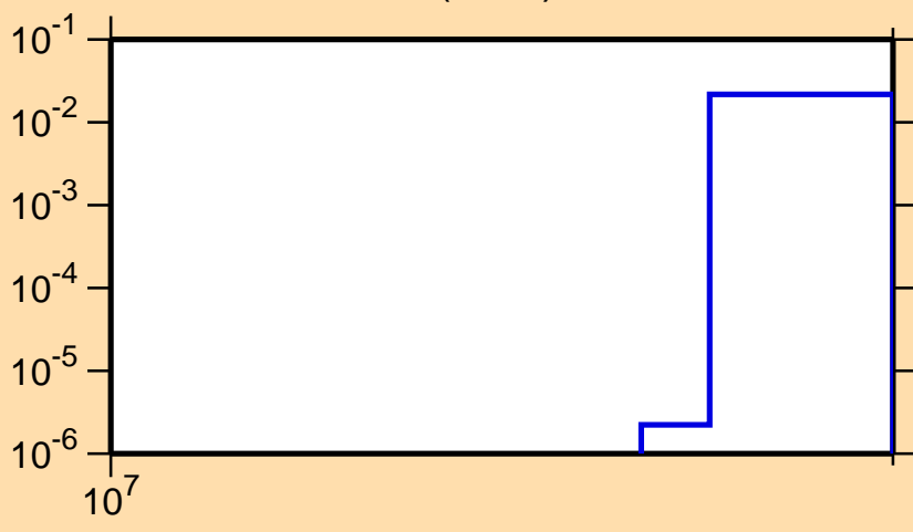
\sigma vs. E for ^{113}\text{In}(n,3n)
