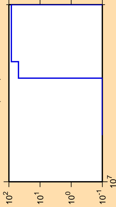
\Delta\sigma/\sigma vs. E for ^{113}\text{In}(n,nd)
