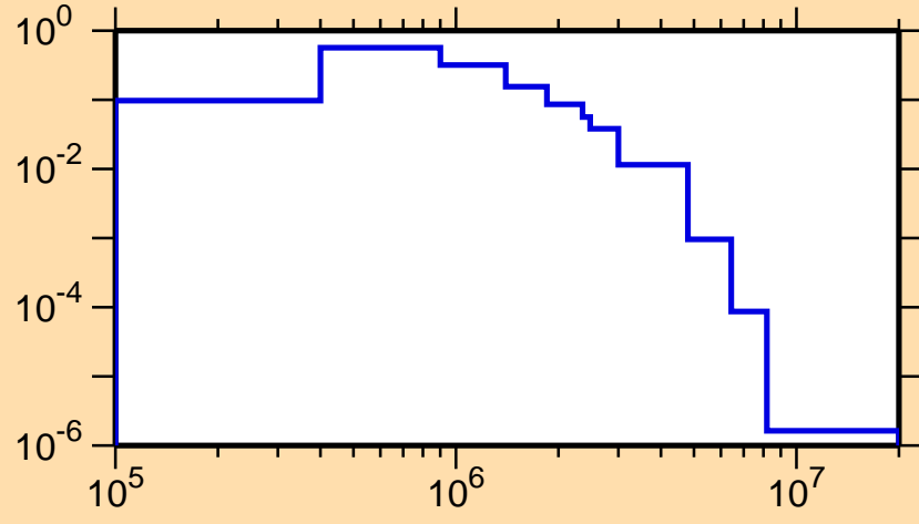
\sigma vs. E for ^{113}\text{In}(n,n_2)
