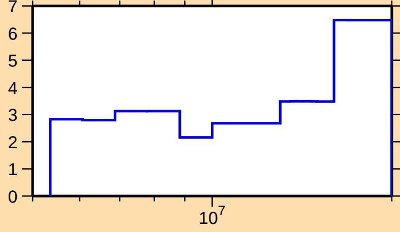
\Delta\sigma/\sigma vs. E for ^{120}\text{In}(n,\text{tot.})
