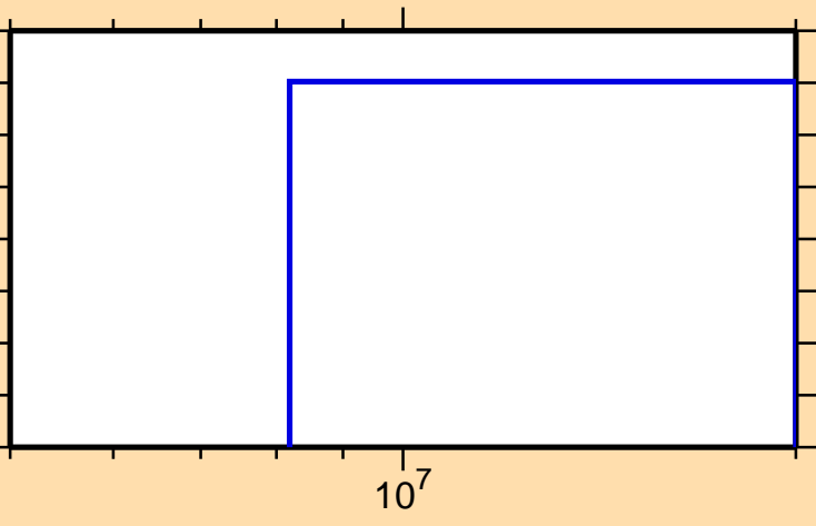
\sigma vs. E for ^{120}\text{In}(n,3n)
