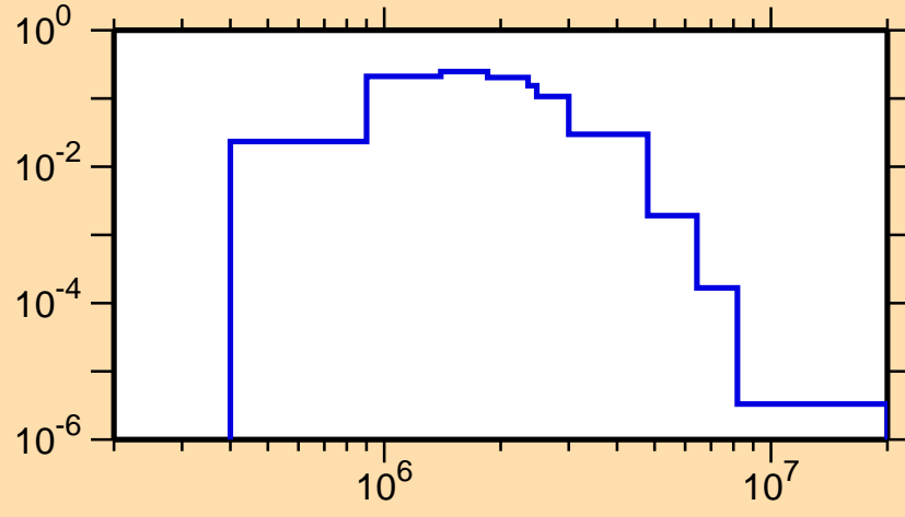
\sigma vs. E for ^{123}\text{In}(n,n_4)
