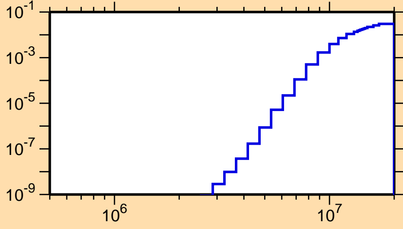
\sigma vs. E for ^{172}\text{Ir}(n,d)
